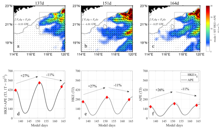
170 Figure 3. (a-c) Spatial distribution of mode-1 SIT energy on days 137, 151, and 164. Black arrows represent energy flux of SIT, and grey 175 contours represent the depth of 250 m. (d-f) Time series of TE, HKE, and APE obtained from area integral over the region R2, with the red diamonds corresponding to days 137, 151, and 164, respectively. The grey curve in (f) is calculated using Eq. (2).
