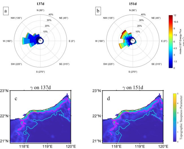
Figure 16. (a-b) The rose diagrams for the mode-2 SIT on days 137 and 151, respectively, the selected region is (119-120° E, 19.9-22.3° N). (c-d) The topographic steepness parameter for days 137 and 151, respectively, magenta line for \gamma=1 and cyan line for the 2000 m isobath.
