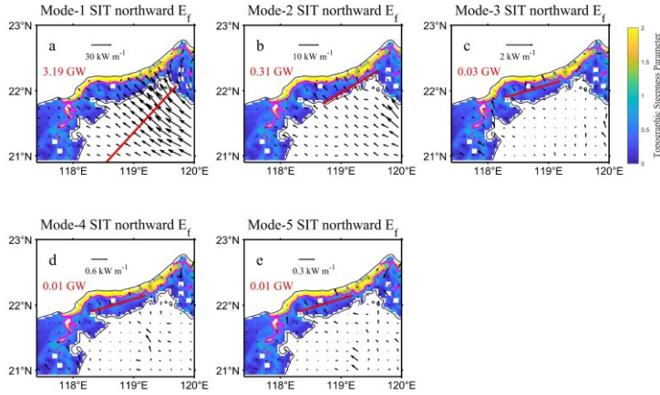
280 Figure 9. Same as Fig. 8, but for day 137.
