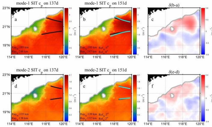
Figure 17. Spatial distributions of phase speeds (only considering the stratification) of mode-1 and mode-2 SITs on days 137 and 151. (c) and (f) represent the differences between days 151 and 137. The black and cyan curves are the propagation rays of SITs during days 137 and 151, respectively.
