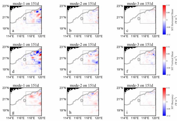
320 Figure 12. Spatial distributions of the first three modes of SITs on day 151, with (a-c) representing horizontal shear production, (d-f) representing vertical shear production, and (g-i) representing horizontal buoyancy production.
