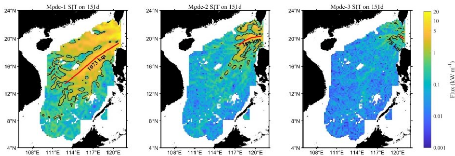
Figure 2. Spatial distribution of energy flux for the first three modes of SITs on day 151 in the SCS (in log scale), the red curves are the main propagation path of the first three modes of SITs , the black values indicate the propagation distance of the red curves.
