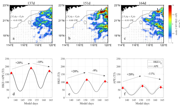
Figure 4. Same as Fig. 3, but for mode-2 SIT.
