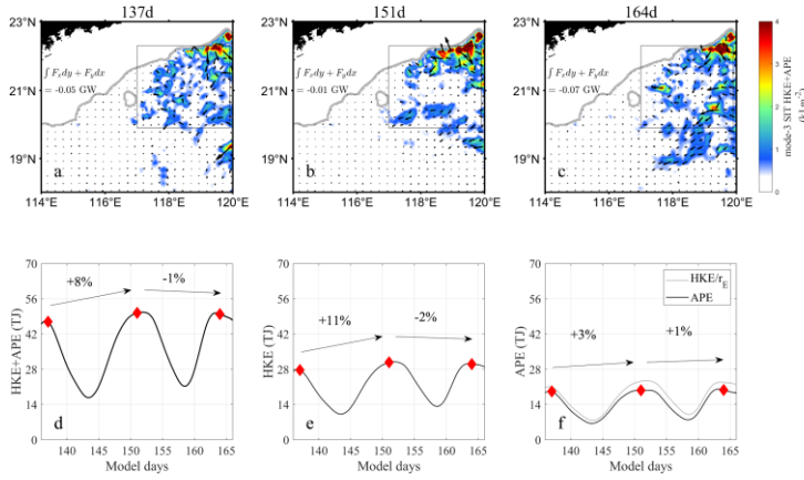
Figure 5. Same as Fig.3, but for mode-3 SIT.
