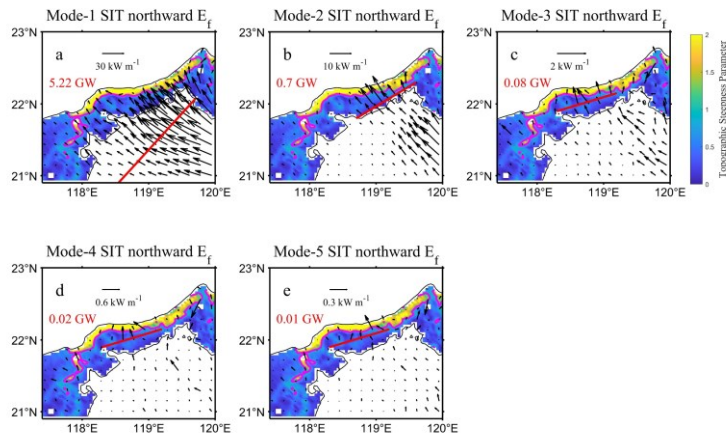
275 Figure 8. Spatial distribution of the northward component (incident wave) of the energy flux (arrows) for the first five modes of SITs on day 151, superimposed on the contour map of topographic steepness parameters from 250 to 2000 m, with magenta contour for \gamma = 1 . The red values in the upper left are calculated by integrating energy flux along the section (red line).
