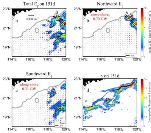
Figure 14. The energy flux of mode-2 SIT on day 151 in (a), (b), and (c) for total, northward, and southward, respectively. The energy fluxes integrated along sections S1 and S2 are labelled as onshore cross-shore and offshore along-shore values, respectively. The topographic steepness parameter for SIT on day 151 is presented in (d).
