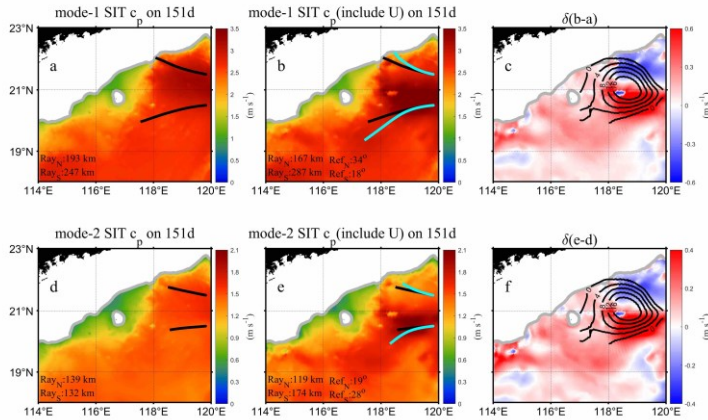
Figure 18. Spatial distributions of mode-1 and mode-2 SIT phase speeds on day 151. (a) and (d) are the same as Fig. 17b and Fig. 17e for c_p without the effect of the background flow; (b) and (e) are c_p^U considering the effect of the background flow; (c) and (f) indicate the difference between the first two modes c_p^U and c_p ; and black contours represent SLA on day 151.
