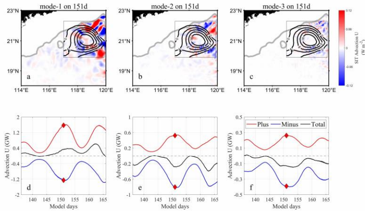
295 Figure 10. Same as Fig. 6, but for the velocity component of the advection term of SIT. The red, blue, and black curves in (d-f) represent the R2 area integral results of positive, negative, and all values within the rectangle, respectively.
