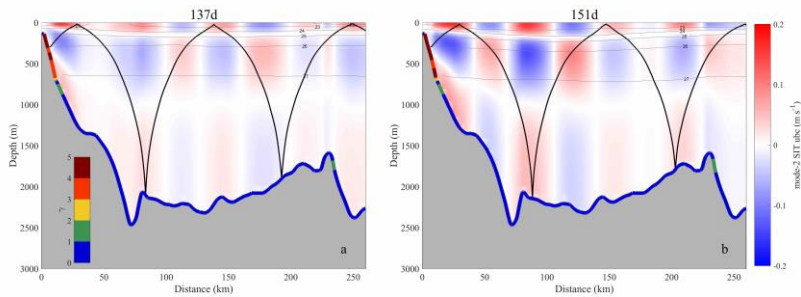
375 Figure 15. The baroclinic velocity of mode-2 SIT on days (a) 137 and (b) 151 along the Beam section shown in Fig. 14c. Black curves are theoretical wave rays, and grey contours are isopycnals ( \sigma -1000). The colors marked along the seafloor represent the values of the topographic steepness parameter.
