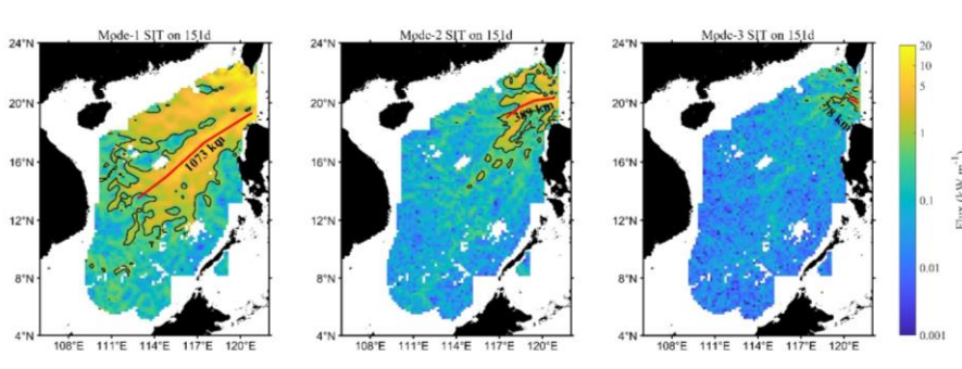
135 Figure 2. Spatial distribution of energy flux for the first three modes of SITs on day 151 in the SCS (in log scale), the black values indicate the length of the red curves.
