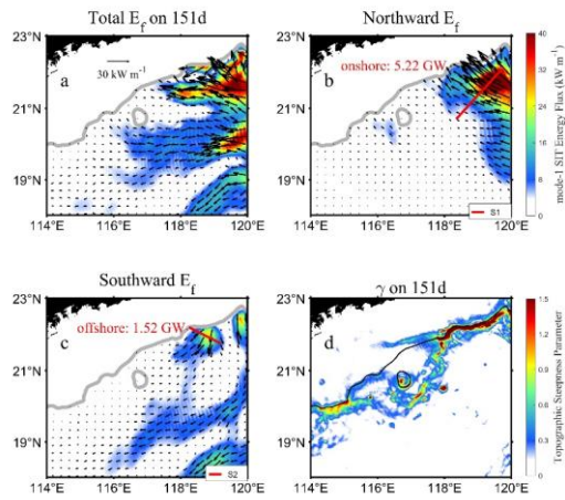
Figure C1. The energy flux of mode-1 SIT on day 151 in (a), (b), and (c) for total, northward, and southward, respectively. The energy fluxes integrated along sections S1 and S2 are labelled as onshore and offshore values, respectively. The topographic steepness parameter for SIT on day 151 is presented in (d).
