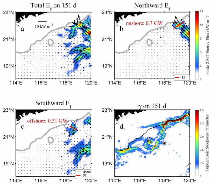
360 Figure 14. The energy flux of mode-2 SIT on day 151 in (a), (b), and (c) for total, northward, and southward, respectively. The energy fluxes integrated along sections S1 and S2 are labelled as onshore and offshore values, respectively. The topographic steepness parameter for SIT on day 151 is presented in (d).
