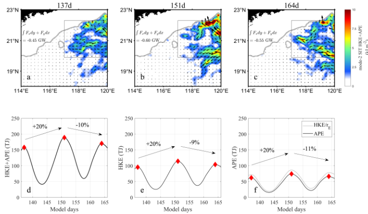
Figure 4. Same as Fig. 3, but for mode-2 SIT.
