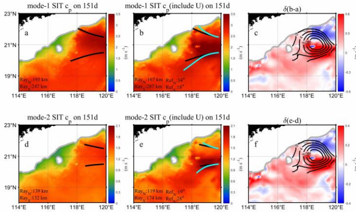
450 Figure 18. Spatial distributions of mode-1 and mode-2 SIT phase speeds on day 151. (a) and (d) are the same as Fig. 17b and Fig. 17e for c_p without the effect of the background flow; (b) and (e) are c_p^U considering the effect of the background flow; (c) and (f) indicate the difference between the first two modes c_p^U and c_p ; and black contours represent SLA on day 151.
