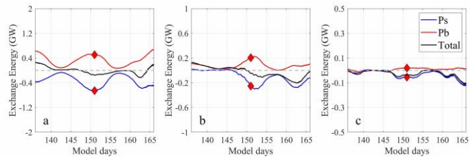
320 Figure 13. Time series of spatial integration for the first three modes (a-c), with Ps representing the sum of the horizontal and vertical shear production terms, Pb representing the horizontal buoyancy production, and Total being their sum.
