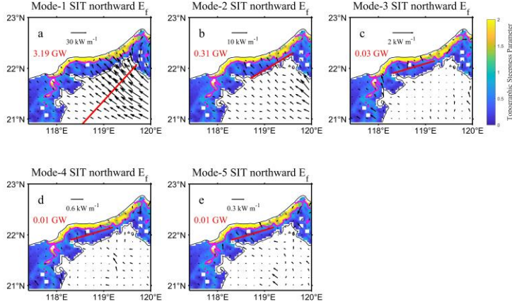
Figure 9. Same as Fig. 8, but for day 137.
