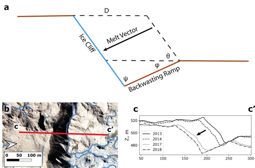
Figure 2. (a) Conceptual model for the geometry of ice cliff backwashing. The melt vector is orthogonal to the exposed ice surface (angle \theta from the horizontal), thus there is a component of vertical incision in addition to horizontal backwashing. The ice cliff as it backwastes produces a ramp of angle \psi to itself and \phi to the horizontal. The value of the angle \psi indicates the efficiency of incision. (b) Map illustrating the location of profile c-c' over a large ice cliff associated with a supraglacial stream (mapped as blue lines). (c) Topographic profiles extracted from ArcticDEM illustrating the backwashing of the ice cliff and the carving out of the backwashing ramp. This ice cliff has an angle between cliff and ramp of \psi = 110^\circ . This ice cliff is in the glacier's stagnant terminus region where the surface velocity is negligible (values of <10 \text{ m yr}^{-1} comparable to values determined outside the glacier outline) and thus did not need to be deconvolved from the signal of surface change.
