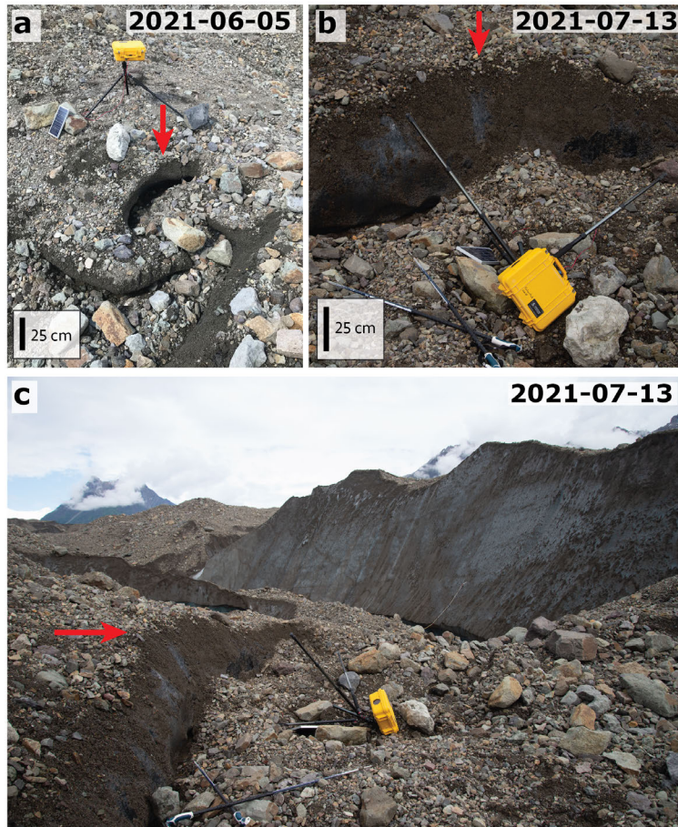
Figure 10. Field evidence for the role of hydrology in generating ice cliffs. (a) Time lapse camera observed on June 5, 2021. Red arrow indicates the crest of a short ( \sim 10\text{-}20 cm tall) ice exposure associated with the incision of minor supraglacial drainage within the debris layer. The natural meander in drainage is expressed in the shape of the ice exposure. (b-c) By July 13, 2021, the ice exposure had grown substantially into a small ice cliff \sim 1 m tall and several meters wide, backwasting through the topography and knocking over the time lapse camera. This also illustrates the need for careful evaluation of local terrain features when placing instruments on the surface of debris-covered glaciers.
