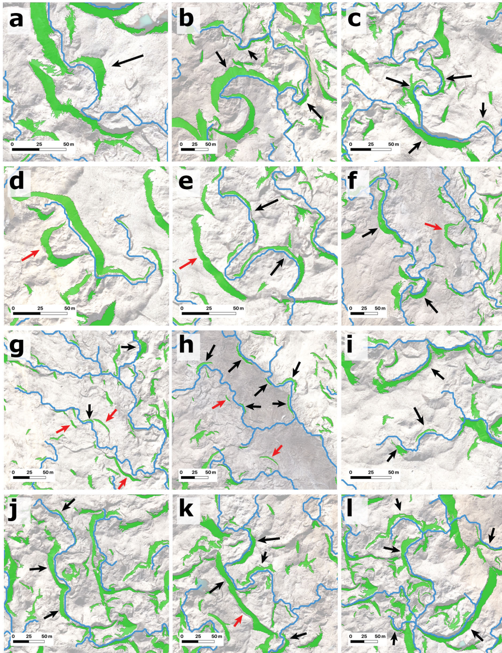
Figure 4. Examples of spatial relationships between identified ice cliffs (green) and stream channels (blue) mapped over a low-opacity orthophoto ( NPS photogrammetry dataset, Section 3.1 ). Black arrows indicate curving ice cliff morphologies observed on the outside bend of supraglacial stream meanders; red arrows indicate similar ice cliff morphologies which appear to have been abandoned by stream channels.
