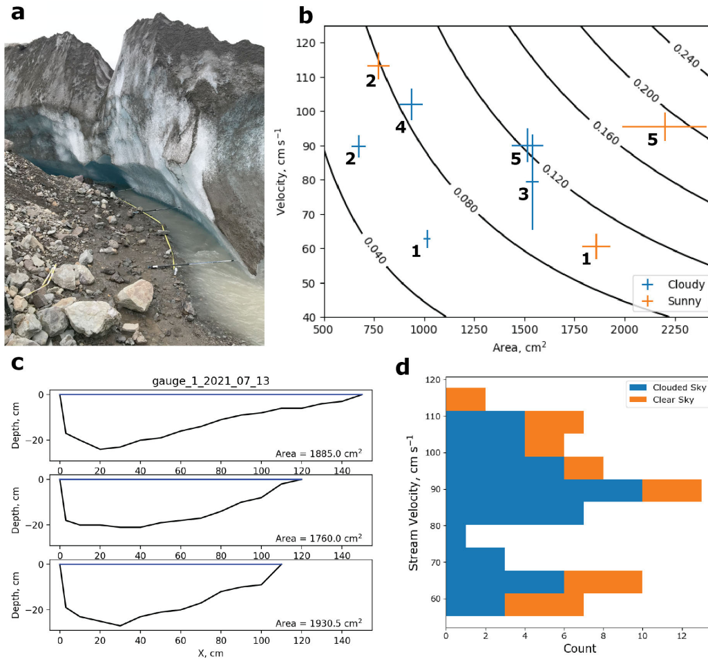
Figure 7. Results of stream discharge measurements. (a) Image of typical setup of discharge measurement including hiking poles ( ~1.4 m length ) marking the flux gates and tape measure. (b) Measured velocity and cross-sectional area for all discharge measurements; plotted contours are the resultant discharge in m 3 s -1 . Data points are distinguished by measurement site (numerical labeling) and sunny/cloudy conditions (color). (c) Example of channel cross-sectional area measurements, from site 1 on July 13, 2021. (d) Histogram of measured velocity values from all 64 datapoints from 8 measurement sets.
