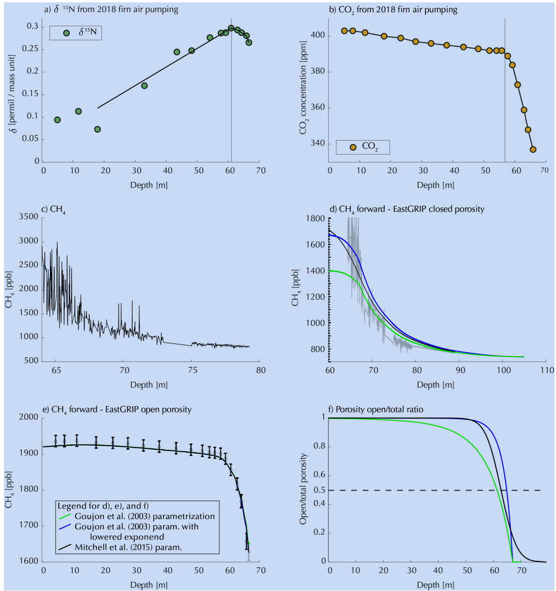
Figure 2. Measurements from the firn air pumping campaign on the S6 borehole, indicating the transition of the diffusive to non-diffusive zone to lie around 61 m for a) \delta^{15}N (not corrected for thermal fractionation) and 58 m depth for b) CO_2 . c) CH_4 measured in the ice core, as a function of depth, around the bubble close-off. d) Forward modeling of CH_4 for closed porosity. e) Laboratory measurements of CH_4 in the air from the open porosity of firn (symbols) compared with IGE-GIPSA firn model results obtained with the two open/closed porosity ratio parameterizations shown in d) (the two model results are nearly superimposed). f) Open/closed porosity ratio parameterizations used in the IGE-GIPSA firn model, blue: usual parameterization using Equation (6) in Witrant et al. (2012), green: the exponential factor is reduced from 7.6 to 3.0.
