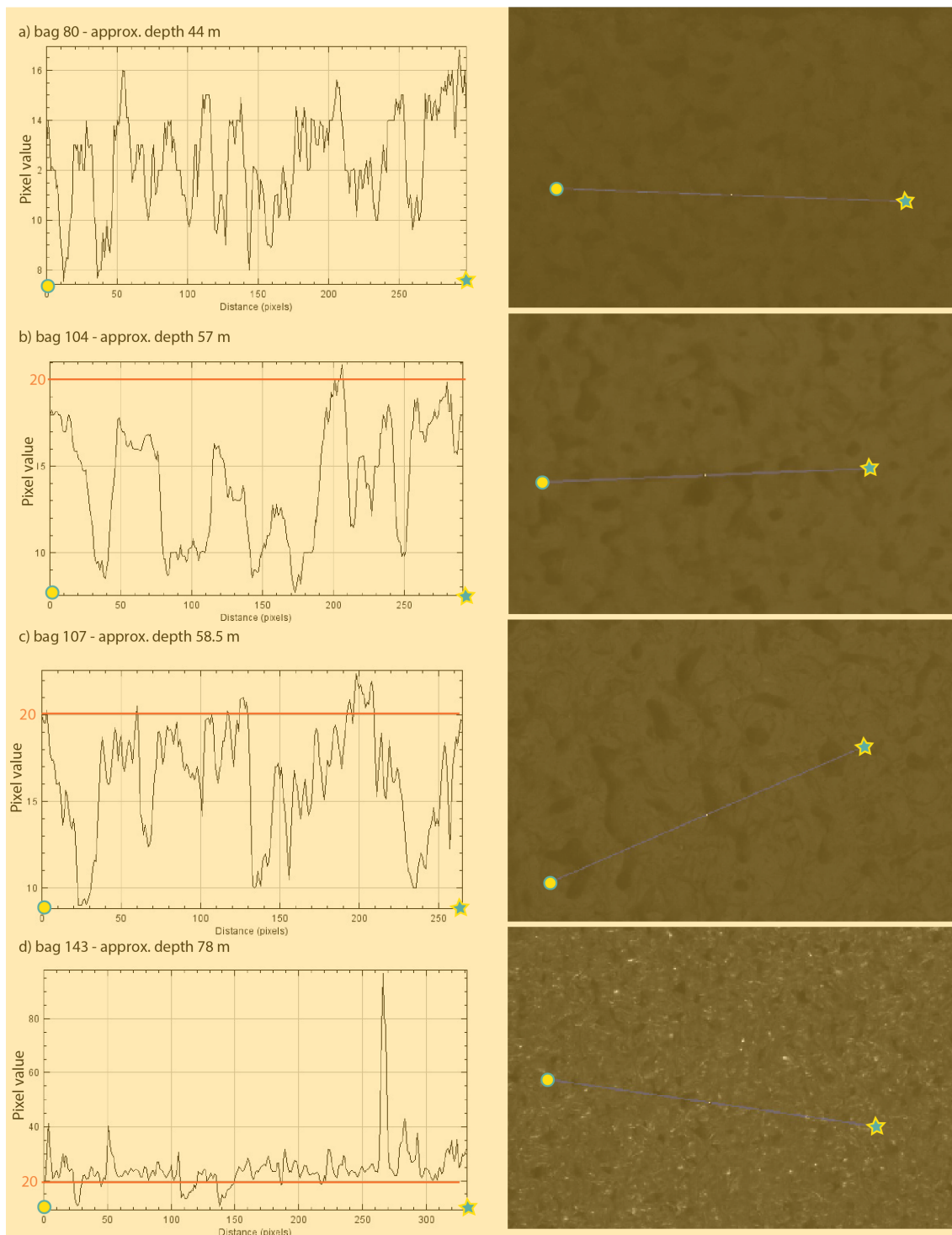
Figure B1. The change of brightness appearance with depth. a) above the firm-ice transition, b-c) the transition, and d) below the firm-ice transition. The left side shows the brightness profiles from the blue lines on the right side. Image width is approximately 2 cm.
