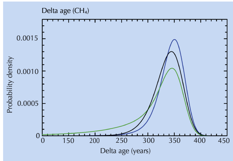
Figure 8. Delta age distributions using different parametrizations (see fig. 2). The different parametrizations discussed throughout this manuscript all result in a delta age of around 350 years.
