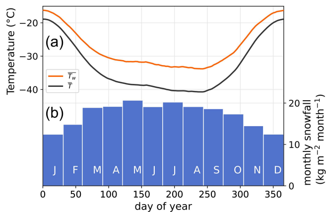
Figure 3. Seasonal cycles of temperature and snowfall averaged over Antarctica. (a) climate normals of temperature ( \bar{T} ) and snowfall-weighted temperature ( \bar{T}_w ). (b) monthly snowfall. For both panels we included all model points on the Antarctic continent, including ice shelves. Climate normal temperatures were computed as arithmetic (for \bar{T} ) or snowfall-weighted (for \bar{T}_w ) average of the same day of year for all the 1979–2020 period, then smoothed with a 30-days rolling mean (see Sect. 2 Methods).
