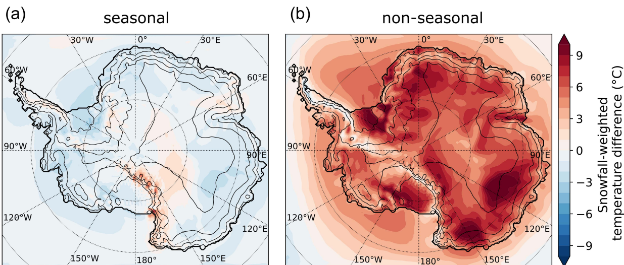
430 Figure 5. Seasonal and non-seasonal effects of snowfall weighting on temperature difference ( \Delta T ). (a) seasonal effect on temperature difference reflects the temperature changes induced by snowfall seasonality. (b) non-seasonal effects of snowfall weighting, revealing the influence of snowfall event-related warming. The sum of both maps results in the map shown in Fig. 2 (see Sect. 2 methods).
