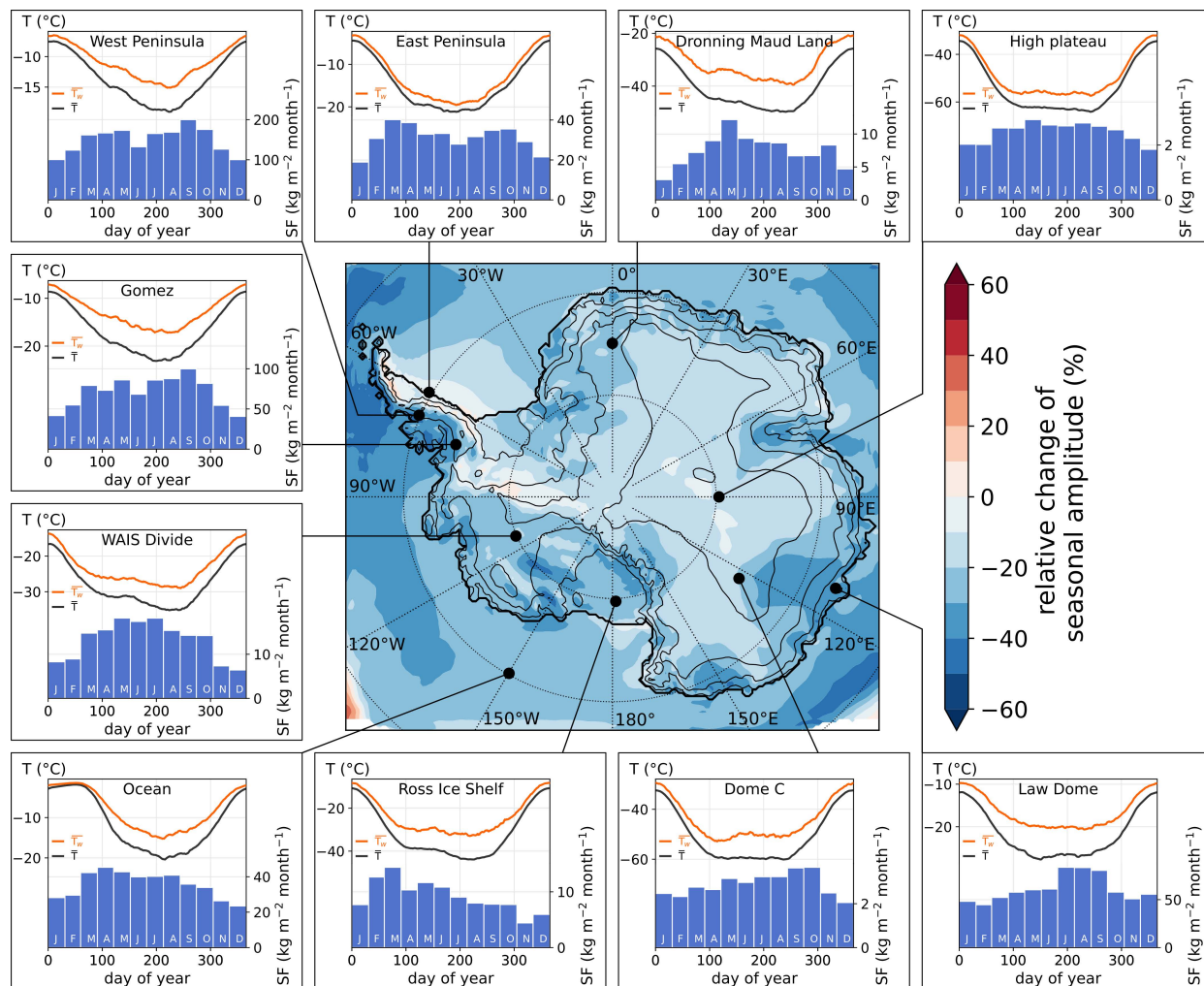
Figure 4. Map of the relative change in seasonal amplitude, defined as the ratio of standard deviations r_{SD} = \left( \frac{SD(\bar{T}_w)}{SD(\bar{T})} - 1 \right) \times 100 for each model cell, where SD is the standard deviation. Inserts show seasonal cycles of temperature and snowfall for a selection of 10 sites in Antarctica. For each site, climate normals of temperature ( \bar{T} ), snowfall-weighted temperature ( \bar{T}_w ) and monthly snowfall, similarly to Fig. 3. Climate normal temperatures were computed as arithmetic (for \bar{T} ) or snowfall-weighted (for \bar{T}_w ) average of the same day of year for all the 1979–2020 period, then smoothed with a 30-days rolling mean.
