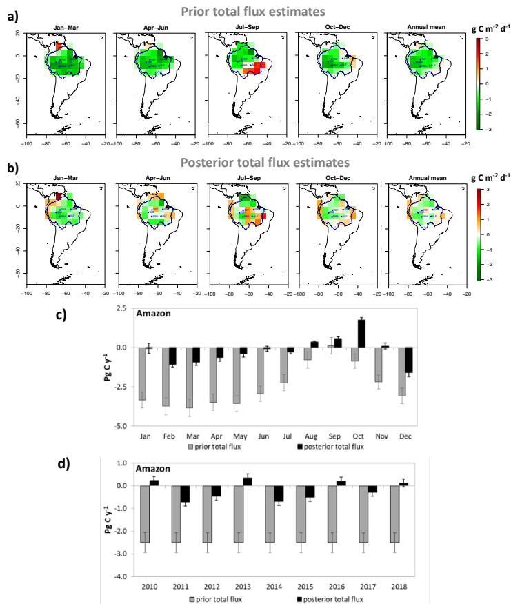
190 Figure A14. Quarterly and annual mean a) prior total (with CARDAMOM as land-biosphere prior flux), 195 b) posterior total (with CARDAMOM as land-biosphere prior flux), carbon fluxes, where a positive value indicates a net emission of C while a negative value indicates a net uptake, c) nine-year monthly mean and d) annual means carbon fluxes for the Amazon using CARDAMOM estimates as land-biosphere prior fluxes between 2010 and 2018. The blue contour represents the Amazon area based on Eva and Huber (2005).
