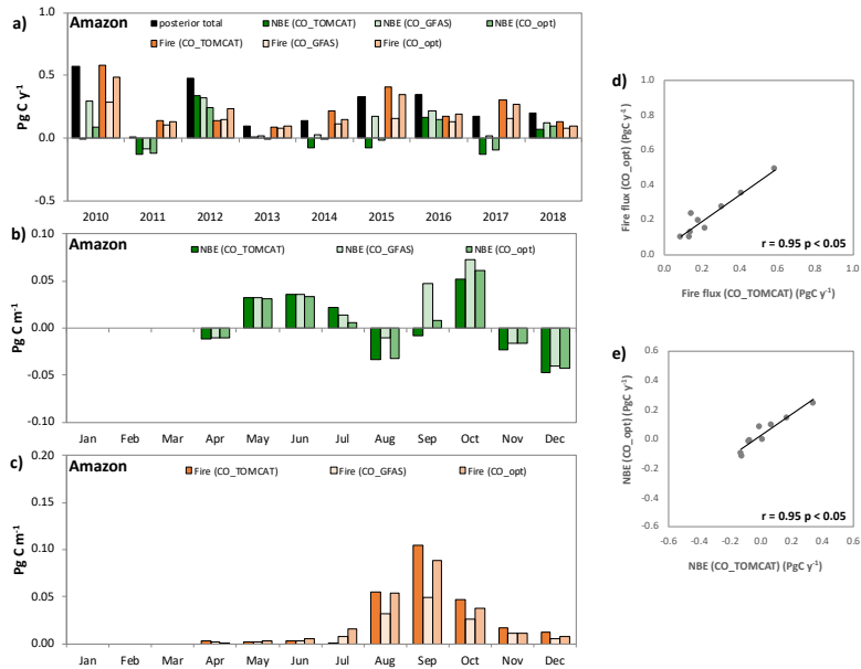
Figure A16. a) Annual mean fluxes for the Amazon region total, fire and NBE estimates. Fire and NBE based on TOMCAT CO inversions (CO_TOMCAT), Naus et al. (2022) emissions using GFAS as a prior (CO_GFAS) and with their CO optimized inversions (CO_opt). Nine-year monthly mean NBE (b) and fire (c) carbon fluxes for the Amazon, Fire and NBE based on TOMCAT CO inversions (CO_TOMCAT), Naus et al. (2022) emissions using GFAS as prior (CO_GFAS) and with their CO optimized inversions (CO_opt). Linear regressions between annual mean carbon fire flux (d) and posterior NBE (e) based on TOMCAT CO inversions (CO_TOMCAT) and Naus et al. (2022) CO optimized inversions (CO_opt)
