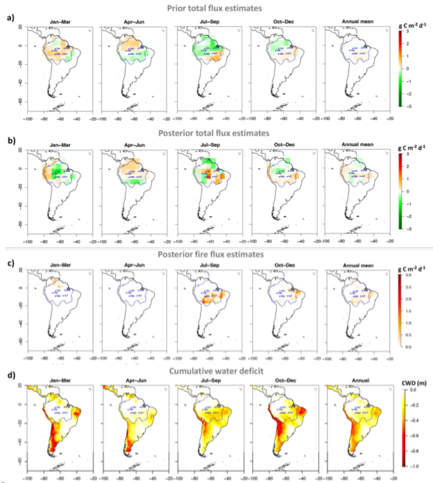
1055 Figure 3: Quarterly and annual mean a) prior total (with CASA as land-biosphere prior flux), b) posterior total, c) posterior fire carbon fluxes, where a positive value indicates a net emission of C while a negative value indicates a net uptake, d) cumulative water deficit (CWD) for the Amazon region between 2010 and 2018. The blue contour represents the Amazon area based on Eva and Huber (2005) .
