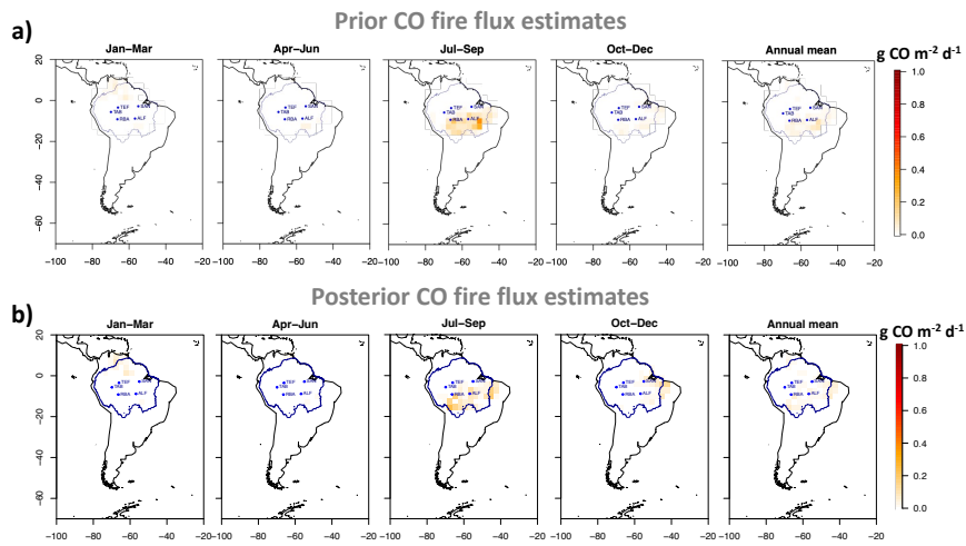
Figure A3. Quarterly and annual mean prior (a) and posterior (b) fire carbon monoxide (CO) fluxes with MOPITT data assimilated for the Amazon region between 2010 and 2018. The blue contour represents the Amazon area based on Eva and Huber (2005).
