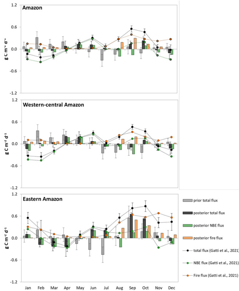
265 Figure A20. Comparison of monthly mean C fluxes from inverse modelling using Amazon vertical profile observations and C fluxes based on the vertical profile observations calculated by mass balance technique from Gatti et al. (2021), for the period between 2010 and 2018.
