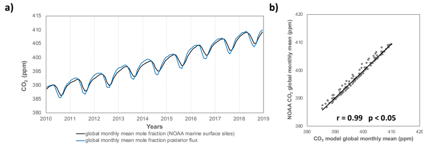
Figure A1. a) Time series of the global monthly mean CO 2 mole fraction from our posteriori fluxes and from the NOAA marine surface sites (Lans, et al., 2023). b) Linear correlation between global monthly mean CO 2 mole fraction from our posteriori fluxes and from the NOAA marine surface sites.
