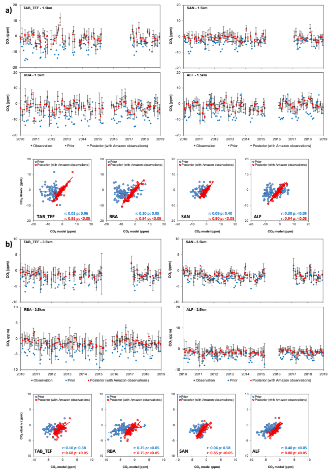
200 Figure A15: Detrended monthly mean CO 2 mole fractions (ppm) for prior (with CARDAMOM as land- biosphere prior flux), posterior and Amazon vertical profiles and its linear regressions, where a) is the mean below 1.5 km altitude (planetary boundary layer levels and b) the mean above 3.5 km altitude (vertical profile free troposphere), for each of the vertical profile sites. The model results were extracted for the grid cell where each site is located. After detrended we subtracted the global mean mole fraction 205 from the observation and model mole fractions. Error bars represent the observation uncertainties.
