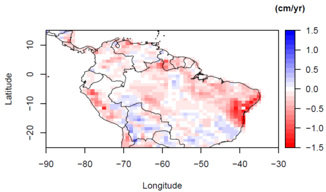
250 Figure A19. Time trend of maximum cumulative water deficit (CWD) between 1998 and 2019 based on TRMM v 7 precipitation estimates (Huffman et al., 2010).
