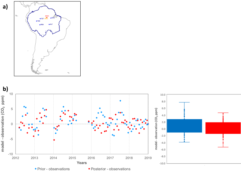
220 Figure A17. A) Locations of INPE/LaGEE Amazon vertical profile sites assimilated in the inversions 225 (blue circles) and the two sites (MAN and ATTO) with data used for cross-validation. The blue contour represents the Amazon area based on Eva and Huber (2005). B) time series and box plot of model bias (model – observations) of monthly mean CO 2 mole fractions (ppm) for the ATTO tower.
