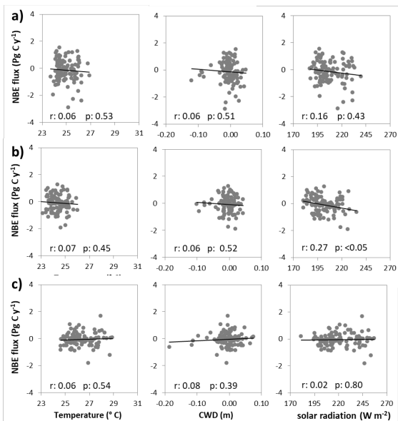
160 Figure A9. a) Linear regressions between monthly mean carbon posterior NBE flux (posterior total flux less posterior fire flux) and temperature, cumulative water deficit (CWD) and solar radiation for a) whole, b) western-central and c) eastern Amazon regions.
