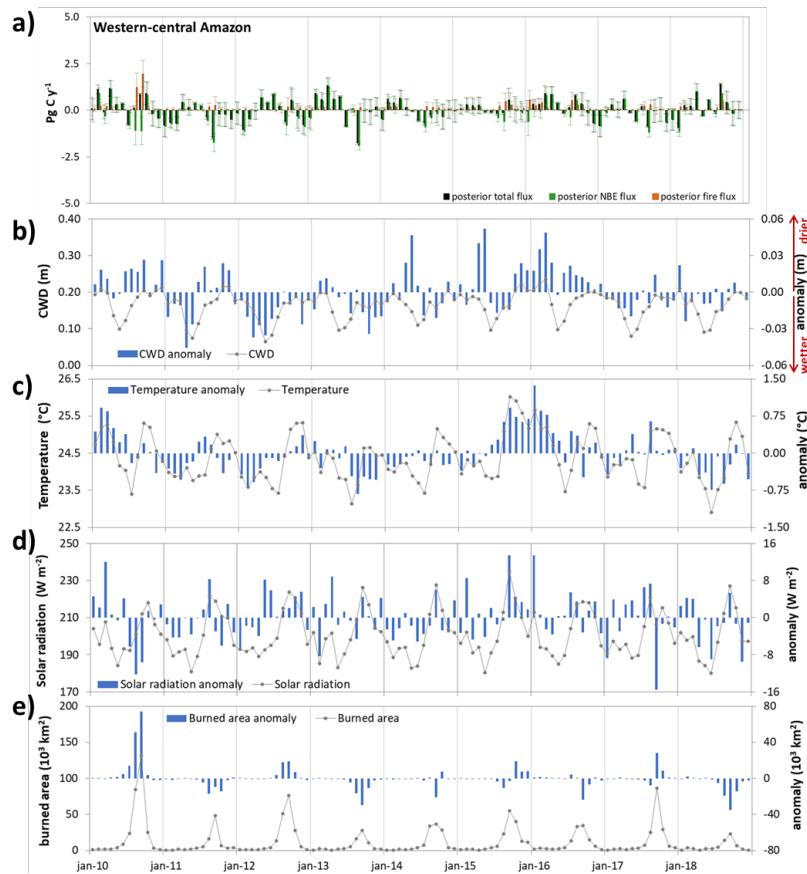
125 Figure A4 a) Monthly mean carbon fluxes for the western-central Amazon area: posterior total flux with the Amazon vertical profile observations in the inversion (black bars), posterior fire fluxes using MOPPIT carbon monoxide observations in the inversion (orange bars) and posterior NBE fluxes which is the result of the subtraction of the posterior fire fluxes from the posterior total fluxes the Amazon vertical profile observations in the inversion (green bars), representing the net biome exchange. Monthly mean and 130 anomalies of b) cumulative water deficit (CWD), c) temperature, d) shortwave flux down solar radiation (all sky) and e) burned area for the western-central Amazon area.
