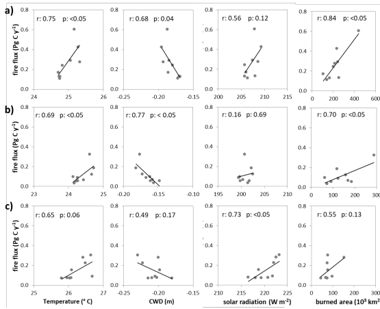
Figure A11. a) Linear regressions between annual mean carbon posterior fire flux (posterior total flux less posterior fire flux) and temperature, cumulative water deficit (CWD), solar radiation and burned area for a) whole, b) western-central and c) eastern Amazon regions.
