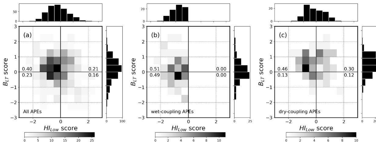
Figure S1: Joint distribution of (a) all APEs, (b) wet-coupling APEs and (c) dry-coupling APEs as functions of B_{LT} score and HI_{Low} score. The number indicates the fraction in each quadrant.
