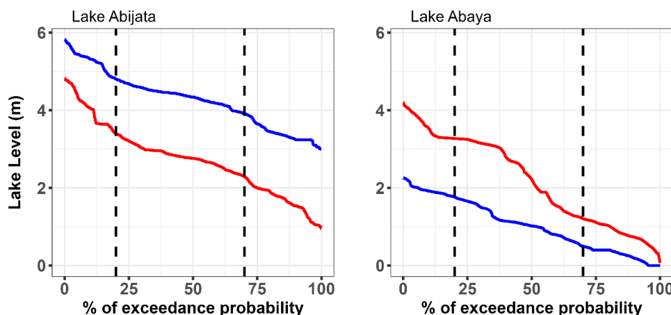
Figure 9 | Monthly median and FDC analysis of pre-impacted and impacted period
