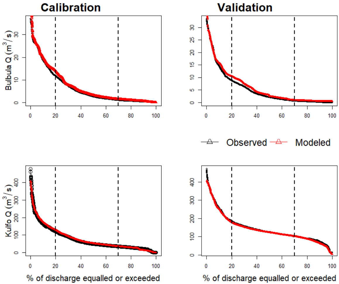
2 Figure 6 | Flow duration curves of observed and modeled daily streamflow for the calibration 3 and validation period of the ‘donor watersheds.
