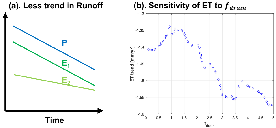
285 Figure 7. (a) Conceptual plot of annual precipitation ( P ) and annual evapotranspiration ( ET ) with different trend ( E_1 and E_2 ). Subplot (b) shows the sensitivity of annual ET trend (e.g., Sen's slope of annual basin averaged ET during the simulation period) to f_{drain} .
