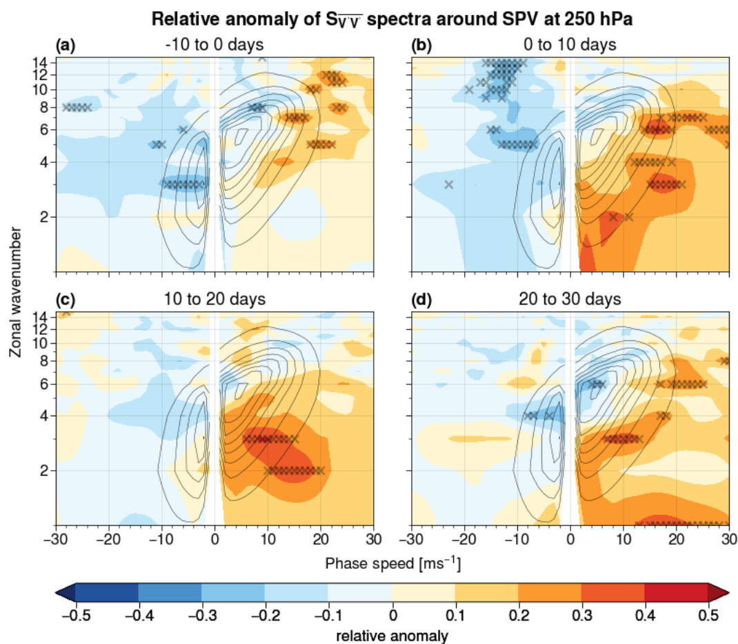
Figure 6. Same as Figure 4, but for SPV events.
