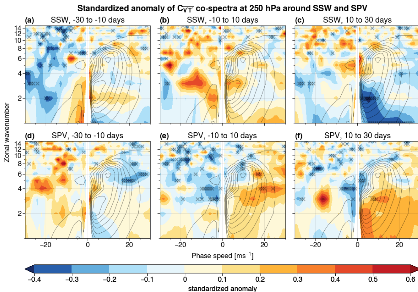
Figure 10. Standardized anomalies of heat flux co-spectra C_{\sqrt{T}} compared to the NDJFM standard deviation at 250 hPa, averaged over 20-day time intervals around 25 SSW events (a to c) and over 31 SPV events (d to f). Wavenumber-phase speed harmonics marked with an \times exceed the 0.5th or 99.5th percentile of the re-sampled distribution. Black contour lines show the NDJFM climatology ranging from -0.006 \text{ K ms}^{-1} \Delta c^{-1} to 0.021 \text{ K ms}^{-1} \Delta c^{-1} in steps of 0.003 \text{ K ms}^{-1} \Delta c^{-1} as in Figure 1c.
