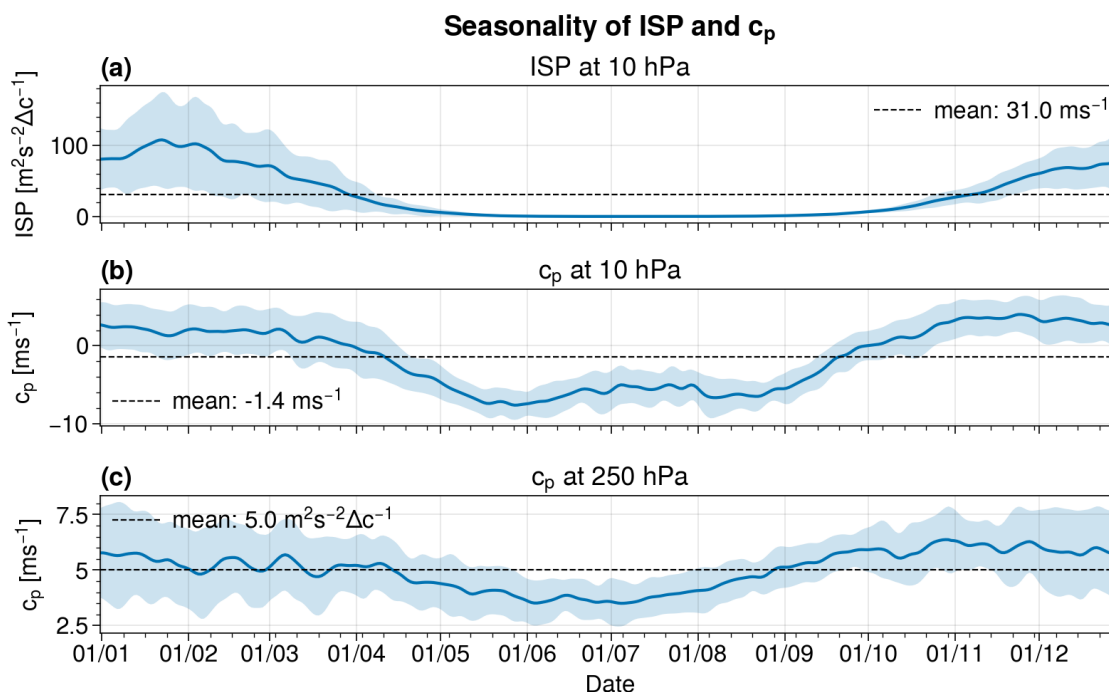
Figure 2. Seasonal cycle of ISP at 10 hPa (a), as well as phase speed at 10 hPa (b) and at 250 hPa (c). Blue lines depict the daily average, and blue shaded areas mark \pm 1 standard deviation around the daily mean. The dashed line shows the mean over the whole time period from 1979 to 2020.
