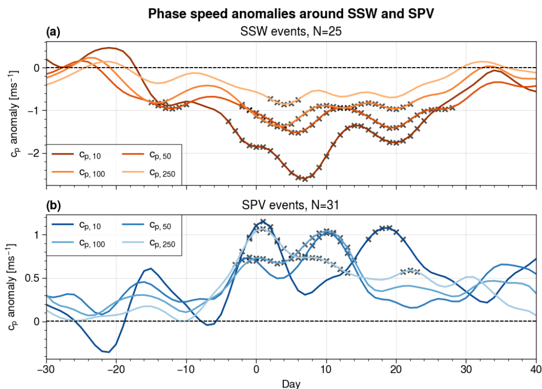
Figure 7. Time series of daily averages around SSW (a) and SPV (b) events for phase speed anomaly with respect to the NDJFM seasonal cycle at each level. Points marked with an \times lie outside of the 99% confidence interval with respect to the seasonal cycle.
