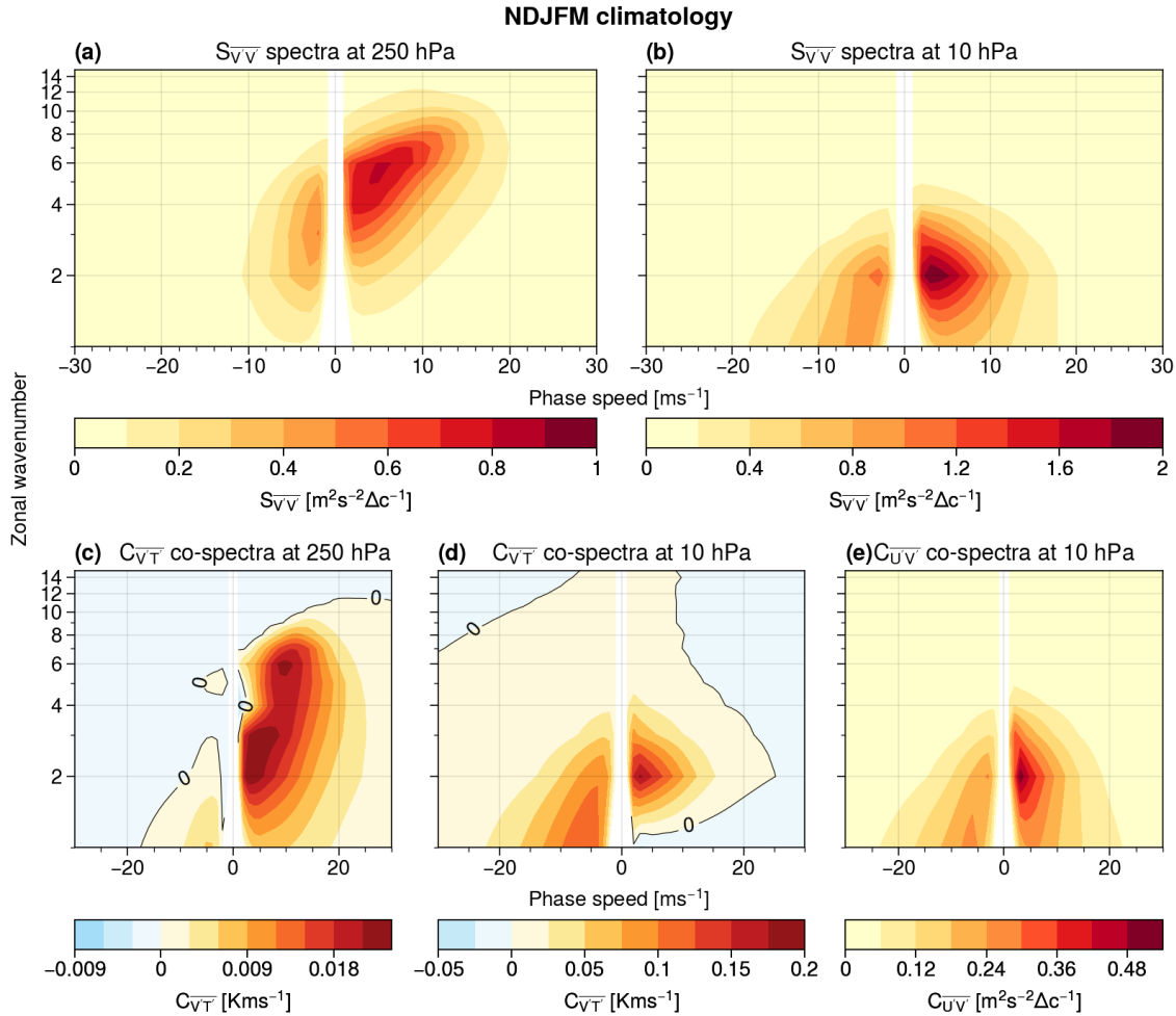
Figure 1. Seasonal mean spectral power S_{\overline{V\overline{V}'}} of meridional wind V at 250 hPa (a) and 10 hPa (b) for NDJFM, as well as for heat flux co-spectra C_{\overline{V\overline{T}'}} at 250 hPa (c) and 10 hPa (d) and momentum flux co-spectra C_{\overline{U\overline{V}'}} at 10 hPa (e). Note the different color scale between the different panels, and that values are multiplied by n to compensate for the non-constant density of points (due to the logarithmic scale used for the y-axis).
