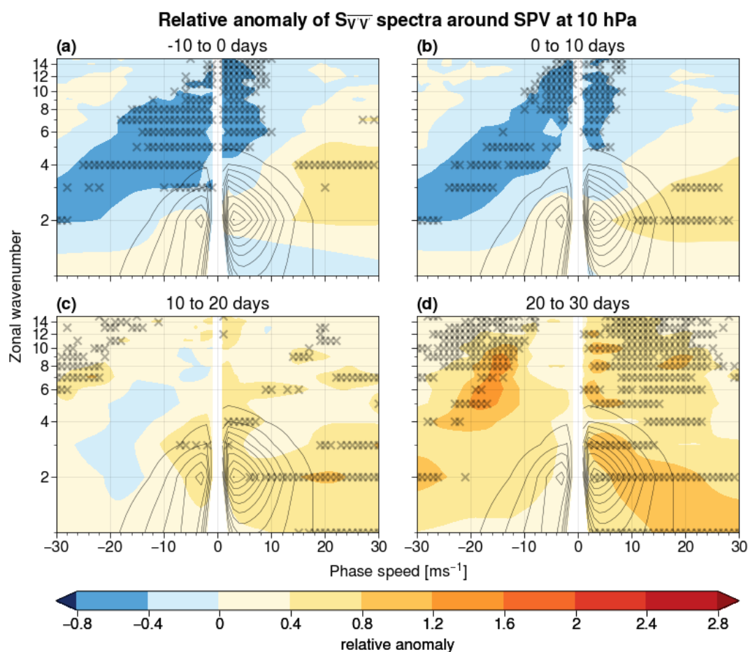
Figure 5. Same as Figure 3, but for SPV events.
