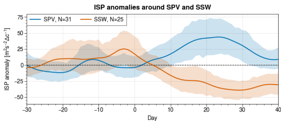
Figure 8. Time series of daily averages around SSW (orange) and SPV (blue) events for ISP anomaly with respect to the NDJFM seasonal cycle at 10 hPa. Shaded areas depict the 99% confidence interval with respect to the daily mean.
