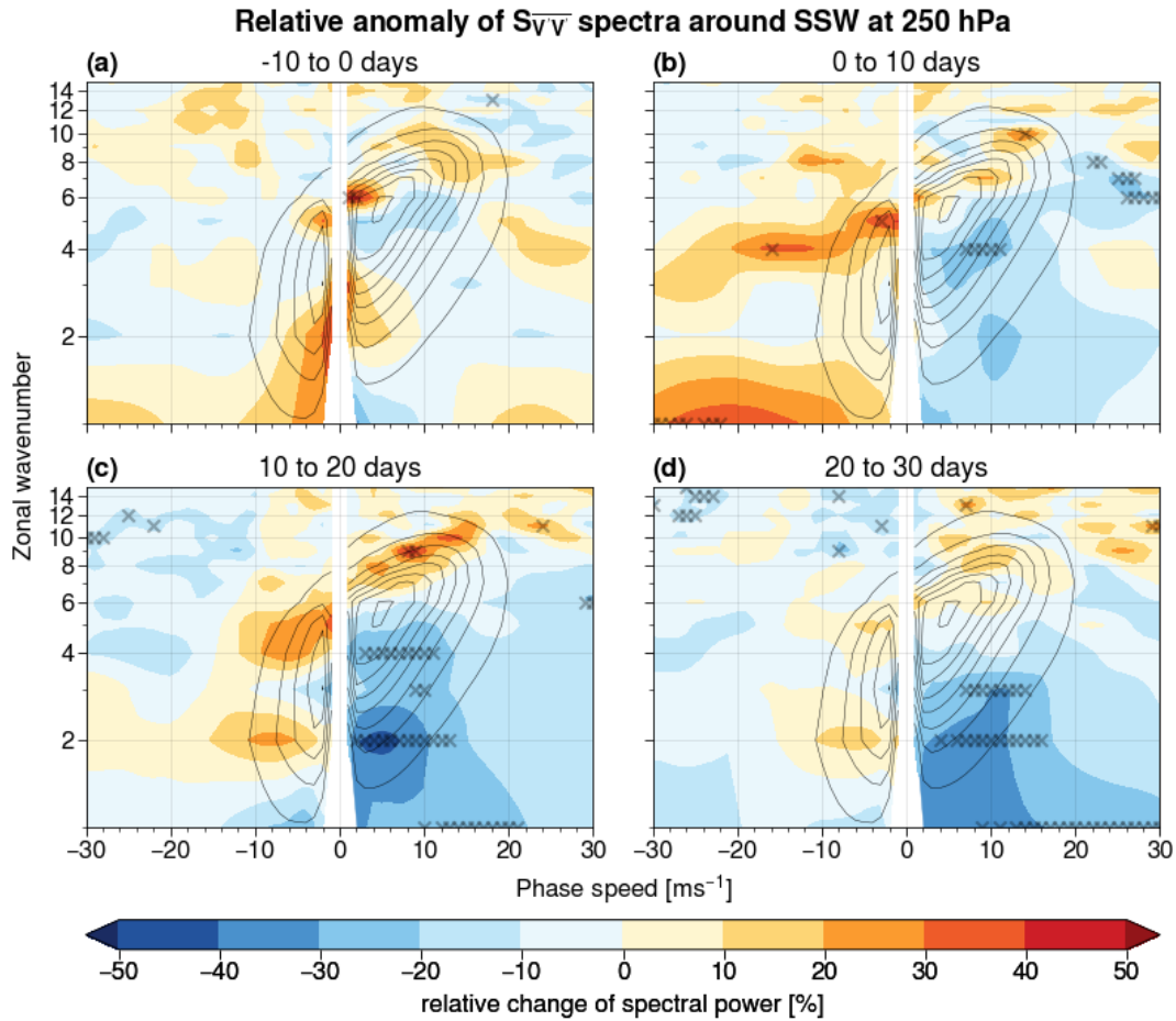
Figure 4. Percentage change of spectral power S_{\sqrt{v}} at 250 hPa with respect to the mean spectrum, averaged over 10-day time intervals, around SSW events (shaded). Subplot (a) shows spectra for 10 days prior to the event to the event start, subplot (b) shows spectra between the event start and 10 days after the event start, (c) for 10 to 20 days, and (d) for 20 to 30 days after the event. Wavenumber-phase speed pairs marked with an \times exceed the 0.5th or 99.5th percentile of the re-sampled distribution. Black contour lines show the NDJFM climatology ranging from 0.1 \text{ m}^2 \text{ s}^{-2} \Delta \text{c}^{-1} to 0.8 \text{ m}^2 \text{ s}^{-2} \Delta \text{c}^{-1} in steps of 0.1 \text{ m}^2 \text{ s}^{-2} \Delta \text{c}^{-1} as in Fig. 1a.
