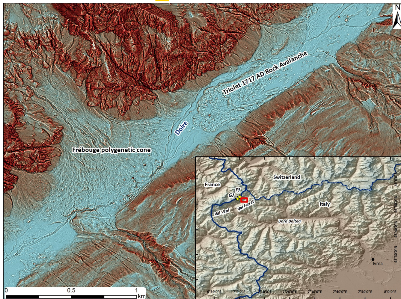
90 Figure 1: The Red Relief Image Map (RRIM) of the Frébouge polygenetic cone and the 1717 AD Triolet rock avalanche. The inset shows the location of the study within the Alpine realm © European Union, Copernicus Land Monitoring Service 2023, European Environment Agency (EEA). PJ = Petites Jorasses and GJ = Grandes Jorasses.
