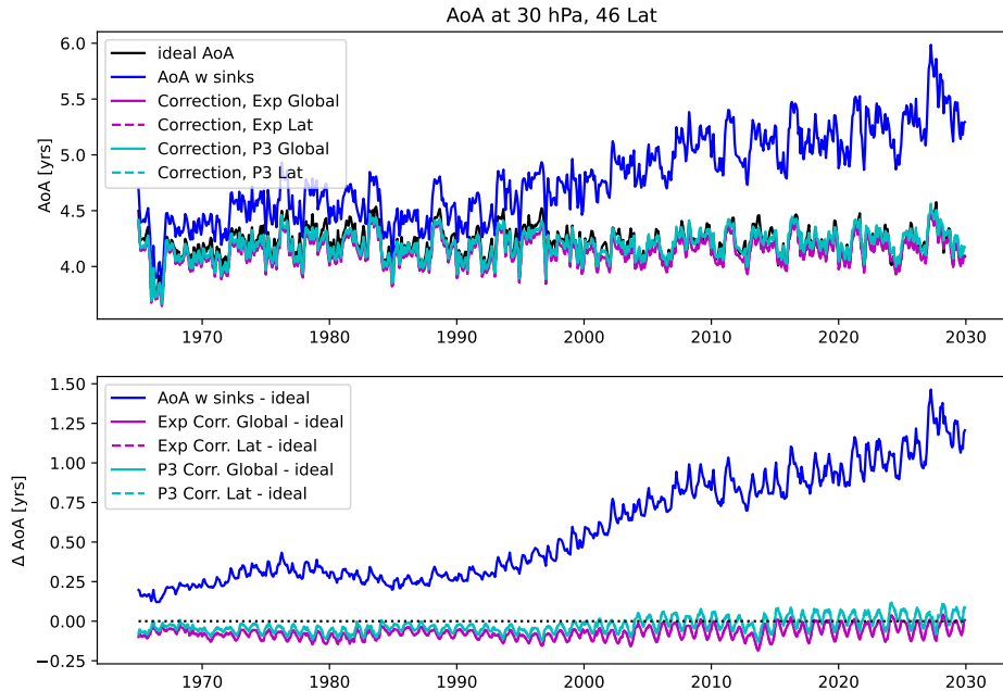
Figure 6. Top: Timeseries of ideal mean AoA (black) in mid-latitudes (46 N) and 30 hPa, together with apparent SF_6 -based AoA (blue), and apparent AoA corrected with the exponential correction scheme (magenta) and the P3 correction scheme (cyan) Bottom: as above, but differences to the ideal mean AoA.
