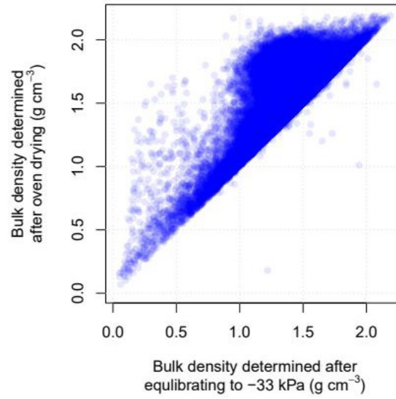
Figure 8: Soil bulk density determined at -33 kPa water content and after oven drying, using data of the USDA- Natural Resources Conservation Service's National Cooperative Soil Survey Soil Characterization Database ( N = 57,512 ). Each dot represents one soil sample.
