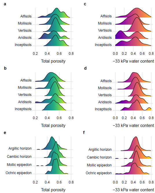
Figure 3: Total porosity and water content at -33 kPa for A-horizons (a, c), B-horizons (b, d) of selected soil orders, and diagnostic horizons (e, f) as defined by US Soil Taxonomy. Data are from the Pedogenic and Environmental Data Set (PEDS).
