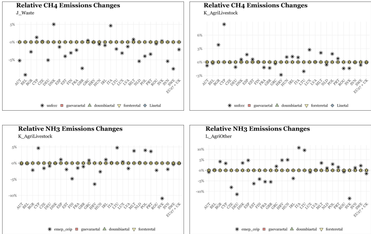
Figure S1: Relative emission changes [%] reported by official (emep_ceip, unfccc) and non-official datasets (guevaraetal, forsteretal, doumbiaetal) per country and at the EU27+UK level for the waste management (GNFR_J) (a) livestock (GNFR_K) (b, c) and other agricultural emissions (GNFR_L) (d)
