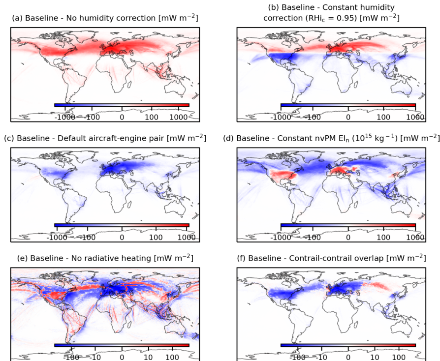
570 Figure 10: Absolute change in the 2019 global annual mean contrail cirrus net RF (in \text{mW m}^{-2} ) when comparing the baseline scenario 575 with the simulation: (a) without humidity corrections applied to the ERA5 HRES; (b) with a constant humidity correction of \text{RH}_i/\text{RH}_c , where \text{RH}_i = 0.95 ; (c) with the default aircraft-engine assignment from BADA3; (d) with a constant \text{nvPM EI}_n of 10^{15} \text{ kg}^{-1} for all waypoints; (e) without radiative heating effects; and (f) that approximates the radiative effects of contrail-contrail overlapping. Basemap plotted using Cartopy 0.21.1 © Natural Earth; license: public domain.
