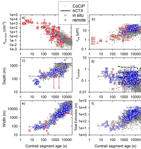
655 Figure 11: Comparison of the simulated contrail properties from CoCiP with in-situ, remote sensing and satellite observations from the contrail library database (COLI) (Schumann et al., 2017) versus the contrail segment age. The contrail properties compared includes the contrail: (a) ice particle number concentration in the plume ( n_{ice,conc} ); (b) r_{ice} ; (c) depth; (d) \tau_{contrail} ; (e) width; and (f) total extinction, i.e., the integral of the optical extinction over the contrail cross-sectional area, which influences the contrail RF'. The red data points are from in-situ measurements, blue data points are from remote sensing, and the black lines in (d) represent the 0 th , 10 th , 50 th , 90 th and 100 th percentiles from the Meteosat Second Generation (MSG) satellites and the automatic contrail tracking algorithm (ACTA) (Vázquez-Navarro et al., 2015). The grey data points are the simulated CoCiP contrail properties from a subset of results within 6-9 UTC in 1-January-2021 and 15-July-2021. 660
