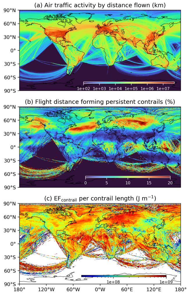
380 Figure 4: The 2019 global: (a) annual flight distance flown; (b) percentage of flight distance forming persistent contrails; and (c) EF_{\text{contrail}} per unit length of persistent contrail formed, where the total EF_{\text{contrail}} throughout the contrail lifetime is added to the pixel where contrails were initially formed. Basemap plotted using Cartopy 0.21.1 © Natural Earth; license: public domain.
