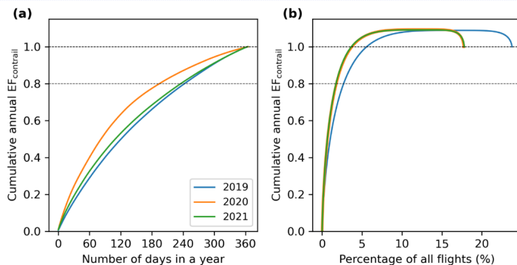
490 Figure 8: Cumulative density function of the global annual EF_{\text{contrail}} from 2019 to 2021 versus the: (a) number of days in a year; and 495 (b) the percentage of all flights that accounted for the proportion of EF_{\text{contrail}} . We note that the cumulative density function in (b) exceeds and returns to 1 because of the presence of flights with cooling contrails.
