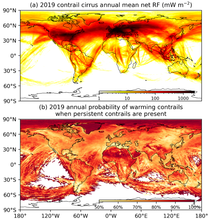
355 Figure 3: The 2019 global: (a) annual mean contrail cirrus net RF; and (b) annual probability of warming contrails, where the hourly contrail net RF is greater than zero when persistent contrails are present in the grid cell. The global annual mean contrail cirrus SW and LW RF, and the annual mean ratio of contrail LW-to-SW RF are shown in Fig. S7 in the Supplement Sect. S3. Basemap plotted using Cartopy 0.21.1 © Natural Earth; license: public domain.
