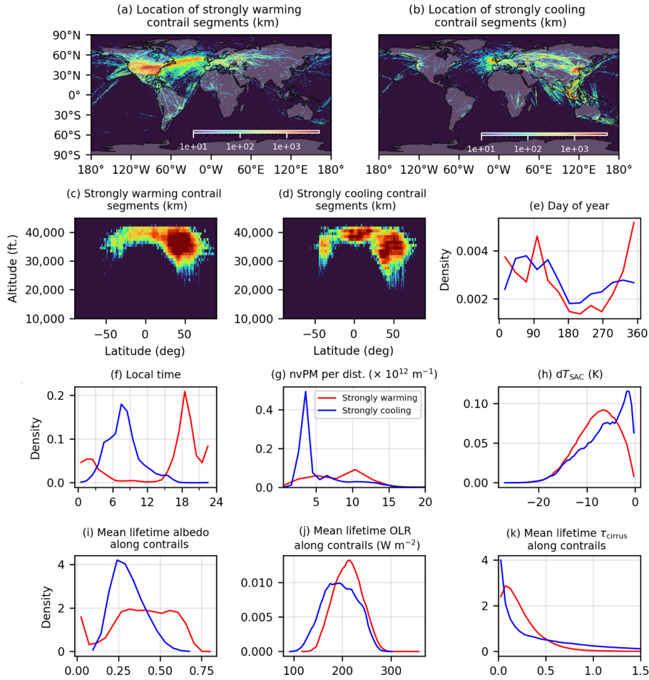
525 Figure 9: The location (longitude, latitude and altitude) of individual contrail segments that are strongly warming ( EF_{\text{contrail}} per contrail length > 15.4 \times 10^8 \text{ J m}^{-1} , 95 th percentile) and strongly cooling ( EF_{\text{contrail}} per contrail length < -2.39 \times 10^8 \text{ J m}^{-1} , 5 th percentile), shown in subplots (a) to (d); and probability density functions showing their respective day of year; (f) time of day; (g) nvPM emissions; (h) the dT_{\text{SAC}} when these contrails were initially formed; and their mean (i) effective albedo; and (j) outgoing longwave
