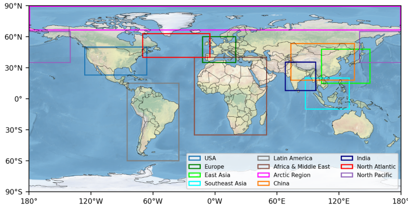
Figure 2: Spatial bounding box used to estimate the regional air traffic, emissions, and contrail properties. The specific dimensions of these bounding boxes can be found in Table S5 in the Supplement. Basemap plotted using Cartopy 0.21.1 © Natural Earth; license: public domain.
