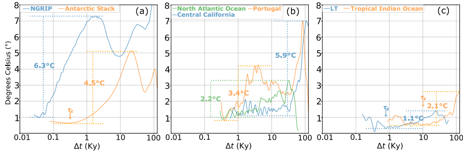
Figure 9. Absolute amplitude differences of the fluctuations for calibrated temperature datasets in degrees Celsius. Shown are (a) polar regions, (b) northern mid-latitudes, (c) tropics. The numbers accompanying the vertical lines estimate the fluctuation amplitude, equivalent to the difference between the peak found at multi-millennial scales minus the minimum found at multi-centennial or millennial scales. Some \tau_c values are shown as reference according to the findings from Figures 4 to 8.
