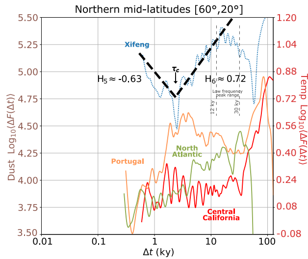
Figure 5. Haar RMS values derived from the northern mid-latitudes records. Temperature proxies are displayed as continuous lines, while dust proxies as dotted lines. Refer to Figure 4 for detailed annotations and references.
