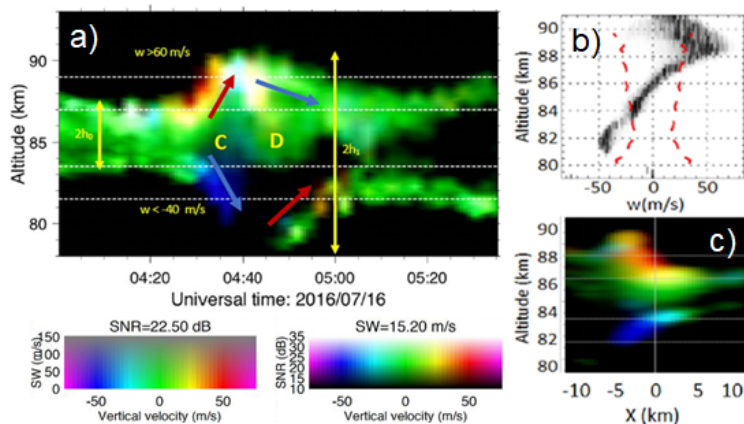
Figure 1. Summary of an observed extreme vertical velocity event with MAARSY. (a) Time evolution of the vertical velocities between 75 and 95 km altitude over a time period of 1.5 hours. The red and blue colors indicate the strong up- and downdrafts, respectively, green indicates vertical velocities around 0 m/s, and the brightness of the colors represents the strength of the signal (SNR). (b) One example of the vertical velocity spectra during the event with the 3\sigma presented as the red dashed lines. (c) A cut through the event and showing the horizontal extent at one specific time (adapted from Chau et al. (2021)).
