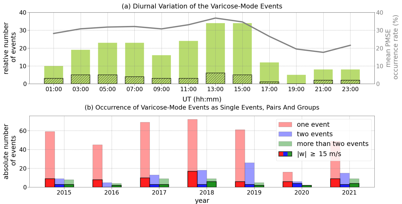
Figure 6. (a) The distribution of the relative occurrence of events in varicose mode over the course of a day. The gray line illustrates the mean diurnal variation in the frequency of PMSE by Latteck et al. (2021). (b) The absolute number of varicose mode events occurring as single events, as pairs, or in groups for each individual year.
