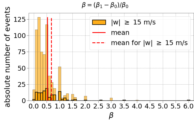
Figure 9. Normalized bore amplitudes of the varicose mode events in general. The red solid (dashed) line represents the mean of all events (events with |w| \geq 15 m/s).
