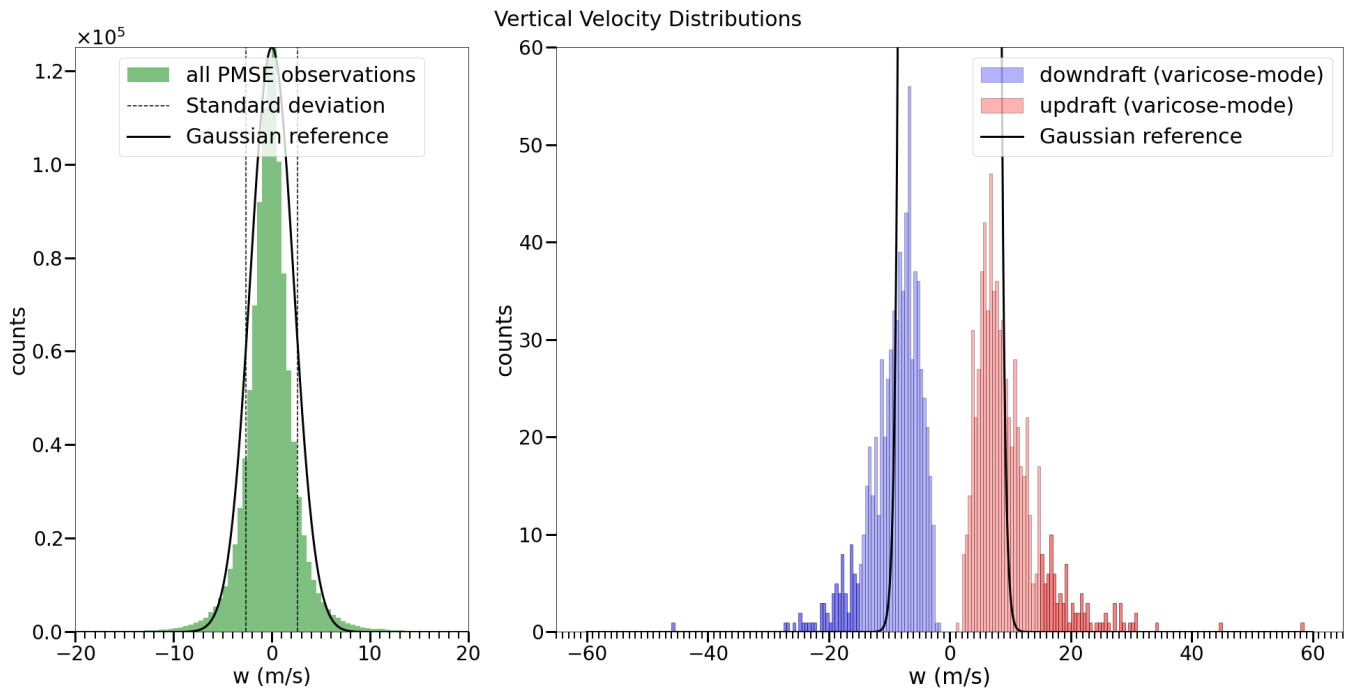
Figure 8. Distribution (a) of vertical velocities across all altitudes and throughout the observation period and (b) of the maximum vertical velocities of varicose-mode events in blue (down-drafts) and red (up-drafts). In both panels, the black curve represents a Gaussian reference.
