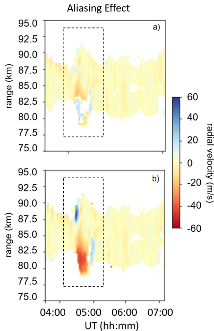
Figure 3. The colored contours show the vertical velocity (a) observed on July 16, 2016 after applying 6 additional coherent integrations (effective v_{\text{rad}} = 140 m/s) and (b) without applying additional coherent integrations (effective v_{\text{rad}} = 175 m/s) over altitude. The velocities cannot be determined from the spectra due to filtering and thus are missing in (ba).
