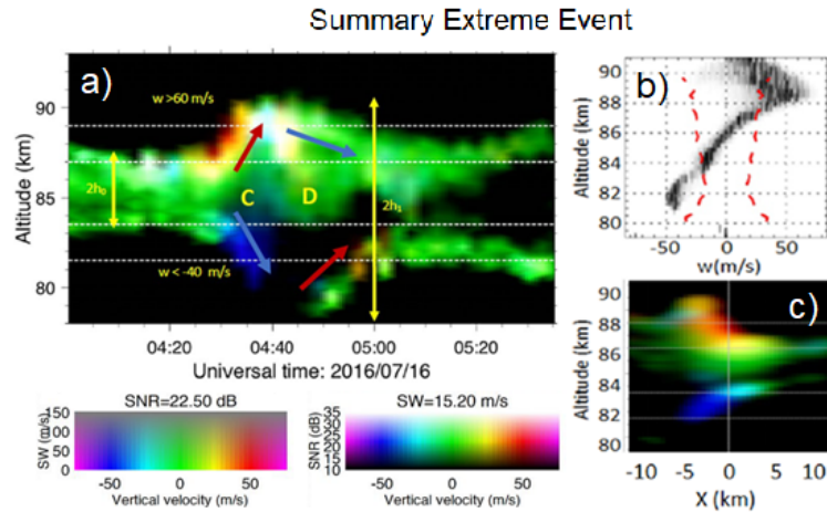
Figure 1. Summary of the highlights of an observed extreme vertical velocity event with MAARSY. (a) Time evolution of the vertical velocities between 75 and 95 km altitude over a time period of 1.5 hours. The red and blue colors indicate the strong up- and downdrafts, respectively, green indicates vertical velocities around 0 m/s, and the brightness of the colors represents the strength of the signal (SNR). (b) One example of the vertical velocity spectra during the event with the 3\sigma presented as the red dashed lines. (c) A cut through the event and showing the horizontal extent at one specific time (adapted from Chau et al. (2021)).
