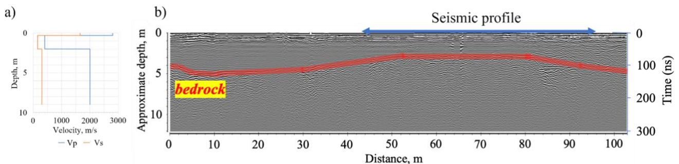
140 Figure 4: (a) Near-surface 1-D velocity model of Talvikangas district of Oulu with the uppermost frozen layer of 30 cm added. (b) results of GPR survey.
