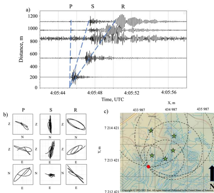
205 Figure 6: The strongest frostquake, detected on 6.1.2023 in Talvikangas: a) vertical component seismograms; b) particle motion diagrams for P- S- and Rayleigh (R) waves; c) location of the epicenter indicated by red dot.
