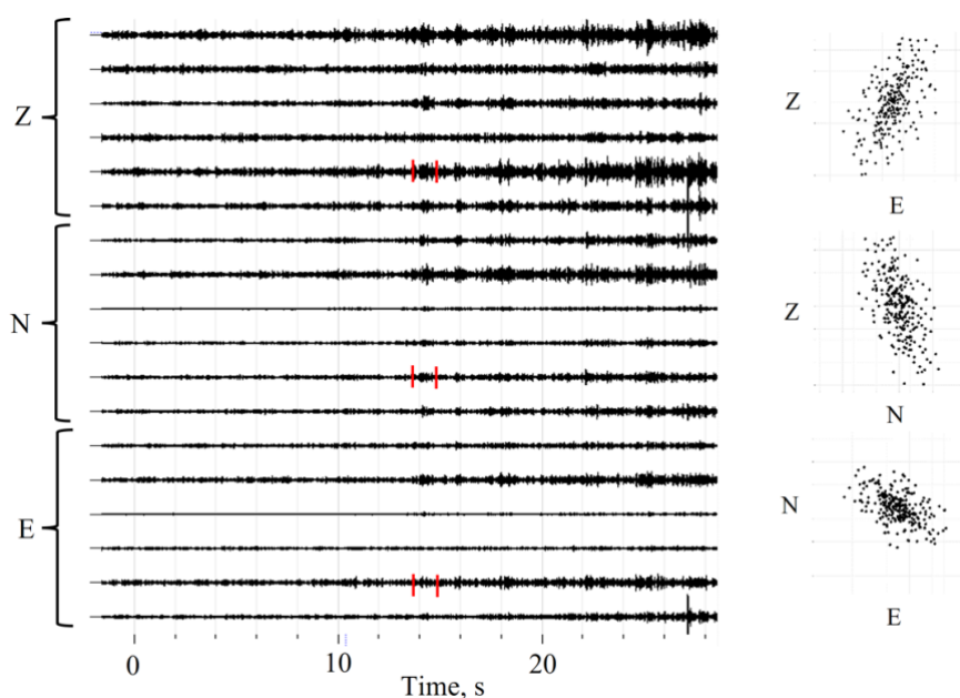
Figure 9: An example of tremors swarm on frequency band of 120-180 Hz, recorded by our seismic arrays (a). Red lines indicate a single tremor signal recorded by the single array station. (b) particle motion diagrams of typical tremor showing elliptical polarization.
