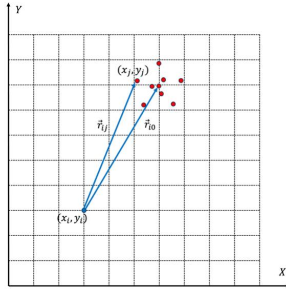
275 Figure 11: Geometry illustrating direct search location algorithm: blue dot show source position been tested; the blue dot shows the source position being tested; the red dots show the locations of seismic sensors.
