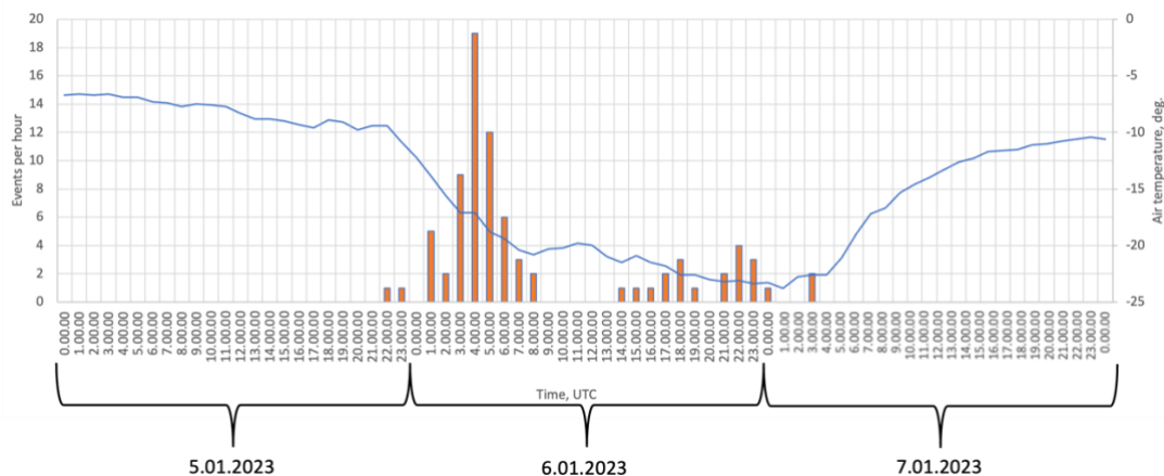
Figure 13: Number of seismic events per hour, recorded by seismic array in Talvikangas 5.01.2023-7.01.2023.
