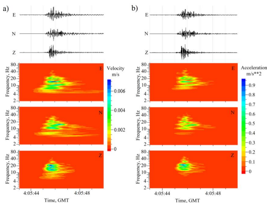
225 Figure 8: Seismic records and corresponding spectrograms of the strongest frostquake in Talvikangas on 6.1.2023, recorded by the closest seismic array to epicenter (epicentral distance is about 300 m): a) ground velocities; b) ground accelerations.
