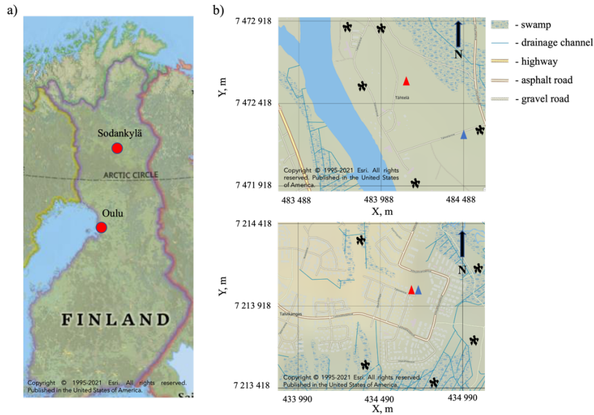
90 Figure 1: (a) Geographical position of two sites of experiment in Northern Finland during winter, 2022-2023. (b) Installations of seismic arrays and soil stations in Tähtelä (upper panel) and Talvikangas (lower panel) blue triangles show soil stations; red triangles show broadband seismic stations; black dots indicate arrays of short period seismic stations. Coordinate system is EUREF_FIN_TM35FIN. (units are in metres; X is Easting and Y is Northing)
