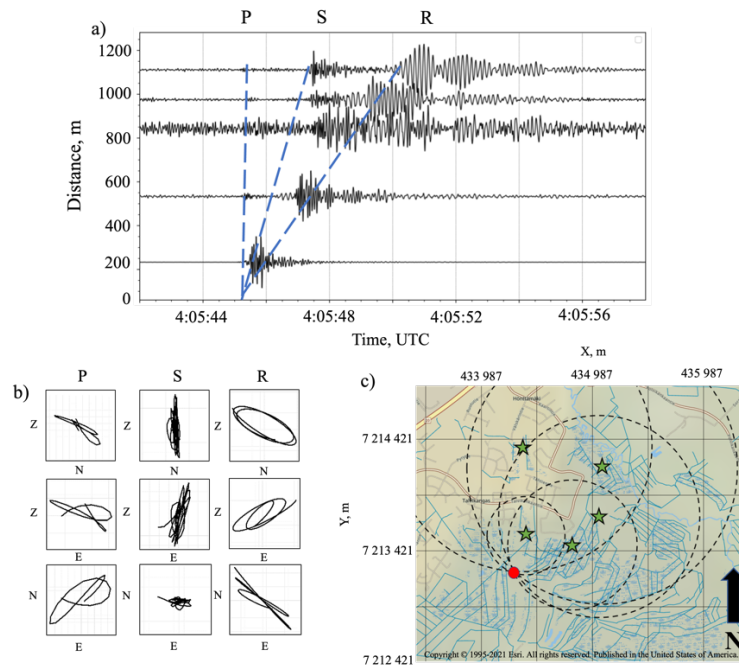
215 Figure 6: The strongest frostquake, detected on 6.1.2023 in Talvikangas: a) stacked vertical component seismograms pre-filtered by bandpass filter 2-20 Hz; b) particle motion diagrams for P- S- and Rayleigh (R) waves; c) location of the epicenter indicated by red dot.
