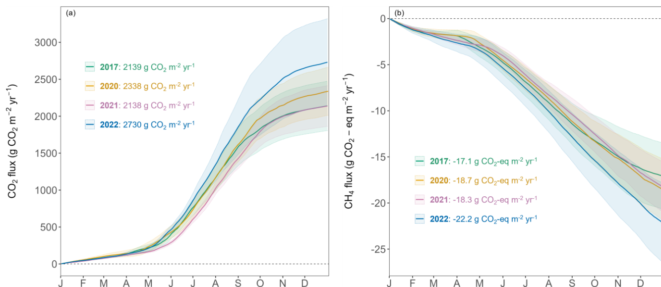
Fig. 5: Cumulative forest-floor (a) respiration ( \text{g CO}_2 \text{ m}^{-2} \text{ yr}^{-1} ) and (b) \text{CH}_4 ( \text{g CO}_2\text{-eq m}^{-2} \text{ yr}^{-1} ) fluxes over four years. Lines show means of all four chambers; colored bands represent standard deviations among four chambers.
