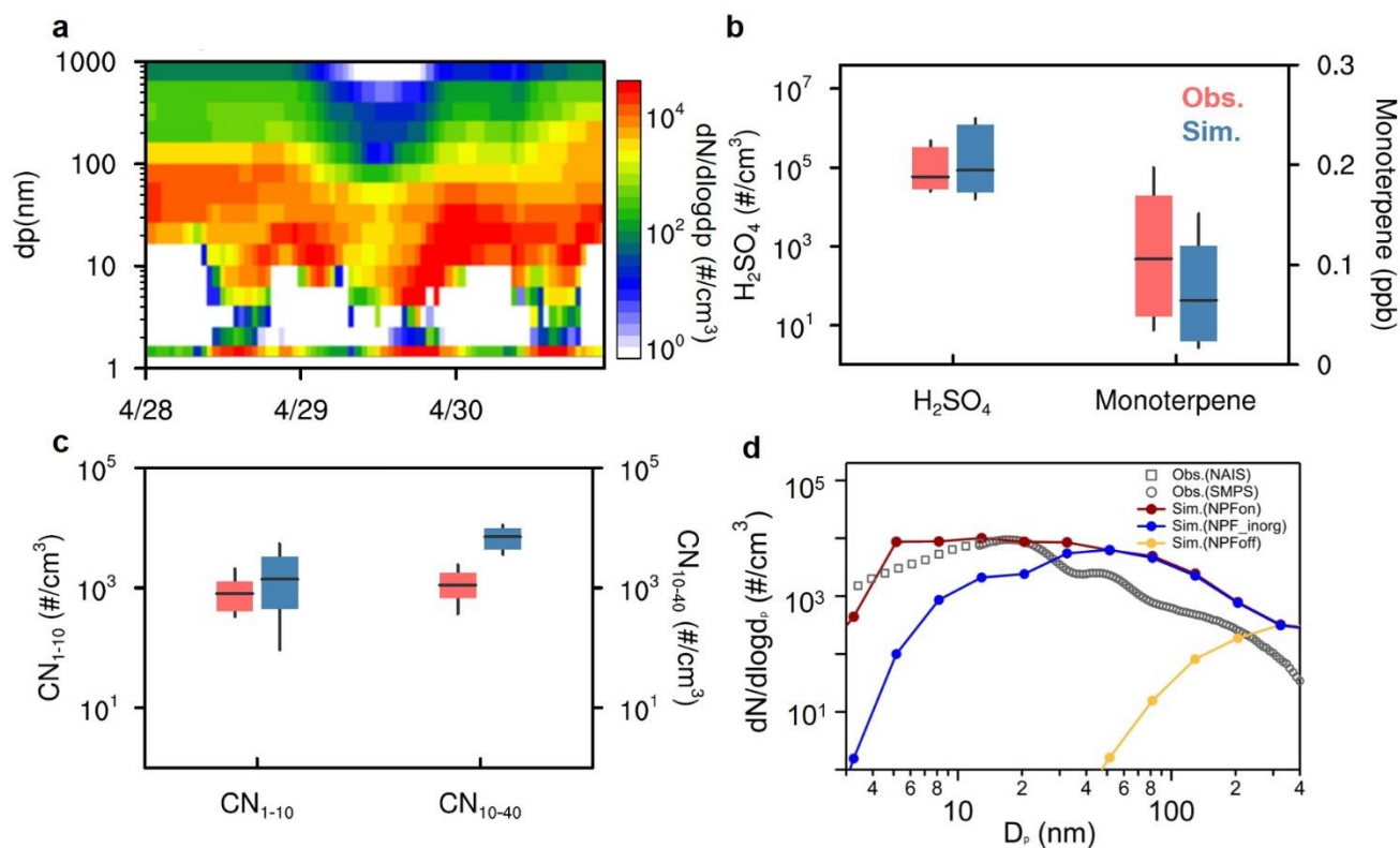
385 Figure 5. (a) Simulated particle number size distribution in Lulang. (b) Observed and simulated H_2SO_4 and monoterpene concentration in Lulang. The horizontal lines of box represent the 66 th percentile, median and 33 rd percentile and the whiskers represent the 75 th and 25 th percentiles. (c) Same as Fig. 5b but for number concentrations of 1–10 nm and 10–40 nm particles. (d) The observed and simulated particle number size distributions averaged from 12:00 to 18:00 (UTC+8) during 28–30 April. The gray squares and gray circles show the measurements by NAIS and SMPS, respectively. Red, blue and 390 orange lines represent the NPF-on, NPF_inorg and NPF-off experiments.
