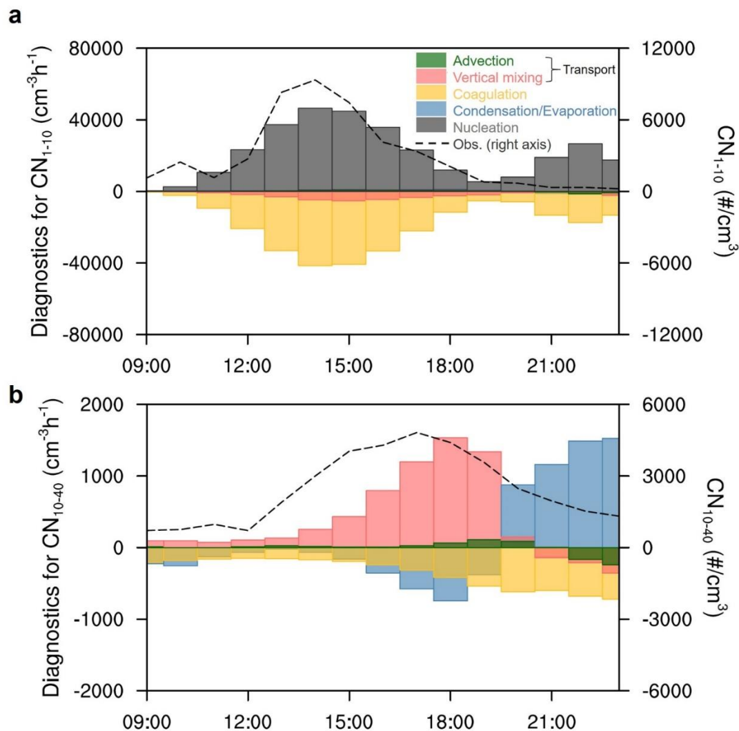
455 Figure 9. (a) Diurnal evolution of contributions of near-surface 1–10 nm particle number concentrations from different processes calculated by WRF-Chem processes analysis during 28–30 April over the research domain. The black dashed line represents the diurnal evolution of observed 1–10 nm particle number concentrations during 28–30 April. (b) Same as Fig. 9a but for 10–40 nm particle number concentrations.
