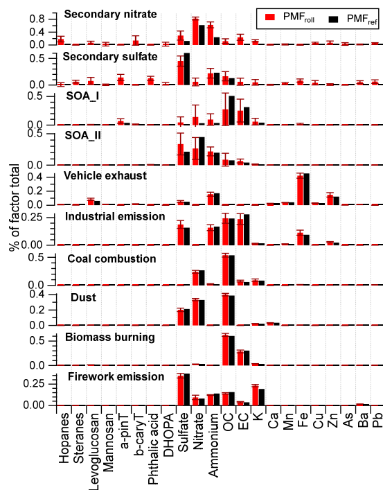
Figure 6. Comparison of the source profiles (% of factor total) derived from the short-term rolling PMF runs ( PMF_{roll} ) and the reference profiles from PMF_{ref} . Error bars represent one standard deviation of profile variability across the PMF_{roll} runs.
