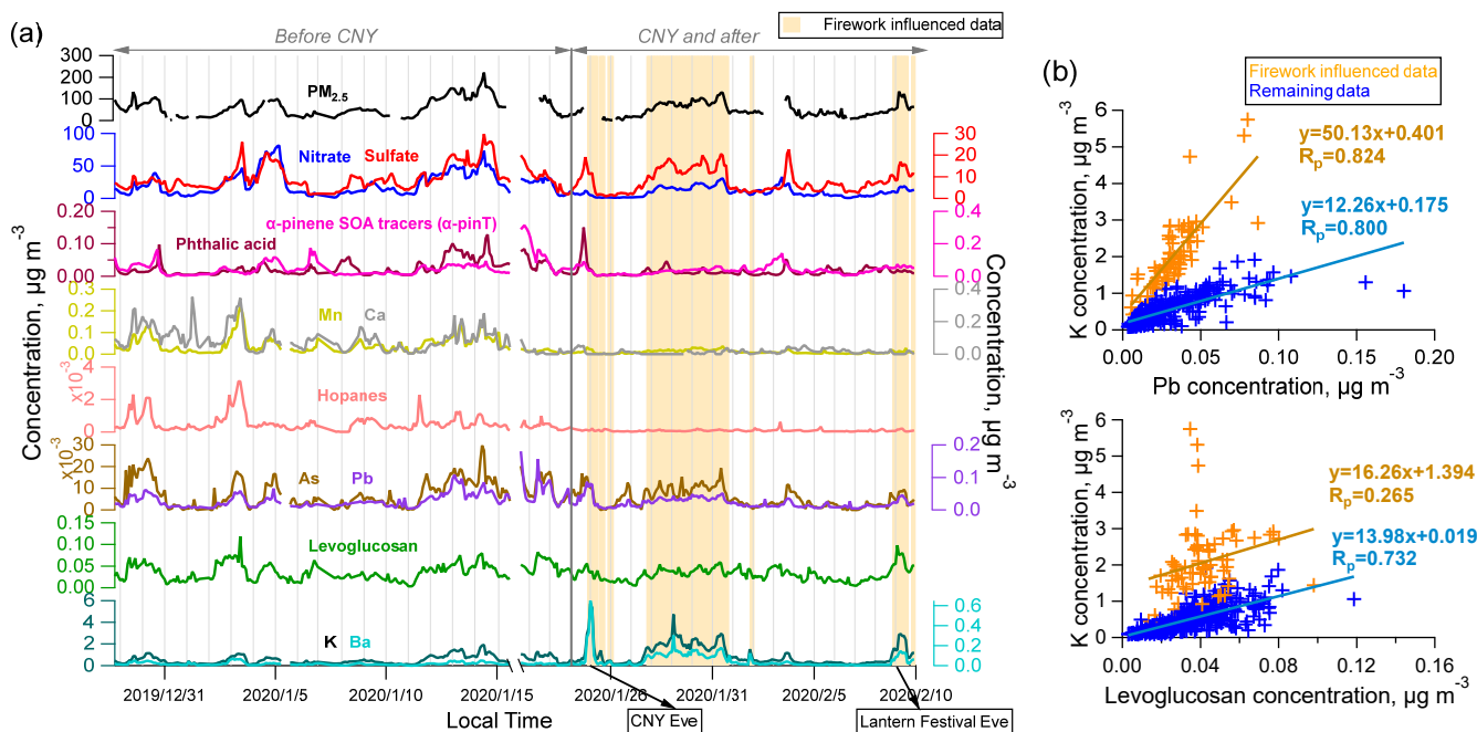
190 Figure 2. (a) Time series of concentrations of total PM 2.5 and selected tracer species from 29 Dec. 2019 to 9 Feb. 2020 at the DSL site in Shanghai. The campaign period was divided into two phases: before Chinese New Year (CNY) and CNY and post-CNY period. The data influenced by firework emissions are highlighted in light orange. (b) Scatter plots illustrating the relationship between K concentrations and two other tracer species, Pb and levoglucosan, during the firework-influenced period and the remaining period.
