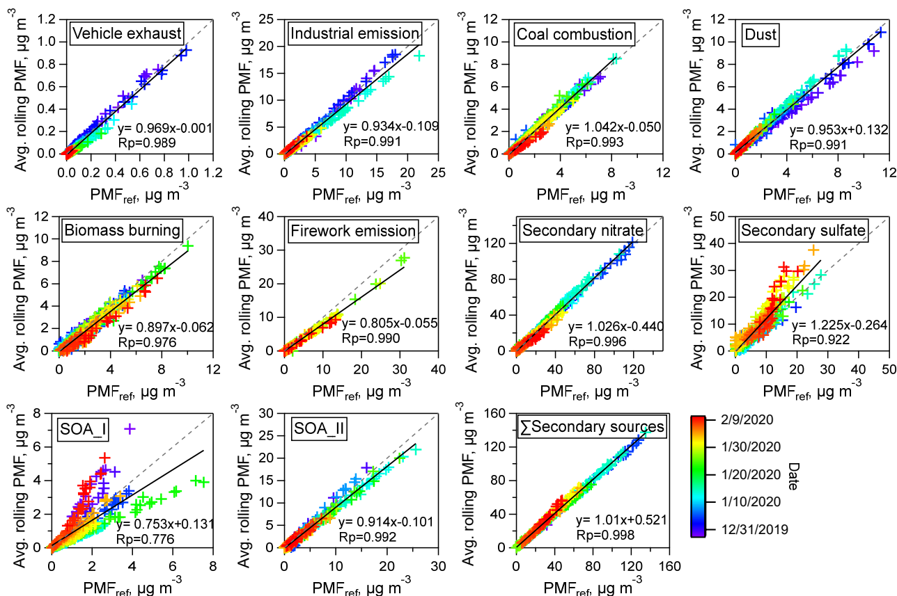
Figure 5. Comparison of the PM 2.5 source contributions obtained from average PMF rolling runs with the reference result in PMF ref for individual source factors and the sum of the four secondary sources.
