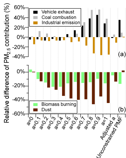
235 Figure 3. Relative differences in PM 2.5 contribution between different \alpha -value constrained runs and the unconstrained PMF run, compared to the reference result, for (a) vehicle exhaust, coal combustion, and industrial emission, and (b) biomass burning and dust. The “adjusted \alpha ” indicated the final \alpha values adopted, i.e., \alpha=0.3 for vehicle exhaust, coal combustion, and industrial emissions, and \alpha=0.1 for biomass burning and dust.
