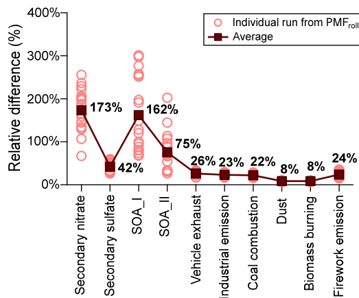
Figure 7. The relative difference in the resolved source profiles among the individual rolling PMF runs. The relative difference for individual rolling PMF run (empty circles) was calculated as the average value of the relative difference for all input species. Solid squares represent the average value from all rolling PMF runs.
