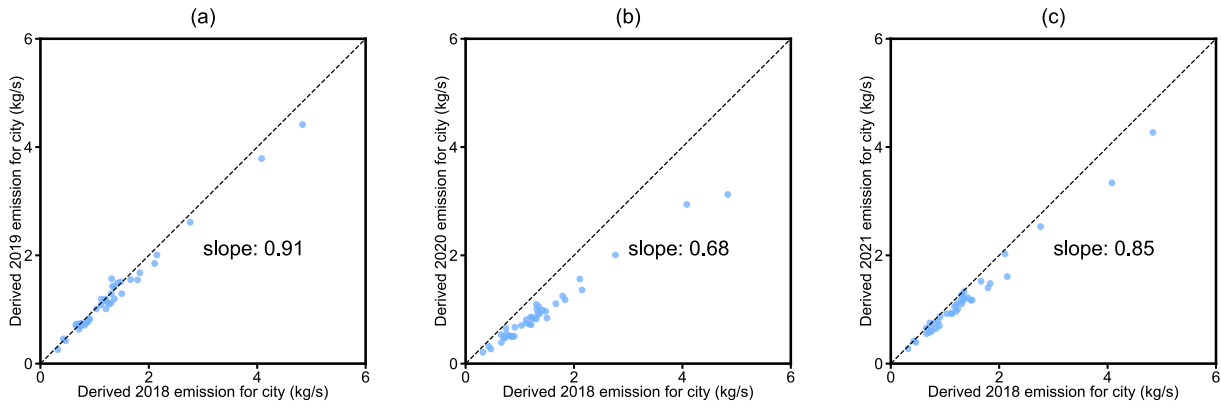
535 Figure 6: Comparison of TROPOMI-derived NO x emission estimates for (a) 2019, (b) 2020, (c) 2021 with those for 2018. The dashed line represents the 1:1 line. The slope of the least-squares linear regression line is provided in the figure.
