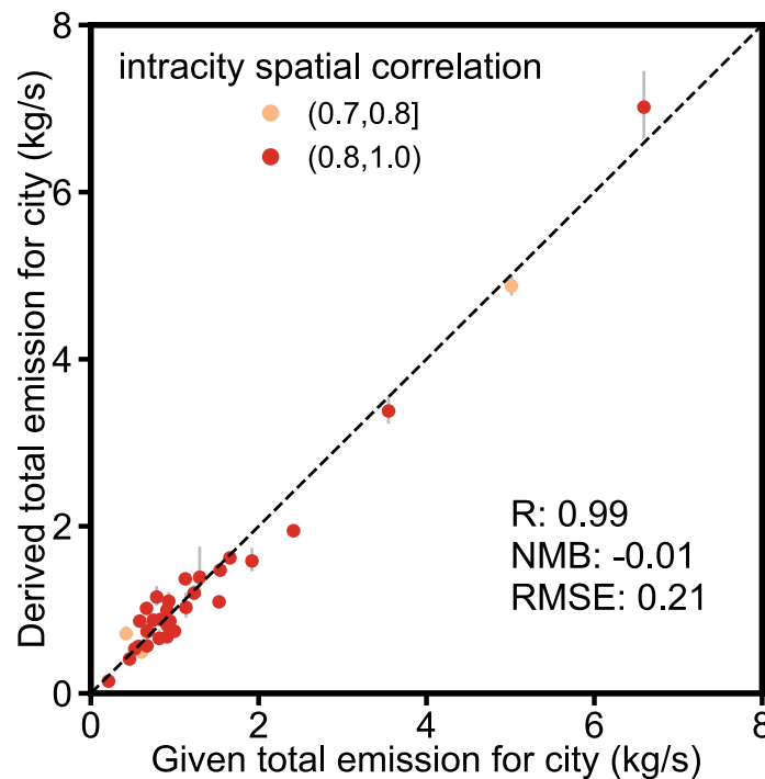
Figure 2: Scatterplot of the derived \text{NO}_x total emissions for the investigated cities based on the \text{NO}_2 tropospheric VCDs simulated by NU-WRF (y axis) as compared to the given emissions used to drive the NU-WRF simulation (x axis). \text{NO}_x emissions from all grid cells within the domain of 70 \text{ km} \times 70 \text{ km} around city center are summed up to derive the total emission for most cities; a 100 \text{ km} \times 100 \text{ km} domain is used for New York, Chicago, Los Angeles and Houston. Error bars show the standard error of the
