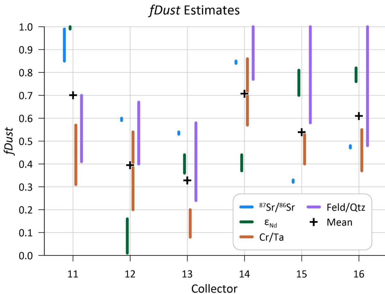
435 Figure 11. Summary of fDust estimates made at the six study sites with four mixing models: ^{87}\text{Sr}/^{86}\text{Sr} and \epsilon_{\text{Nd}} , Cr/Ta, and Feld/Quartz. Vertical extent of each bar reflects the range of estimates for a given approach at a given site. The black crosses represent the overall mean at each site
