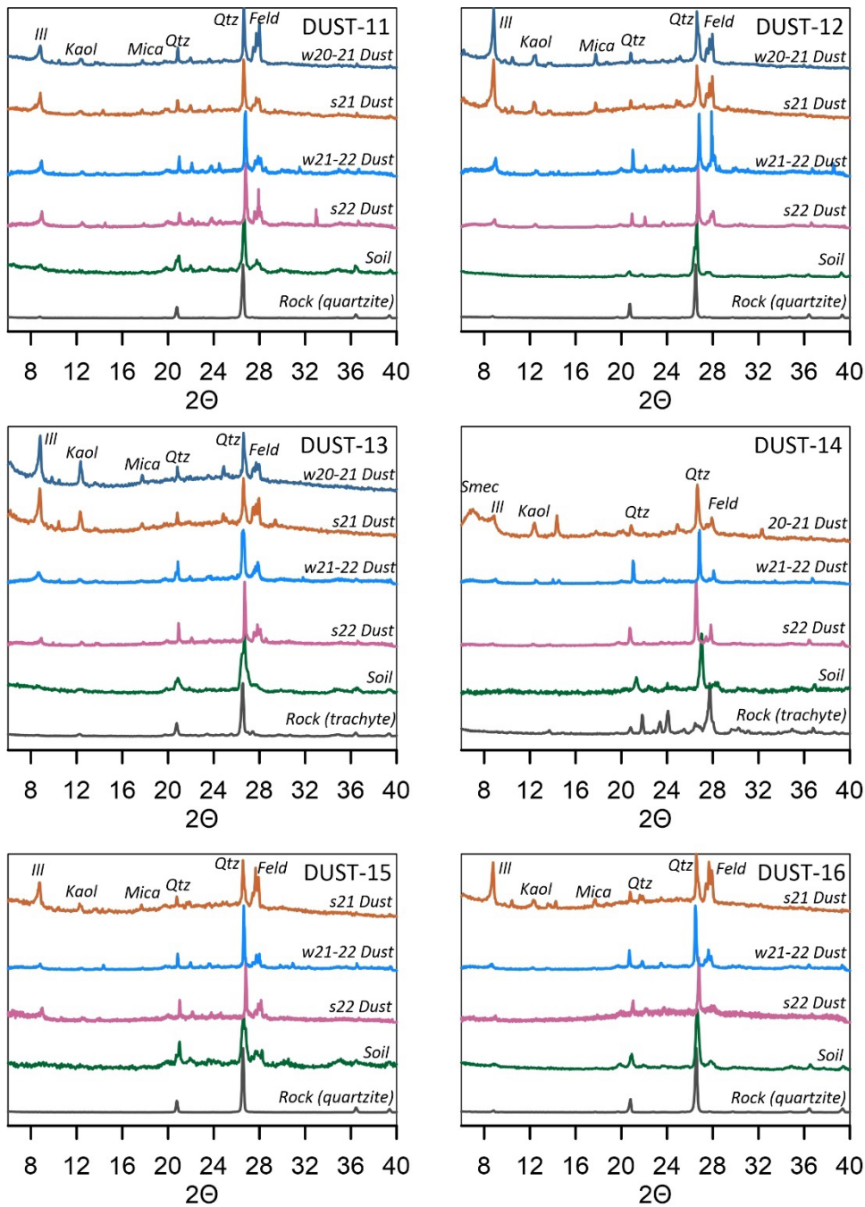
350 Figure 6. X-ray diffraction (XRD) results for samples of dust, soil, and rock at the six study sites. Individual dust samples are presented to emphasize the general seasonal and interannual consistency of dust composition. “w20-21” is dust accumulating during the winter of 2020-21. “s21” is dust from summer 2021. “w21-22” is dust from the winter of 2021-22. “s22” is dust from summer 2022. Soil and rock samples are a composite of the individual samples collected at each site. Prominent mineral peaks are identified: “Ill” is illite, “Kaol” is kaolinite, “Mica” indicates K-mica, “Qtz” is quartz, and “Feld” is Ca and Na feldspar.
