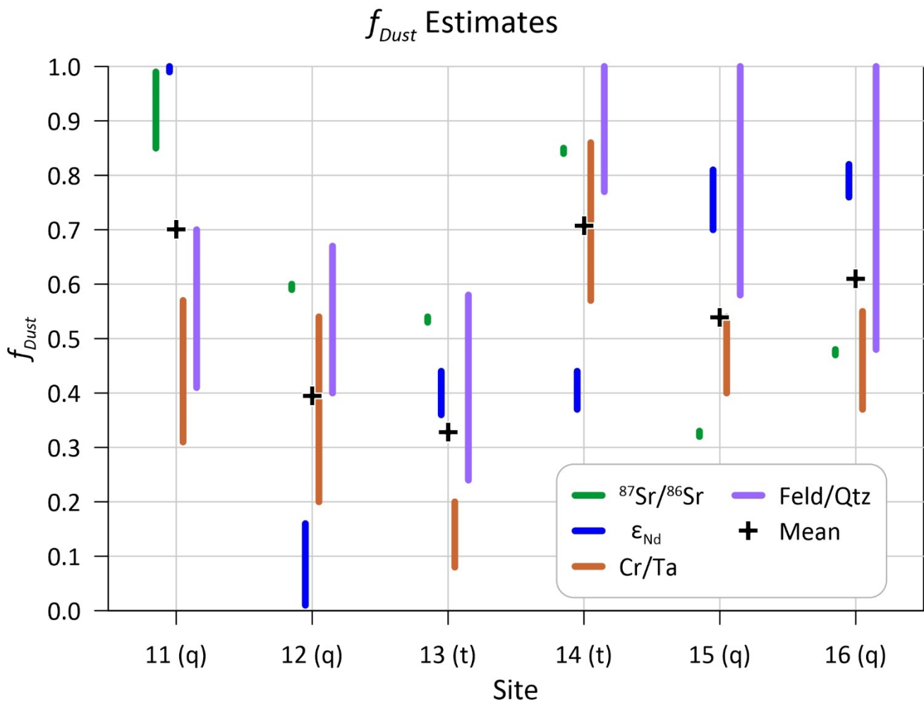
450 Figure 11. Summary of f_{Dust} estimates at the six study sites (X-axis) from four mixing models: ^{87}\text{Sr}/^{86}\text{Sr} and \epsilon_{Nd} , Cr/Ta, and Feld/Quartz. Vertical extent of each bar reflects the range of estimates for a given approach at a given site. The black crosses represent the overall mean at each site. “q” designates quartzite bedrock; “t” denotes trachyte.
