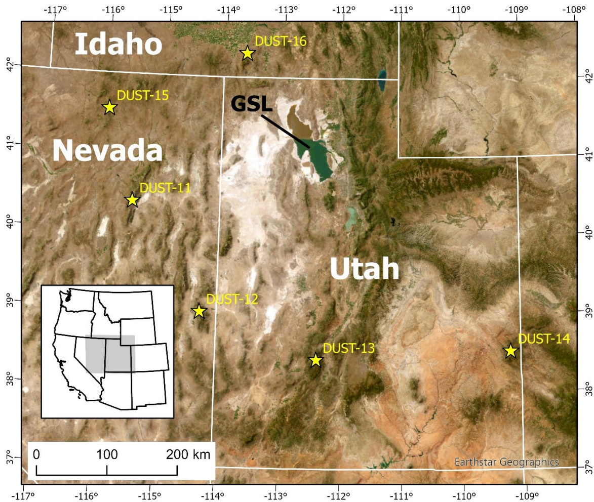
65 Figure 1. Map presenting the locations of the six passive dust collectors utilized in this study (yellow stars). Background is a true-color satellite image from Earthstar Geographics (World Imagery - Overview, 2023). Inset shows the location of the main map (gray rectangle) in the western United States. The states of Utah, Nevada and Idaho are identified. GSL denotes the Great Salt Lake in northern Utah.
