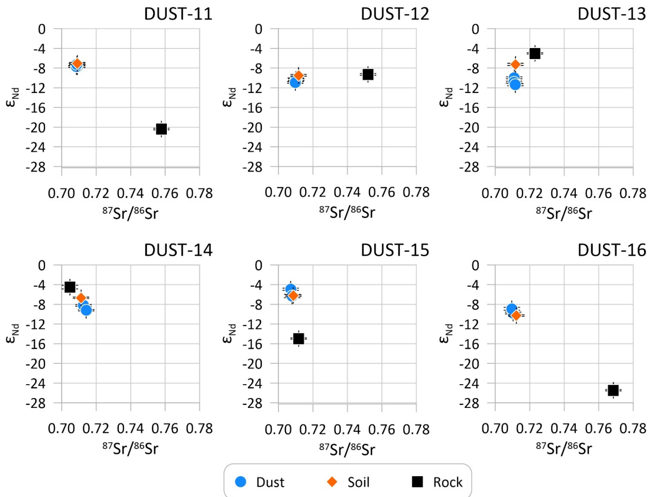
435 Figure 9. Biplots of ^{87}Sr/^{86}Sr and \epsilon_{Nd} of soil, dust, and rock samples at the six study sites. Symbols represent the mean \pm 1 standard error.
