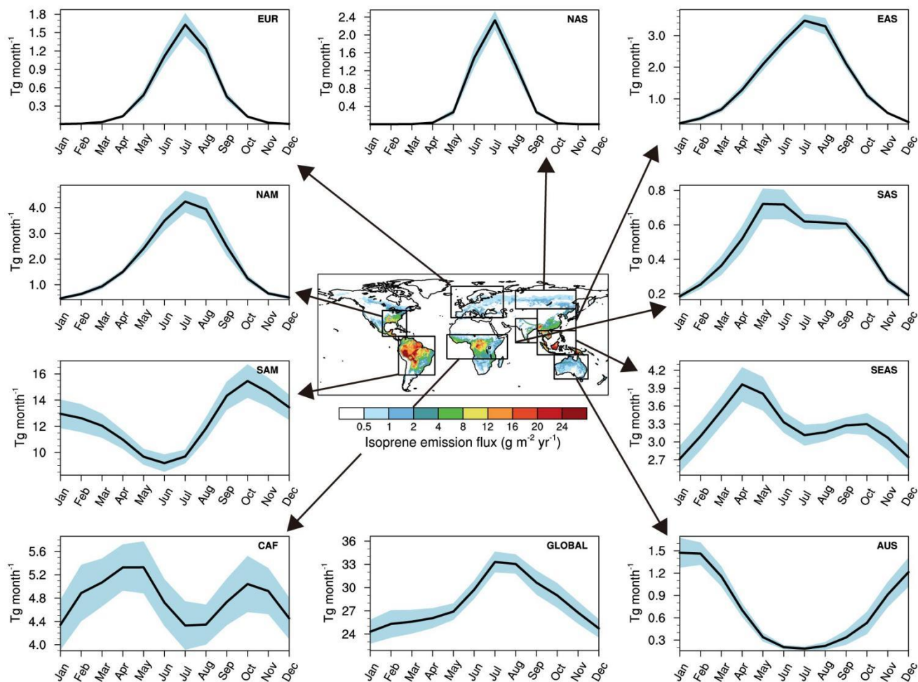
330 Figure 4: The seasonal variation of isoprene emissions for each region outlined in black on the map averaged during 2001-2020. The shaded area represents one standard deviation. The nine regions are listed below: NAM: North America; EUR: Europe; NAS: North Asia; EAS: East Asia; SAS: South Asia; SEAS: Southeast Asia; SAM: South America; CAF: Central Africa; AUS: Australia.
