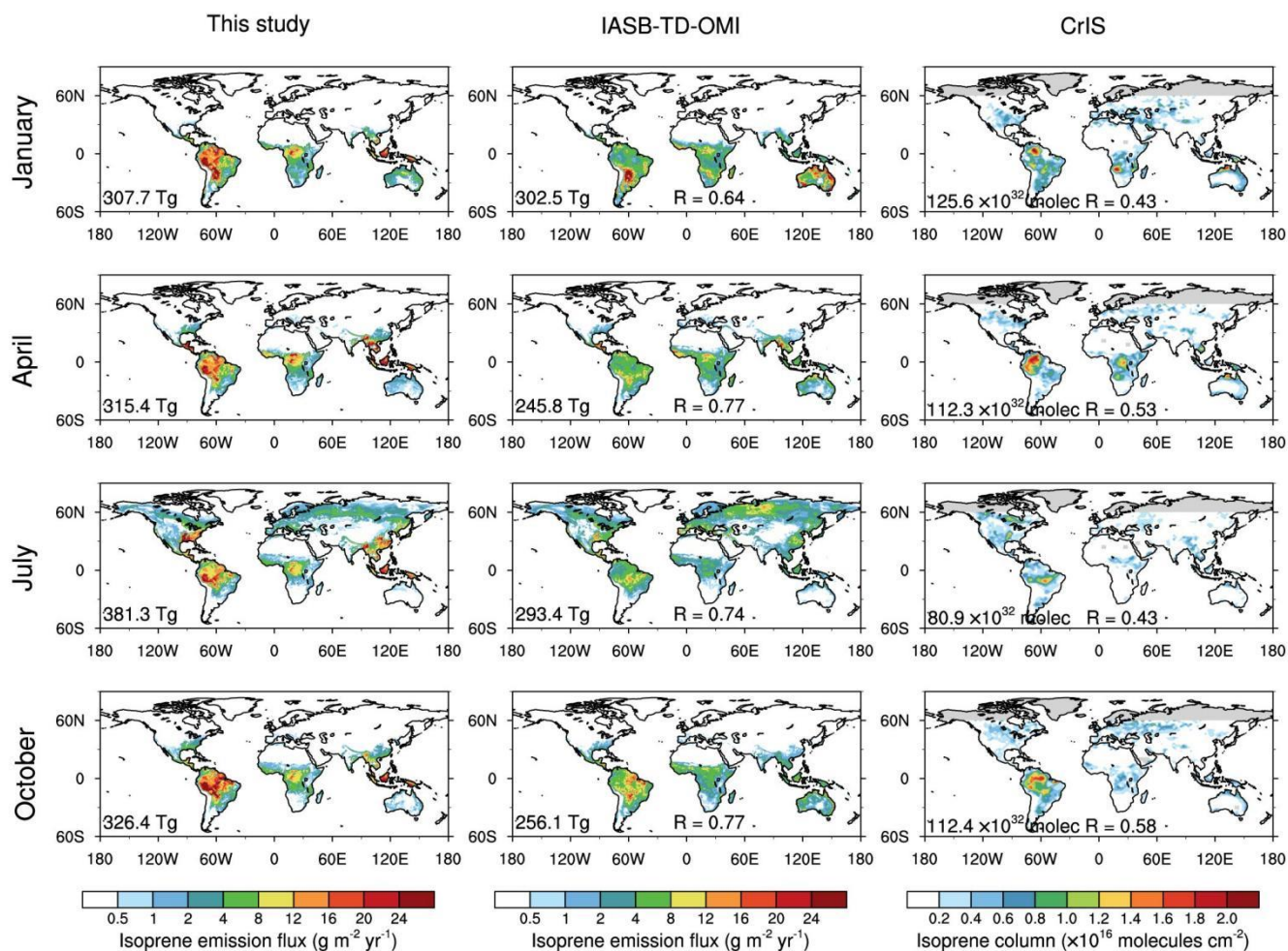
255 Figure 2: The comparison of (left column) simulated isoprene emission fluxes ( 0.5^\circ \times 0.5^\circ ) with (middle column) IASB-TD-OMI ( 0.5^\circ \times 0.5^\circ ) and (right column) CrIS data ( 2^\circ \times 2.5^\circ ) in January, April, July, and October of 2013. The annual global emission or burden are given at the bottom-left of each panel. The correlation coefficients R of the simulation results with IASB-TD-OMI and CrIS are marked in the subplots in the middle and right columns, respectively. Gray shade denotes the region where data is not available.
