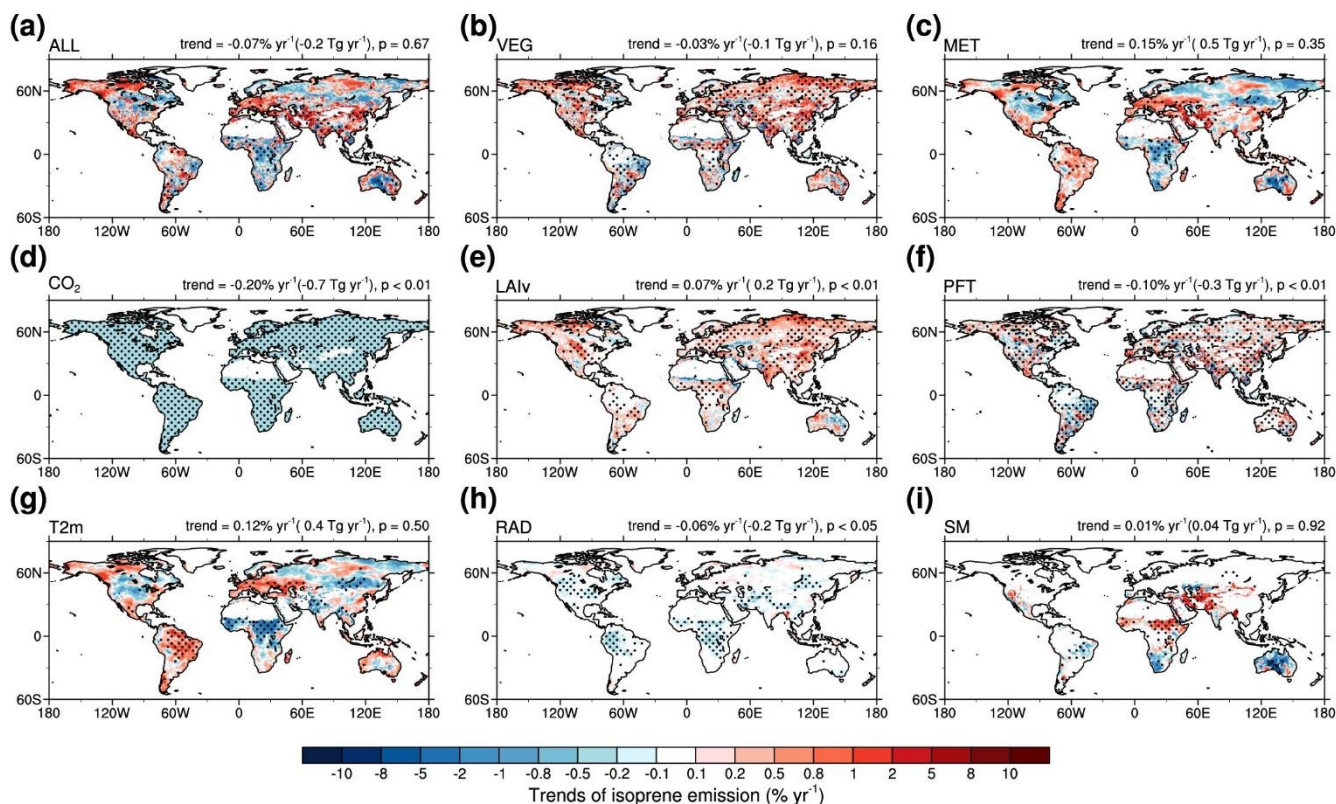
470 Figure 8: Spatial distribution of isoprene emission trends from 2001 to 2020. (a) ALL represents simulated results considering interannual variability of all drivers. (b, c, and d) VEG, MET, and CO 2 represent simulated trends when considering only interannual variability of vegetation, meteorology, and CO 2 concentrations, respectively. (e, f) Contributions from individual vegetation parameters including LAIv (leaf area index of vegetation covered surfaces) and PFT (plant functional types). (g, h, and i) Contributions from individual meteorological factors including T2m (surface 2 m temperature), RAD (surface solar radiation), and SM (soil moisture). Stippling denotes regions where the trend is statistically significant (p < 0.1) using the Mann-Kendall test. Trends are expressed by the relative change in percentage (i.e., the linear change during 2001-2020 divided by the mean value) and absolute change. p-values represent statistically significant levels using the Mann-Kendall test.
