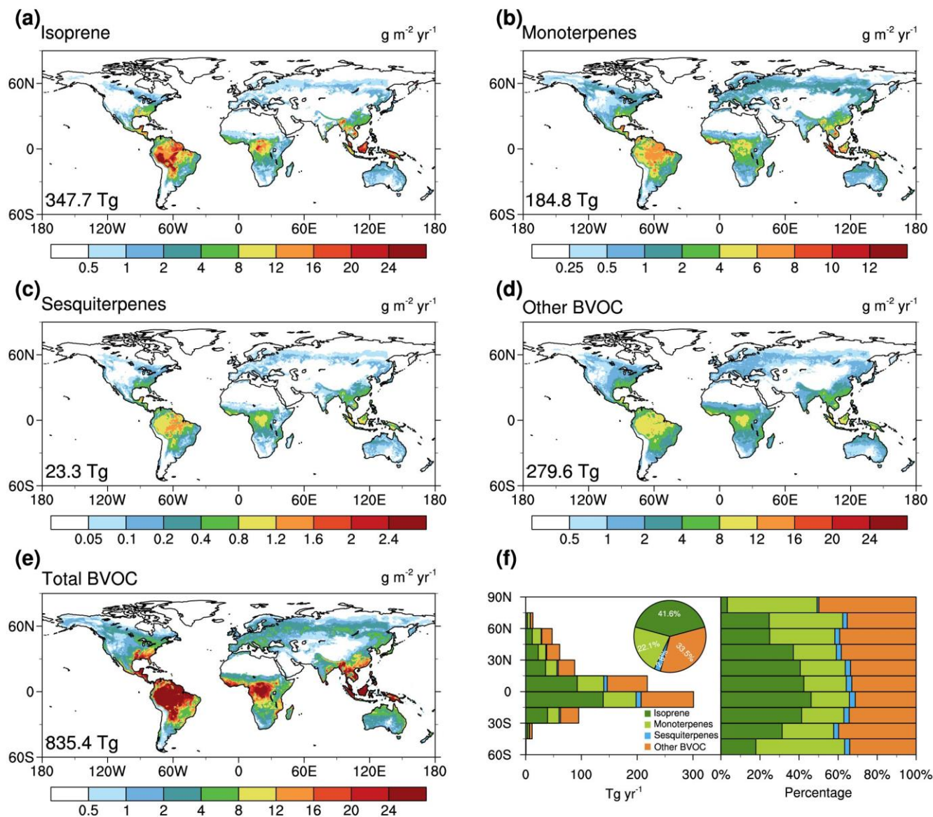
270 Figure 3: The spatial pattern of the annual average BVOC emission fluxes of (a) isoprene, (b) monoterpenes, (c) sesquiterpenes, (d) other BVOCs, (e) total BVOC, and (f) the latitudinal distribution (left: total emission, right: fraction of each category; pie chart: the fraction of each category in global total emissions) for the period 2001–2020. The annual global emissions are given at the bottom-left of each subplot.
