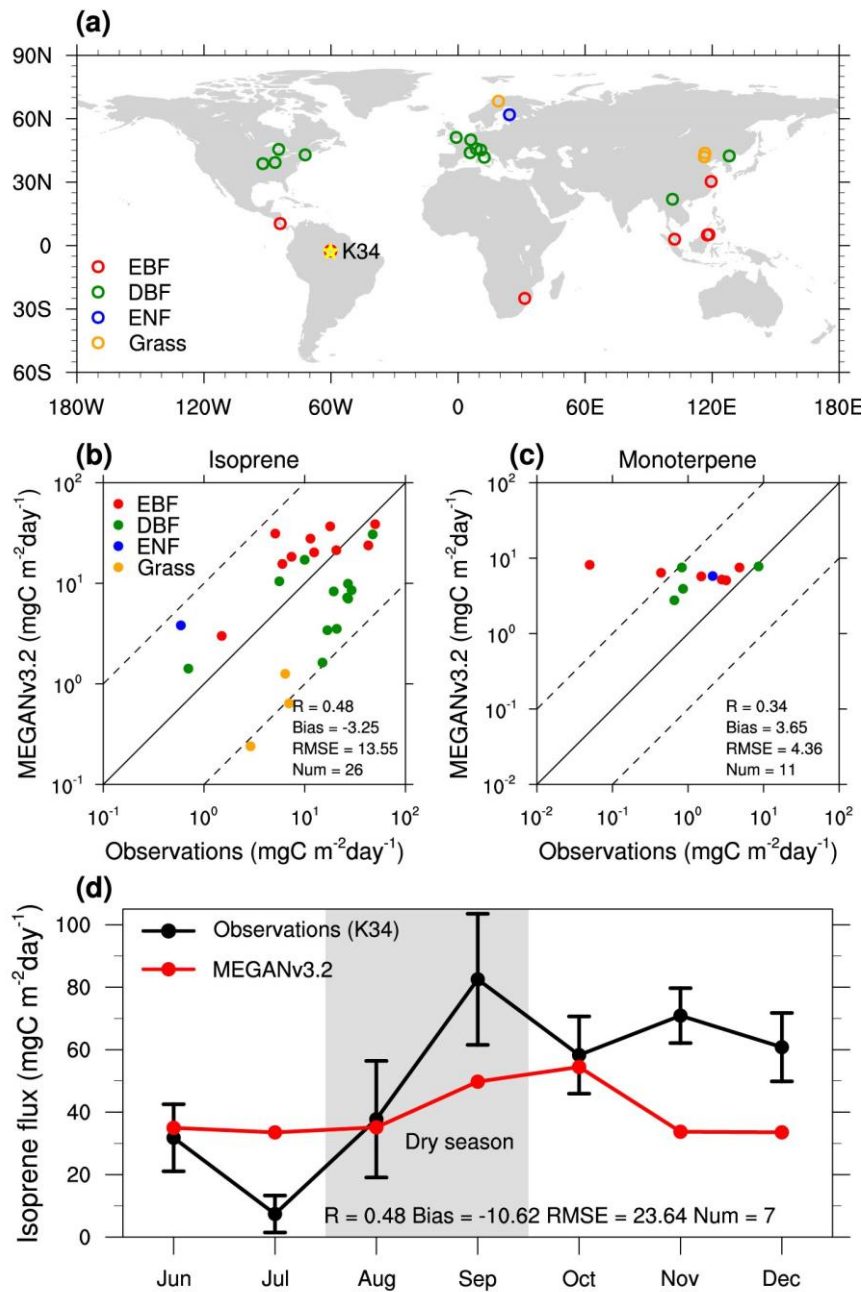
230 Figure 1: (a) The location distribution of isoprene and monoterpene observation sites based on the literature collection (the five- 235 pointed star represents the location of the K34 tower site, EBF: evergreen broadleaf forest, DBF: deciduous broadleaf forest, ENF: evergreen needleleaf forest, Grass: grassland), and comparison with simulated (b) isoprene fluxes, (c) monoterpene fluxes, and (d) monthly variations of isoprene fluxes measured at the K34 tower site in 2013 (the upper and lower limits of the observations represent one standard deviation). R: correlation coefficient, Bias: absolute bias, RMSE: Root mean square error, and Num: Total number of observation samples. In (b) and (c), the 1:1 (solid) and 1:10/10:1 (dashed) lines are plotted for references. In (d), gray shade denotes the dry season.
