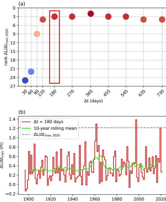
Figure 7. (a) Rank of the 2020 event in the 1897–2021 time series of annual block maxima of the rate of change in lake levels ( \Delta L/\Delta t ) based on the size of the time window ( \Delta t ). Red indicates a higher rank (more extreme), blue a lower rank (less extreme). The rank of the 2020 event with the chosen event definition ( \Delta t = 180 days) is highlighted by the red box. (b) Annual block maxima time series ( \Delta L/\Delta t ) max with \Delta t = 180 days for the period 1897–2021 and 10-year rolling mean of the time series.
