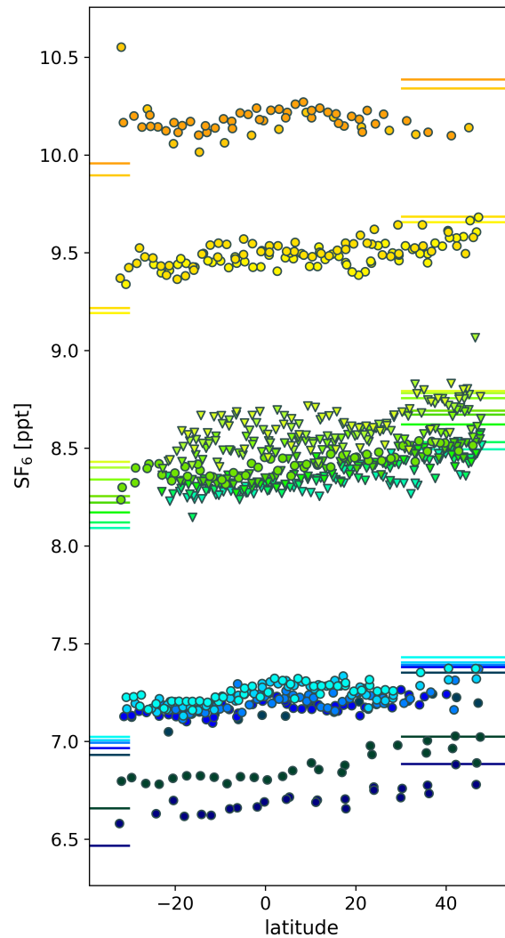
Figure 3. Latitudinal profiles of SF 6 mixing ratios measured in CARIBIC flask samples collected during flights with sections in the southern hemisphere including high SF 6 extreme values. Flights took place between May 2009 and March 2020, with flights between Germany and South Africa represented by circles and flights to South America by triangles. Horizontal lines denote surface mixing ratios for the extratropical latitudes outside \pm 30^\circ of each hemisphere. Different colours are used to group flights by year and month to guide the eye only, therefore a legend is omitted.
