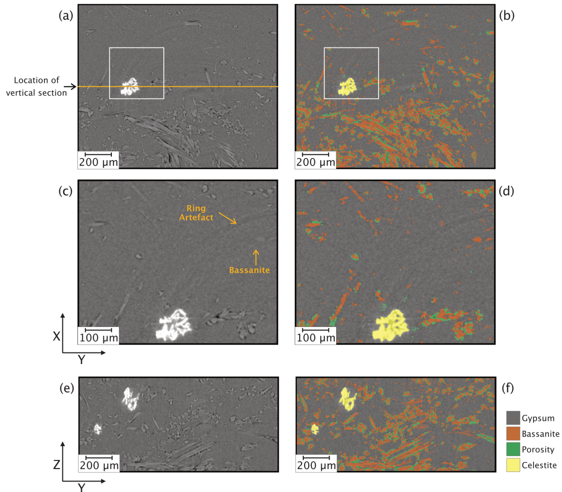
Figure 5. Horizontal (XY) and vertical (YZ) slices of the S - \mu CT images before (a, c, e) and after (b, d, f) deep learning segmentation performed using a model trained with Random Forest classified images. Images in (c) and (d) are closer captions of areas indicated with white boxes in (a) and (b).
