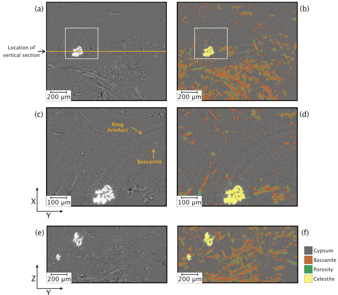
Figure 5. Horizontal (XY) and vertical (YZ) slices of the \mu\text{CT-S-}\mu\text{CT} images before (a, c, e) and after (b, d, f) deep learning segmentation performed using a model trained with Random Forest classified images. Images in (c) and (d) are closer captions of areas indicated with white boxes in (a) and (b).
