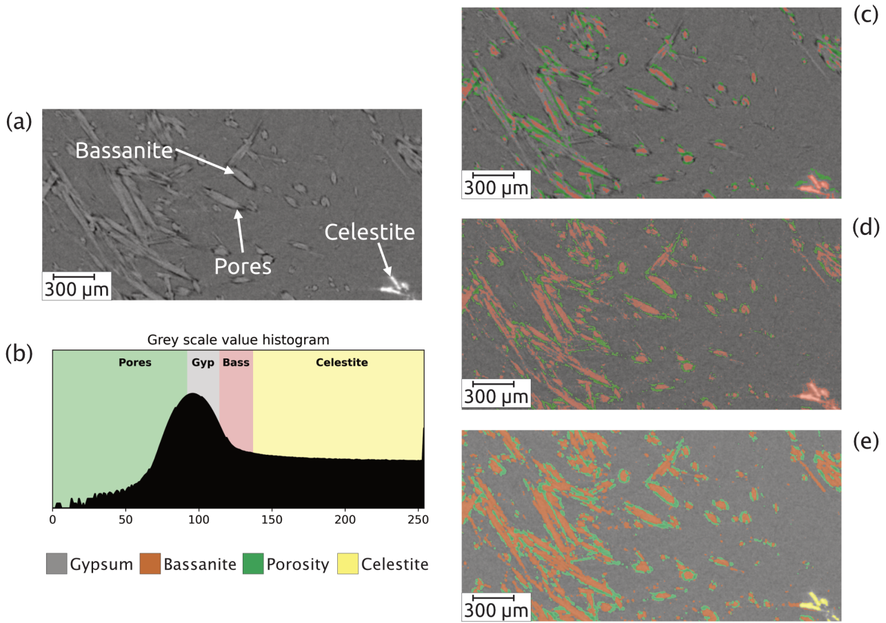
Figure 3. Challenges of the segmentation. (a) Portion of a horizontal cross-sectional slice of the raw \mu CT image showing the relative low contrast between gypsum and bassanite. (b) threshold values for the four phases present in the image. Two main phases – Gypsum and Bassanite – are difficult to split up accurately into two classes by the deep learning algorithm with (c) no data augmentation but are better segmented when using data augmentation (d) but still showing evident artefacts in the segmentation. Both cases (in c and d) struggle in separating the celestite phase which is wrongly classified as bassanite. (e) the segmentation results using Random Forest classifier as input into the deep learning algorithm.
