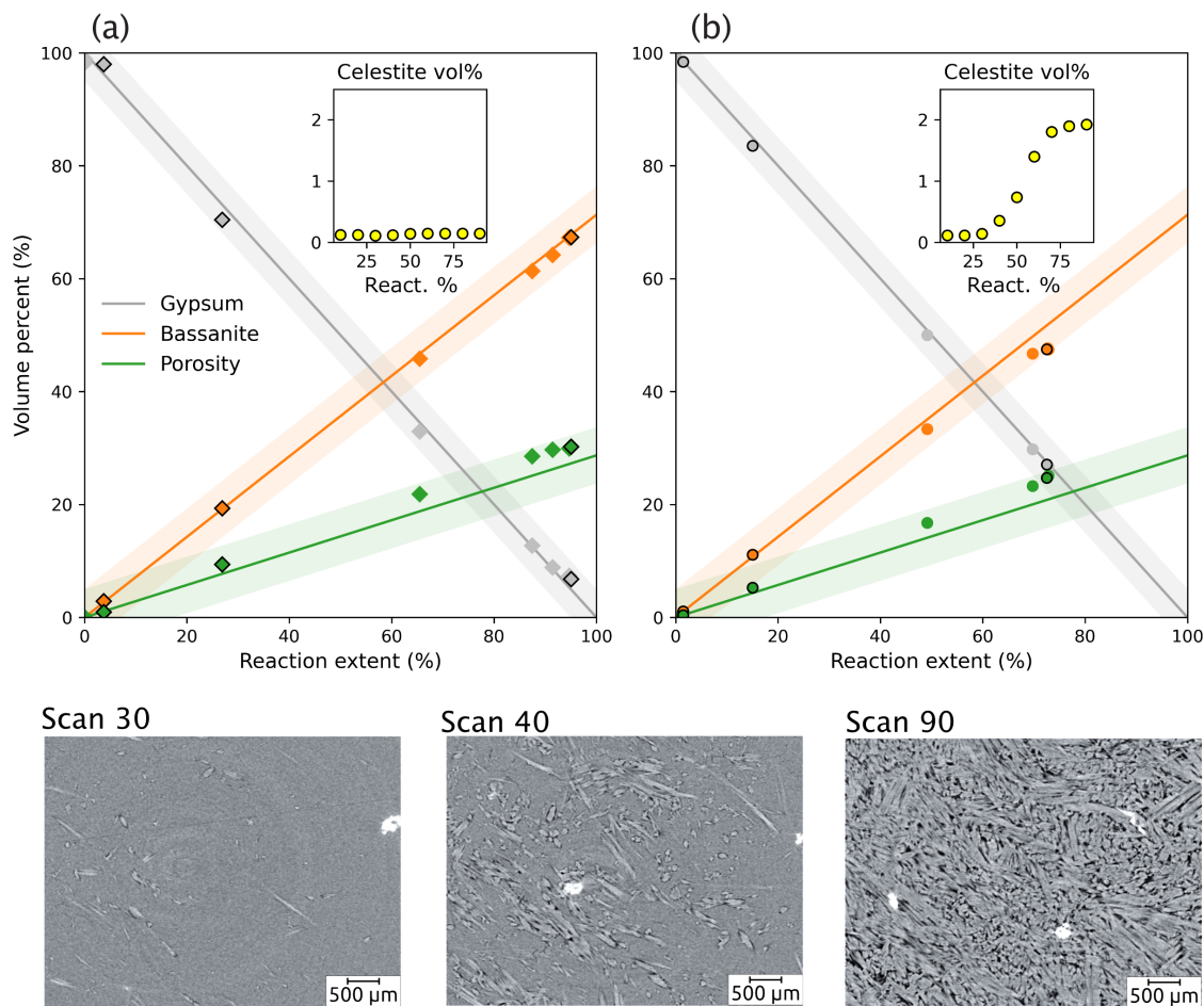
Figure 7. Quantitative analysis of phase volume changes during the gypsum dehydration experiment, as determined by segmenting the same volume-time-series data (sample VA19time-step-40) using two distinct segmentation methods. The new workflow developed in this study in (a) , which leverages a random forest classifier to label input data for a deep learning model, yields significantly improved accuracy in phase volume measurements relative to conventional histogram thresholding segmentation in (b) – including “despeckle” and “non-local means” with \sigma = 5 , smoothing = 1(b)-1 . The inset graphs show volume measurements for the celestite phase (yellow), which is a non-reacting phase during dehydration. The bottom images show slices of the sample at different stages; in the graph they are represented by the data points with a black outline
