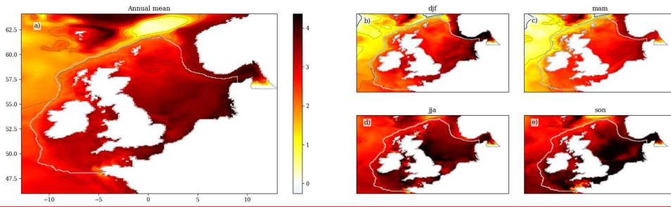
Figure 9 The SST ensemble mean change over the 21 st Century (2079-2098 compared to 2000-2019), for the: a) annual mean; b) winter (December to February (a, e, i)); c) spring (March to May (b, f, j)); d) summer (June to August (c, g, k); and e) autumn (September to November (d, h, l)). For each column and row, the main panel gives the ensemble mean (i), while the smaller panels on the left give the ensemble (j). Black contours relate to the colour bar ticks, and the zero contour is a thicker black line. The coast line and NWS region are delineated with a grey line, and Full comparison between the early and late century, and the components of variance (ensemble variance and interannual variability (upper (ii) and lower row (iii) respectively)), see Figure S17.
