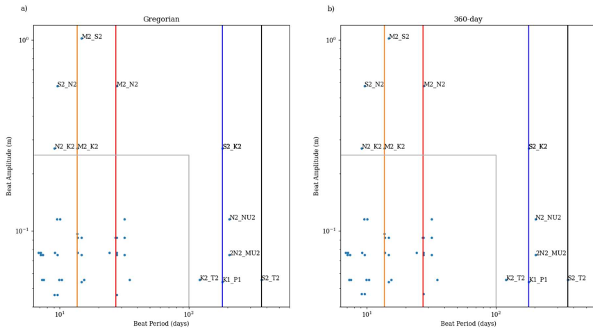
Figure A4B4 Beat frequency and amplitude for the standard Gregorian tidal constituent frequencies (left), and the modified 360-day frequencies under the Compress tidal scheme (right). The yellow and red lines show the monthly, and bimonthly frequencies, and the blue and black lines show the biennial and annual frequencies ( 2\pi/(365.24 \times 24) and 2\pi/(360 \times 24) respectively). The grey box shows the beat pairs with periods less than 100 days, and amplitudes less than 0.2m.
