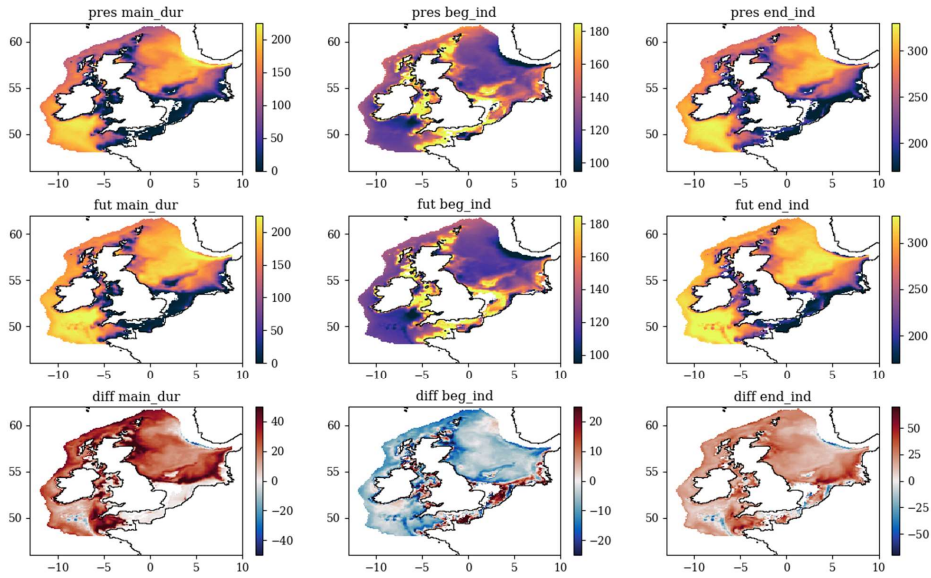
Figure 12 The ensemble mean duration, initialisation and break down of stratification, in day of year, (first, second and third column respectively) for the early- 21 st century (2000-2019, upper row) and late- 21 st century (2079-2098, middle row) DFT and their difference (bottom row). See Figure 6 for details, and how it changes between the two periods (first, second and third rows respectively).
