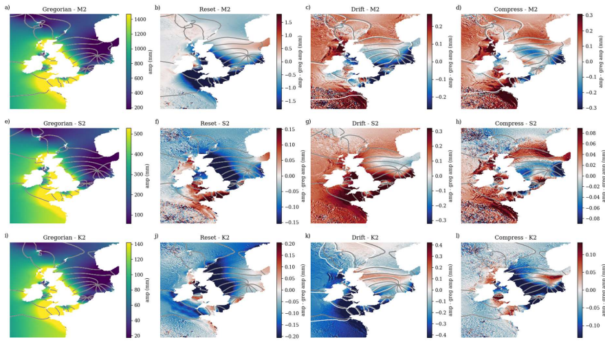
2400 | Figure A3B3 Cotidal charts for M 2 , S 2 and K 2 (upper, middle, and lower row respectively), for Gregorian (left column) and anomalies (relative to Gregorian) for Reset, Drift and Compress (second, third and fourth column respectively). The colours give the amplitude (or amplitude minus Gregorian amplitude anomaly) in mm, the contours give the co-phase lines (every 45 degrees), grey for Gregorian, and white for Reset, Drift and Compress respectively.
