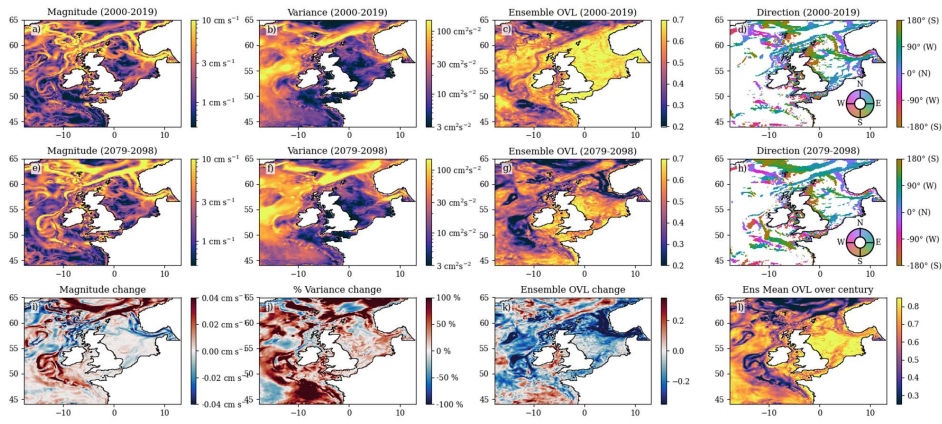
Figure 8 Barotropic residual current statistics. The early- 21st century (2000-2019, upper row, a-d) and, late- 21st century (2079-2098, middle row, e-h) SST and their difference (bottom row, i-l) of the ensemble mean current magnitude (a, e, i respectively), variance, as measured by the area of the 2.45 standard deviation current ellipse (b, f, j), the Ensemble OVL (the overlap of the ensemble, as a measure of how similar the ensemble members are (c, g, k) and the early and late 21st century current configuration (colours show the direction of the currents where the mean is more than 1 standard deviation). The four main columns give the seasons (ensemble mean of the OVL for each ensemble member when comparing early and late 21st century current distribution).
