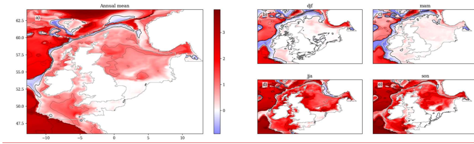
910 Figure 11 The surface-bed temperature difference (DFT) ensemble mean change over the 21 st Century (2079-2098 compared to 2000-2019), for the: a) annual mean; b) winter (December to February); c) spring (March to May); d) summer (June – August) and e) autumn (September – November). Black contours relate to the colour bar ticks, and the zero contour is a thicker black line. The coast line and NWS region are delineated with a grey line, and Full comparison between the early and late century, and the components of variance (ensemble variance and interannual variability), see Figure S19.
