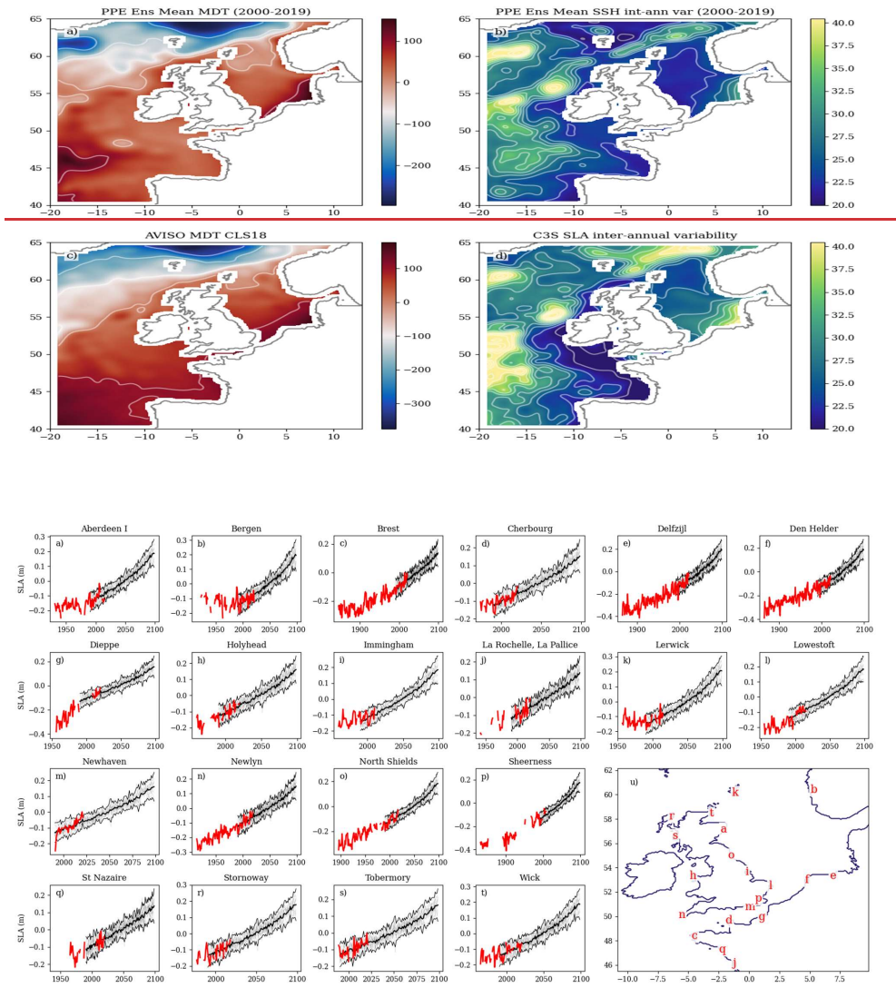
Figure 6 Tide gauge - model sea level anomaly comparison (metres). a-t) time-series of annual mean SSH from tide gauges (red), and the 12 ensemble members (grey), with the ensemble mean \pm 2 ensemble standard deviations shown in black. No account is taken of the differing benchmarks between the model and the tide gauges, so an arbitrary offset is added to align the two datasets to allow visual comparison of the trends and variability. Note the differing time tide gauge record length leads to different ranges on the x and y axes. u) Tide gauge locations are given in Table 3.
