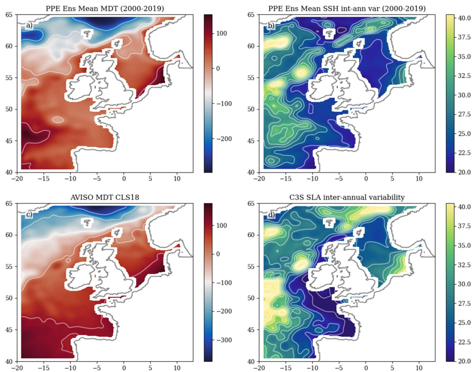
1840 Figure 5 Comparison of Modelled SSH with satellite altimetry (mm). a) Ensemble mean SSH anomaly (2000-2019) b) Ensemble interannual variability (standard deviations of annual mean SSH, averaged over the ensemble, 2000-2019), c) AVISO MDT (mean SSH), d) CS3 interannual variability of Sea Level Anomaly.
