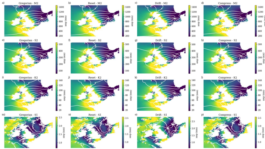
385 Figure A1B1 Cotidal charts for the M 2 (a-d), S 2 (e-h), K 2 (i-l) and S 1 (m-p) tidal constituents under the Gregorian (control, a, e, i, m), Reset (b, f, j, n), Drift (c, g, k, o) and Compress (d, h, l, p) tidal schemes. The colour maps represent the amplitude, and is constant for a given constituent, while the lines are lines of equal phase, (every 45°).
