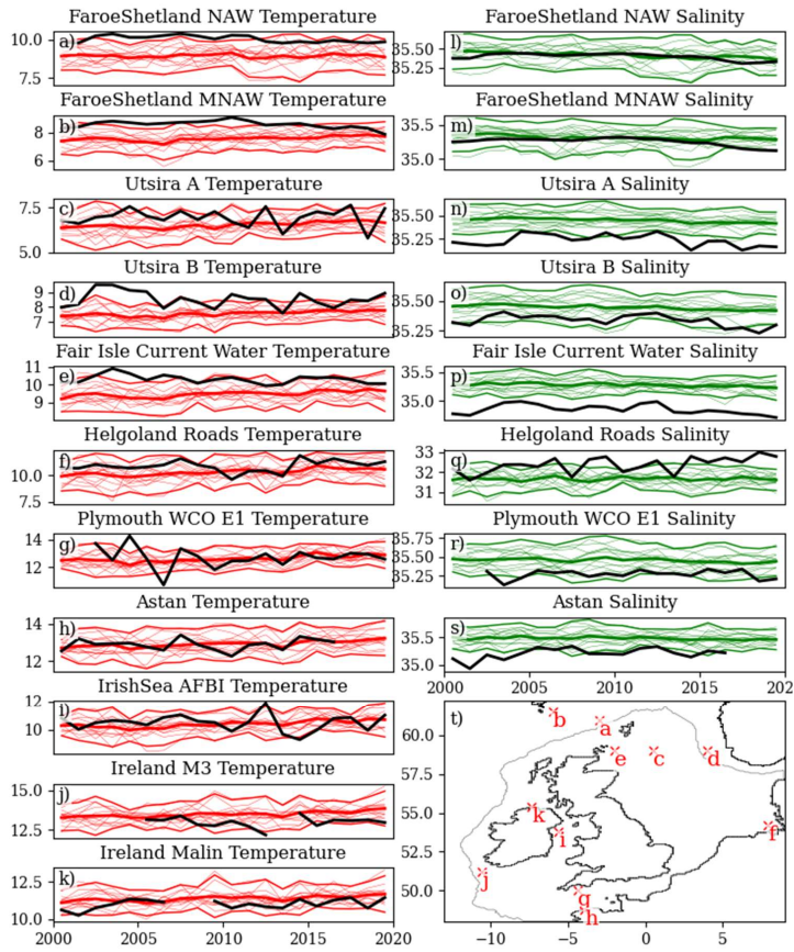
Figure 4 comparison of the NWSPEE with long annual mean timeseries of in situ T and S, from around the NWS (see text). The left column shows temperature, and the right shows salinity. i-k only measured temperature. These records are a mix of surface, near bed, water column mean and the mean of the upper water column.
