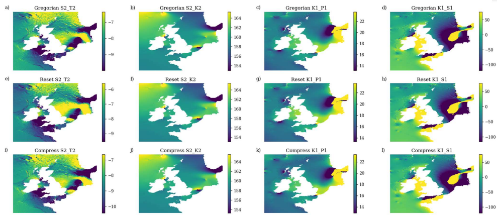
Figure A6B6 Timing of largest beat pair maximum (in day of year), for pairs that occurs at approximately the same time of each year. Note S 2 -K 2 are the beating pair with the greatest amplitude, \sigma_2 .
