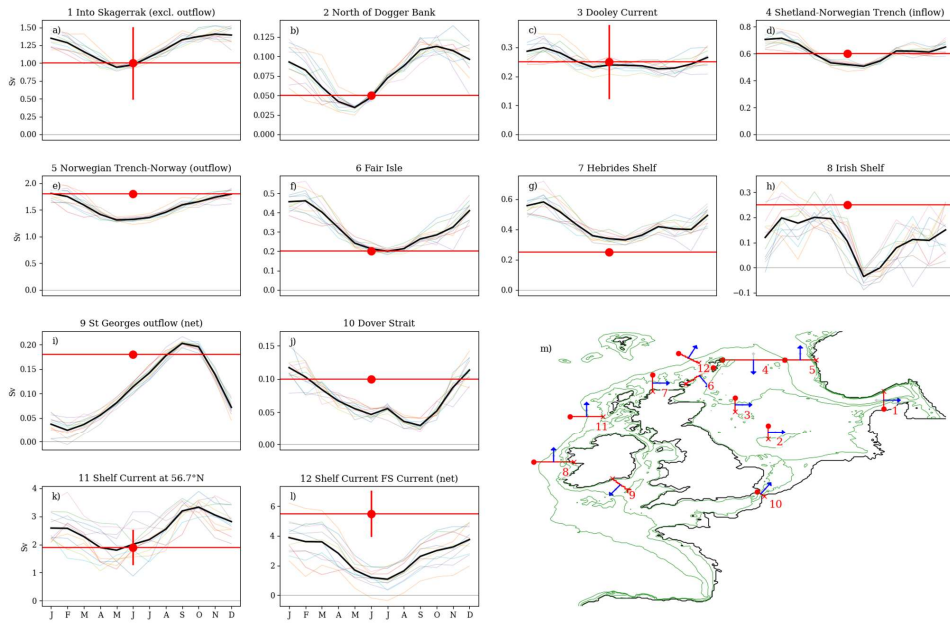
Figure 7 Comparison of modelled and observed volume transport through cross-sections. a-l: the NWPPE Ensemble mean (bold black) seasonal cycle (and ensemble members, coloured thin lines) compared to observed transport estimate (red circle, and horizontal line), and observation error estimate (vertical red line) where available. M) map of the NWS giving the location of the cross-sections. Table 4 gives the longitudes and latitudes of the ends of the cross-sections, and summarise the data.
