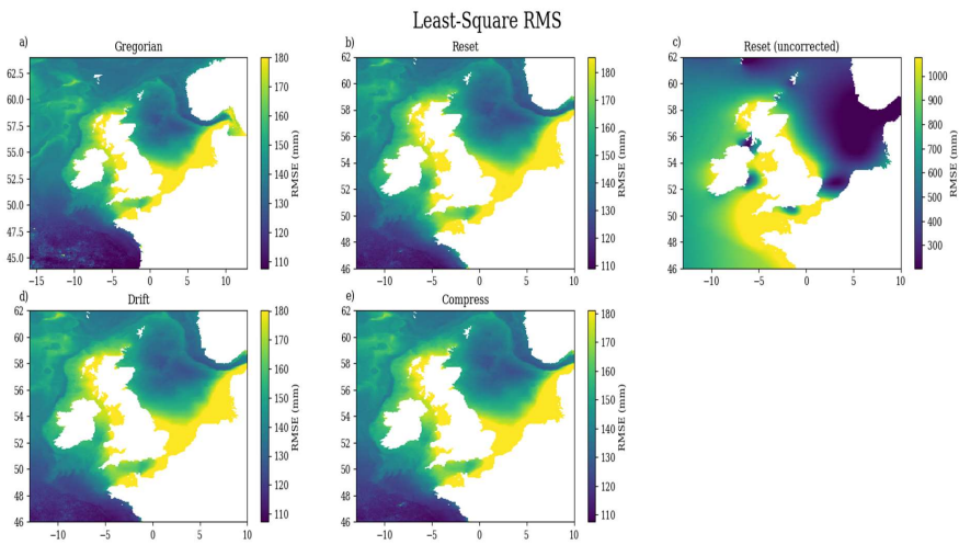
Figure A2B2 RMS of least square tidal fit, for the simulations: a) Gregorian; b) Reset; c) Reset (uncorrected); d) Drift; and e) Compress. For Reset, we construct an equivalent time (resetting to the Gregorian calendar at the beginning of each month) and use this for the least squares. We do not correct this in Reset (uncorrected), and the RMS errors are much greater (c).
