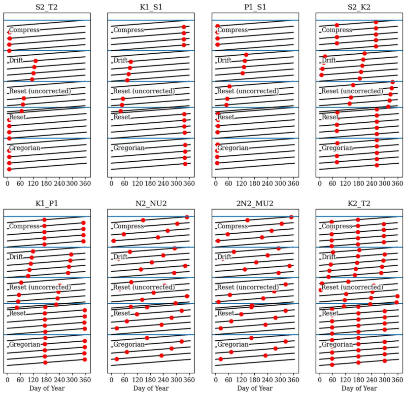
2415 | Figure ASB5 The timing (day of year) of the maximum of the beating tidal constituent pairs (with periods greater than 100 days) for the four different tidal systems for an example location. Each subplot is a beating tidal pair. The black line represents the day of the year (in the x direction) and the decimal year (in the y direction). The red dot is the local maximum of the beating pair. Each tidal system (Greg, Reset, Reset (uncorrected), Drift, and Compress) is stacked on top of one another.
