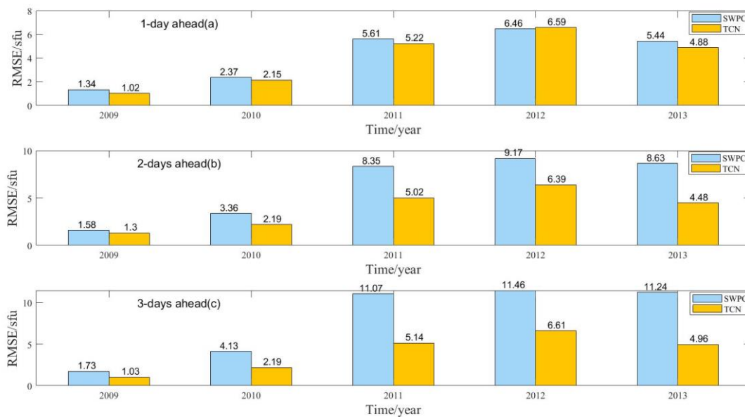
Figure 6: Comparison of the prediction performance between SWPC and TCN
