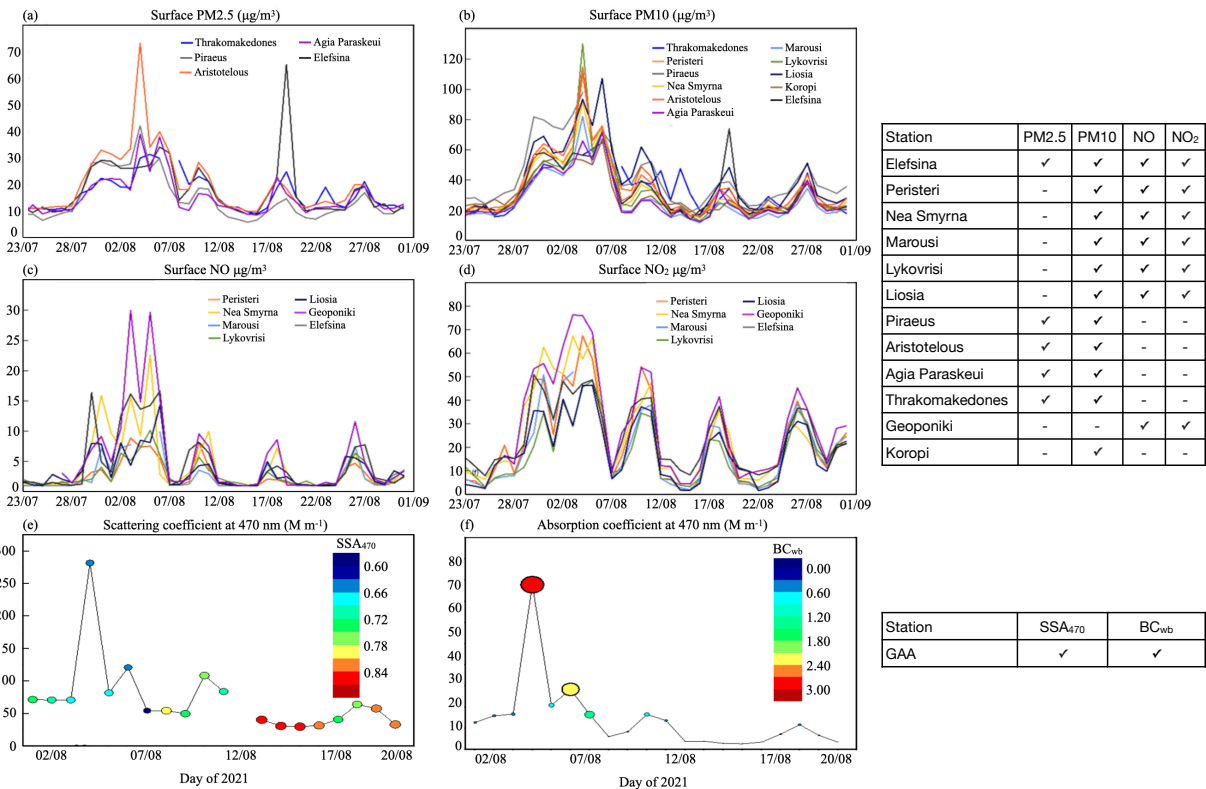
Figure 3. Variation of (a) PM 2.5 ( \mu\text{g m}^{-3} ), (b) PM 10 ( \mu\text{g m}^{-3} ), (c) NO ( \mu\text{g m}^{-3} ) and (d) NO 2 ( \mu\text{g m}^{-3} ) in Greater Athens Area (GAA) during August 2021. Temporal variation of the daily-mean values for the (e) scattering and (f) absorption coefficients in Athens during 1-20 August 2021. The data points in (e) and (f) are color-coded as a function of SSA 470 and BC wb concentration, respectively.
