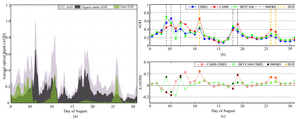
Figure 6. (a) Total, organic matter and dust AOD from CAMS at 550 nm. (b) Comparison of AOD from CIMEL with AODs from CAMS and SKYCAM at 500 nm (see text). (c) AOD differences between CAMS and CIMEL, and between SKYCAM and CIMEL at 500 nm.
