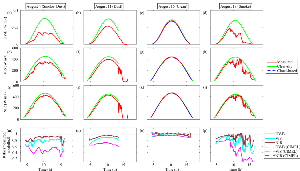
Figure 10. Effect of aerosols on UV-B (a, b, c, d), VIS (e, f, g, h) and NIR (i, j, k, l) irradiances on August 4, August 11, August 16 and August 18, respectively and the ratio between measured and modelled irradiances (m, n, o, p).
