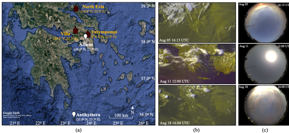
Figure 1. (a) Map for the wildfire source sites (in red) and the study region (in white). Base map credits: ©2022 Google Earth. Identification of the event on August 5, 11 and 18 using (b) Meteosat Second Generation (MSG) and (c) sky-camera images
