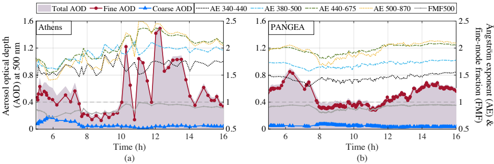
Figure 8. Variation of total, fine- mode and coarse- mode AOD at 500 nm, and Ångström exponents in (a) Athens (AERONET Level 1.0) and (b) PANGEA (AERONET Level 2.0) during the wildfire event of August 7, 2021.
