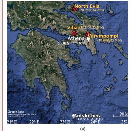
Figure 1. (a) Map for the wildfire source sites (in red) and the study region (in white). Base map credits: ©2022 Google Earth. Identification of the event on August 5, 11 and 18 using (b) Meteosat Second Generation (MSG) and (c) sky-camera images
