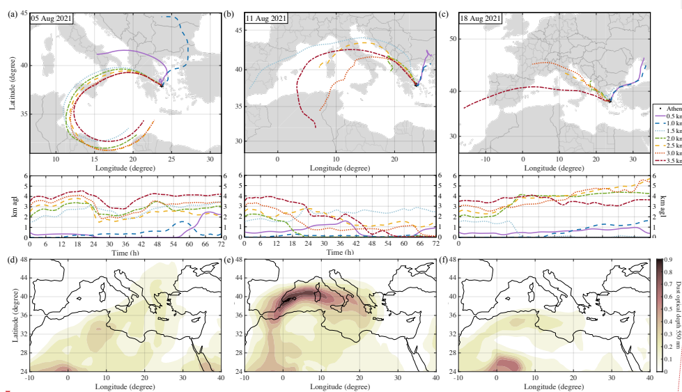
Figure. 2. Identification of dust transfer to Athens using HYSPLIT back trajectories ending at 12:00 UTC (a, b, c) and Copernicus Atmospheric Monitoring Service (CAMS) reanalysis time-averaged dust optical thickness over 00–21 UTC (d, e, f).
