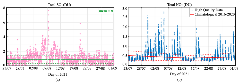
Figure A3. Variation of (a) total \text{SO}_2 (DU) from Brewer measurements and (b) total \text{NO}_2 (DU) from Pandora measurements at Athens during August 2021.
