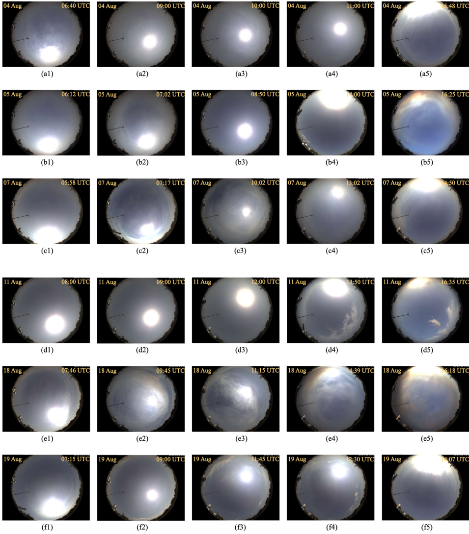
Figure A1. Sky-camera images for Athens (a1–a5), (b1–b5), (c1–c5), (d1–d5), (e1–e5) and (f1–f5) for August 4, 5, 7, 11, 18 and 19, respectively.
