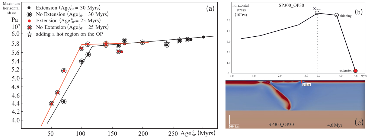
Figure 11. (a) Maximum vertically averaged horizontal stress ( \sigma_{hmax} ) over OP thickness (from the surface to the OP bottom, 50 km depth when the Age OP 0 is 30 Myrs and 45 km depth when the Age OP 0 is 25 Myrs which was defined by the temperature contour of 1300K.) vs. Age SP 0 . The stars mark the models which have a hot region on the OP. (b) Depicts the time evolution of vertically averaged horizontal stress ( \sigma_h ) and (c) identifies the specific location (in the viscosity field) where the stress in panel (b) is calculated. (b) and (c) are both from model SP300_OP30. A positive stress value means extensional.
