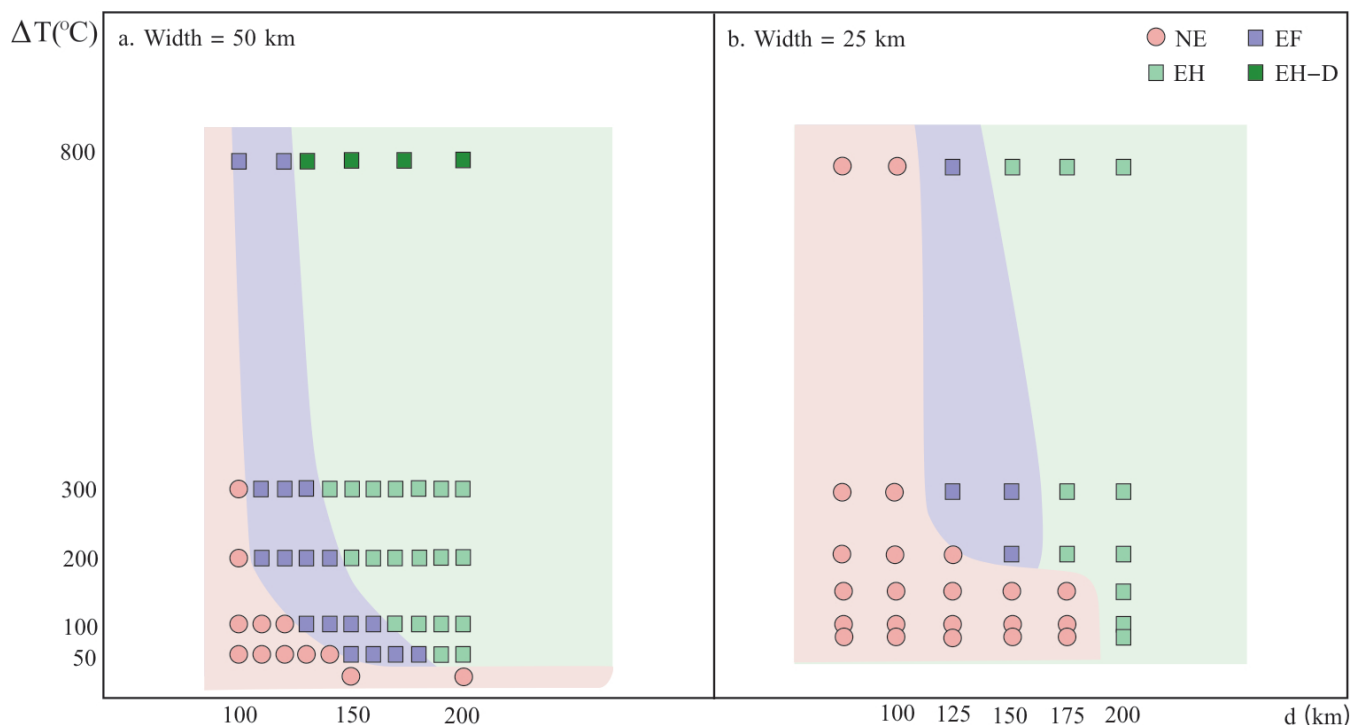
Figure 7. (a) Regime diagram of distance vs. \Delta T when the width is 50 km and (b) the comparison to the results when the width is 25 km.
