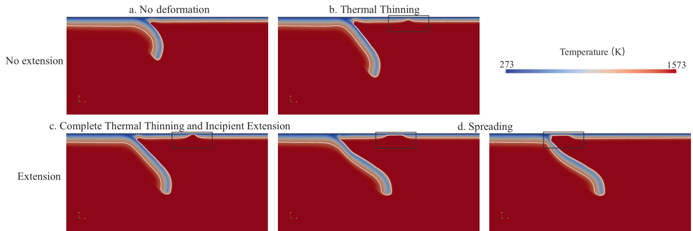
Figure 3. Defination-Definition of the extension levels by the isothermal contour of 1300 K (the white line). The temperature fields show (a) No deformation, (b) Thermal Thinning , (c) Complete thinning-Thermal Thinning and Incipient Extension and (d) Spreading (far-field spreading on the left and hot-region spreading on the right). (a) and (b) are classified as 'No Extension', whereas (c) and (d) are classified as 'Extension'.
