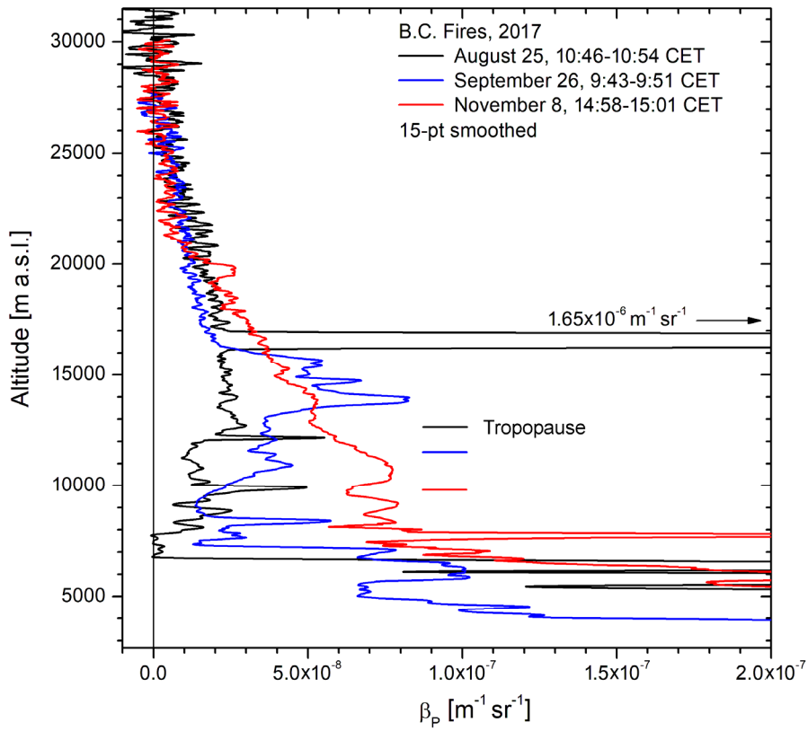
195 | Fig. 4. Three examples of 532-nm backscatter coefficients following the British Columbia (B.C.) fires in 2017; the data are slightly smoothed (sliding arithmetic average over \pm 7 bins) because of elevated noise due to analogue data acquisition, daytime conditions and just 20000 laser shots. The corrected Munich tropopause altitudes of from the Munich radiosonde are marked in the colours of the corresponding backscatter coefficients.
