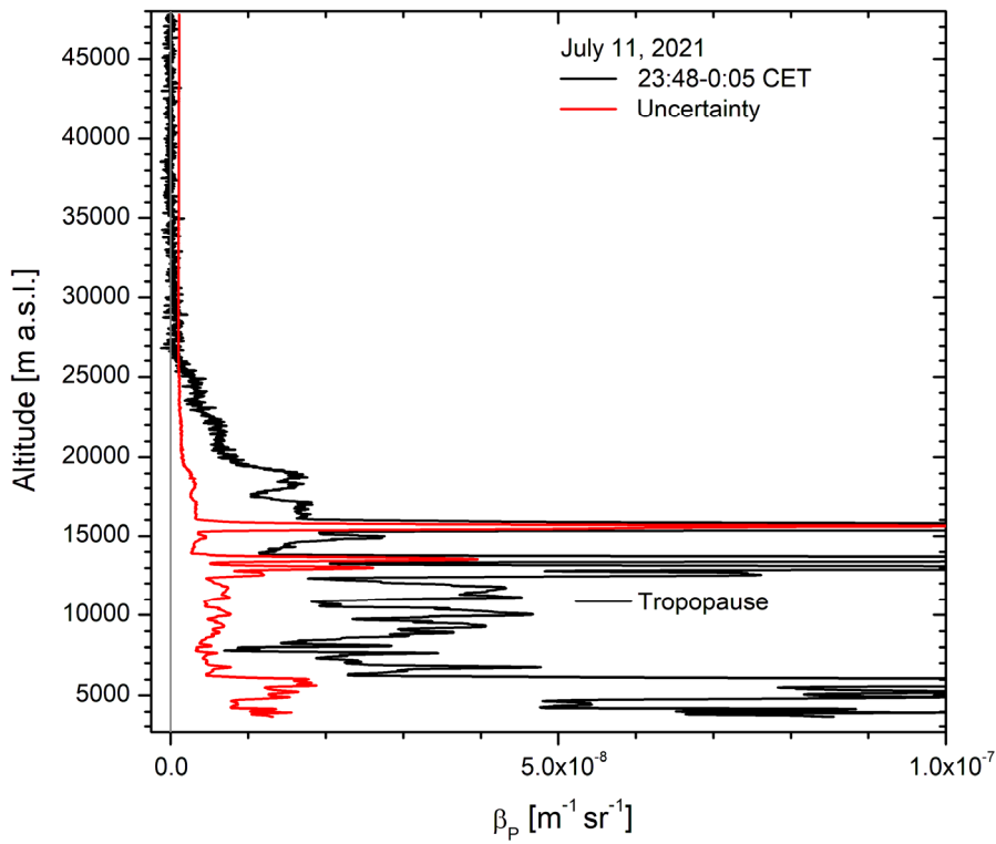
1215 Fig. 8. 532-nm aerosol backscatter coefficients on 11 July 2021; the two maximum values are 2.63 \times 10^{-7} \text{ m}^{-1} \text{ sr}^{-1} at 13.5 km and 7.07 \times 10^{-7} at 15.6 km. The relative uncertainty at 15.6 km is estimate as 18 %.
