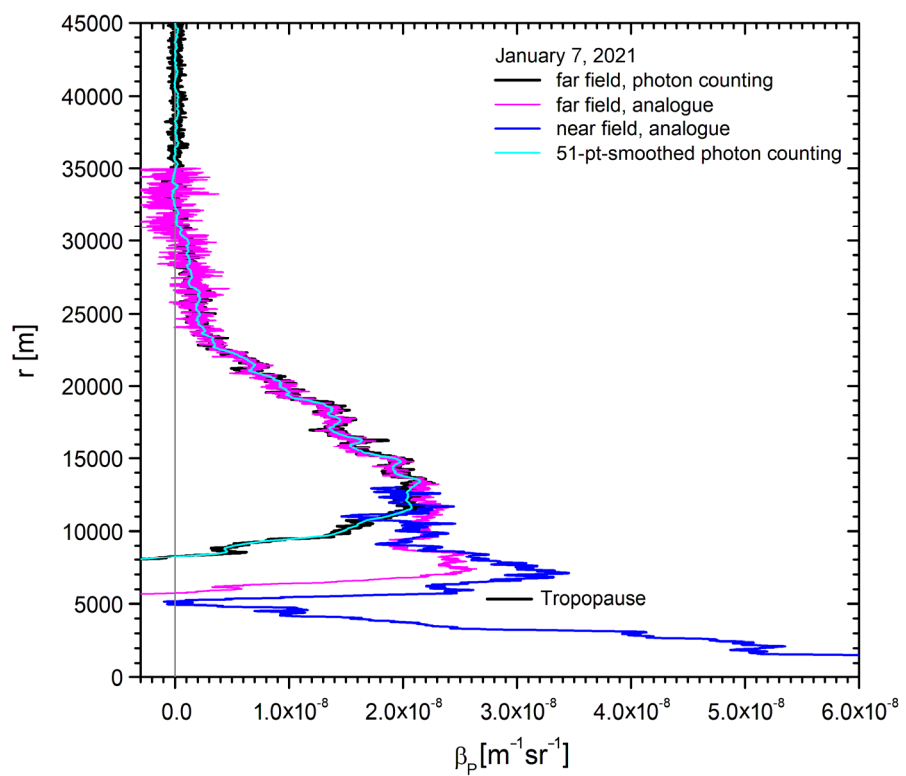
Fig. 1. Backscatter coefficients from the Klett inversions of the data of the near- and far field detection channels in the evening of 7 January 2021 (100000 laser shots); the values are displayed with bin sizes of 7.5 m (old system: 75 m, same noise amplitude up to 40 km). The photon-counting values are smoothed with a \pm 25 -bin sliding average that reveals the high far-field performance of the system. Please, note the low wintertime Munich tropopause at r = 5.3 km ( h = 8.0 km). r = 0 m corresponds to 2675 m a.s.l. (laboratory at UFS). The aerosol below 5 km was advected from Ukraine and Turkey.
