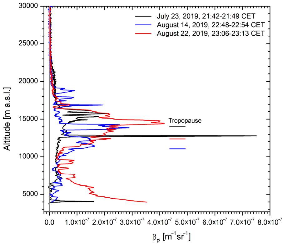
1225 Fig. 10. High 532-nm aerosol backscatter coefficients following the Raikoke volcanic eruption in June 2019; the tropopause levels are 13.89 km, 11.06 km and 12.40 km, respectively. We tend to assume that the spike at 12.8 km on 23 July was caused by a cirrus cloud because it is located below the tropopause. However, the Munich relative humidity at that altitude was less than 30 %. The tropopause altitudes are marked in the colours of the respective backscatter coefficients.
