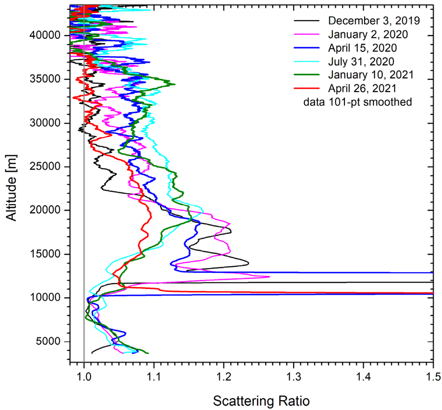
1230 Fig. 11. 532-nm scattering ratios smoothed by gliding \pm 50 -bin averages for selected measurements in 2019, 2020 and 2021; starting in January 2021 the aerosol layer expanded to more than 28 km a.s.l., possibly caused by northward propagation of the plume from the tropical eruption of Ulawun in the Brewer-Dobson circulation. The uncertainty of the values strongly grows above 35 km because the relative noise in the data starts to exceed the size of the aerosol features.
