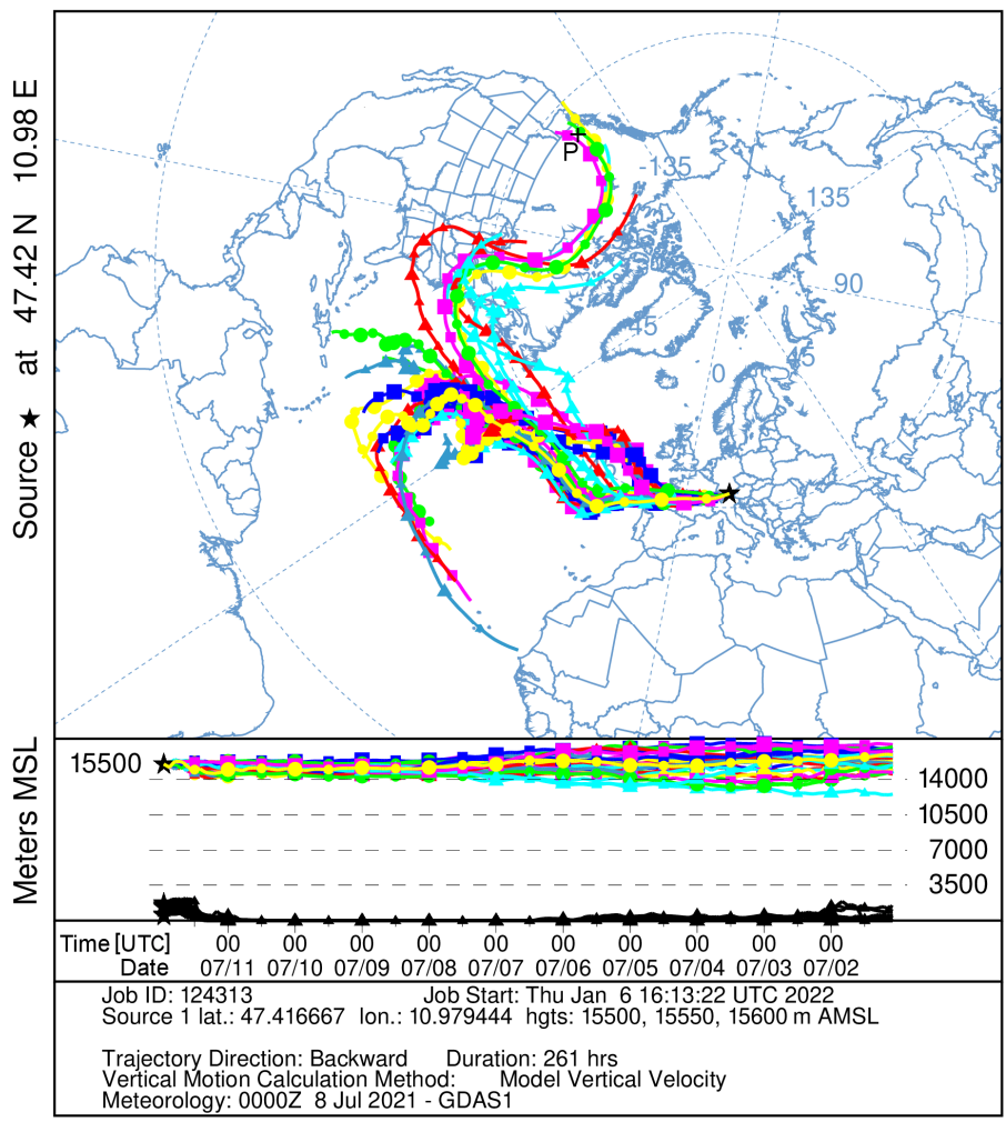
Fig. 9. HYSPLIT ensemble backward trajectories initiated at 15.55 km ± 0.05 km a.s.l. above UFS (Garmisch-Partenkirchen) on 11 July 2021 (23 UTC); the duration of the trajectories is 261 h (see text); the most likely pyro-Cb position at 51.0° N and 120.8° W is marked with a black cross (labelled with P).
