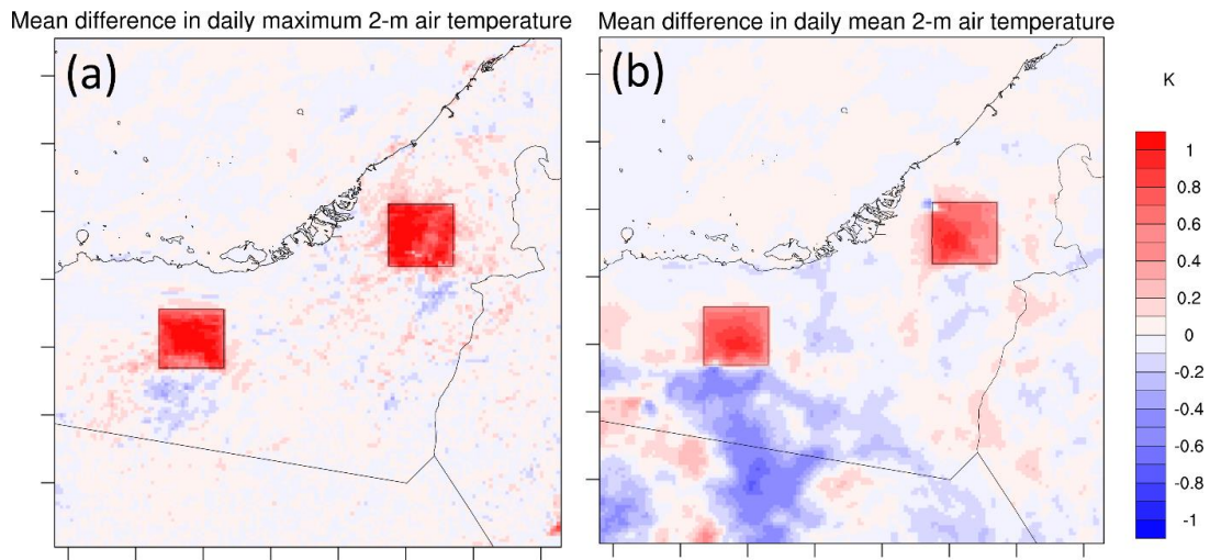
Figure X: The case-average impact on daily mean and daily maximum 2-m air temperatures from the 50km ABS. Computed respectively, as \frac{1}{n} \sum_1^n (\overline{T2m_{ABS_{50km}}} - \overline{T2m_{Control}}) and \frac{1}{n} \sum_1^n (\overline{T2m_{max_{ABS_{50km}}} - T2m_{max_{Control}}) , where n is the number of cases. Panel (a) is the daily maximum 2-m temperature impact, and Panel (b) 24-hour daily mean impact.
