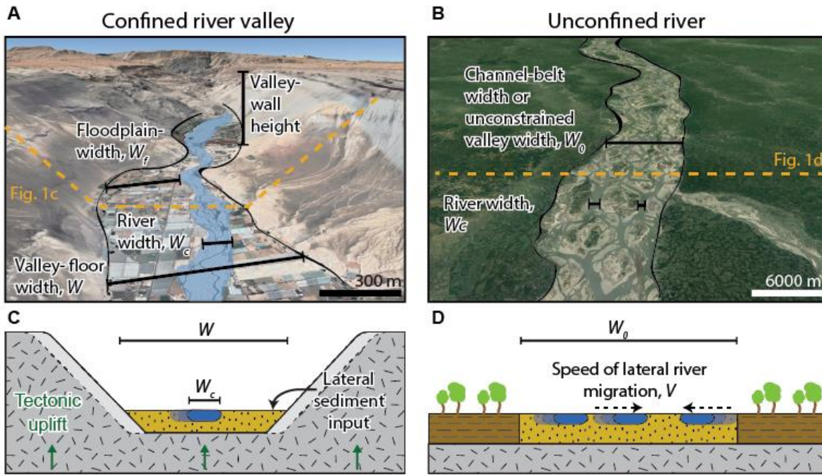
130 Fig. 1: Examples and concepts for confined river valleys and unconfined rivers. (A) Oblique view from © Google Earth of the San Jose River, Chile (18.58°S, 69.97°W), showing a confined valley. Debris cones on the valley flanks are signs for substantial sediment input from valley walls into the river valley. The scalebars refer to the foreground. (B) Oblique view from © Google Earth of the Brahmaputra river, Bangladesh (25.3°N, 89.7°E), that is laterally unconfined. (C) Conceptual sketch of the dynamics in a confined river valley. (D) Conceptual sketch for the dynamics in an unconfined channel belt.
