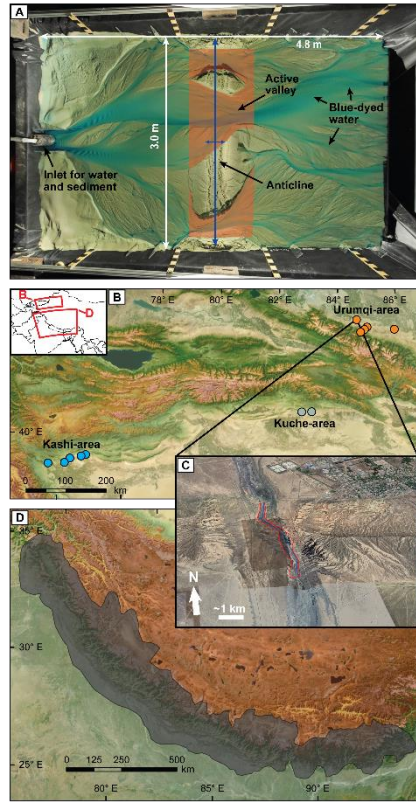
270 Fig. 3: Overview of the datasets used for model testing. (A) Overhead picture from an analogue experiment of braided rivers that cross an active uplift. The red shaded area marks the area of the uplift eroded by streams that is divided by the length of the area in the downstream direction to obtain a characteristic width. Where the stream splits, the entire valley area is summed. Figure adapted from Bufe et al. (2016a). (B) Locations of folds in the foreland of the Tian Shan for which we assembled uplift rates from the literature and mapped valley widths on Google Earth. Basemap sourced from Esri and hillshade created from an SRTM digital elevation model. (C) Oblique © Google Earth View of the Dushanzi anticline (location in B) and the mapped area (red) and stream length (blue) across the valley. (D) Overview of the Himalaya and the area covered by the width dataset of Clubb et al. (2023b). Basemap sourced from Esri and hillshade created from an SRTM digital elevation model. 275
