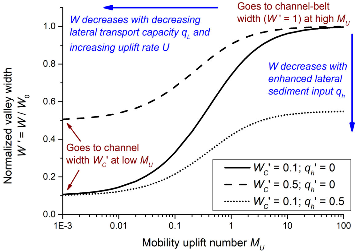
365 Fig. 4: Evolution of dimensionless valley width as function of the mobility-uplift number M_U , predicted by eq. (16). An increase in M_U corresponds either to an increase in lateral transport capacity, q_L , or a decrease in uplift rate U . A change in the relative channel width W_C' affects the left-hand limit (solid and dashed lines), while a change in the relative hillslope supply q_h' affects the right-hand limit (solid and dotted lines).
