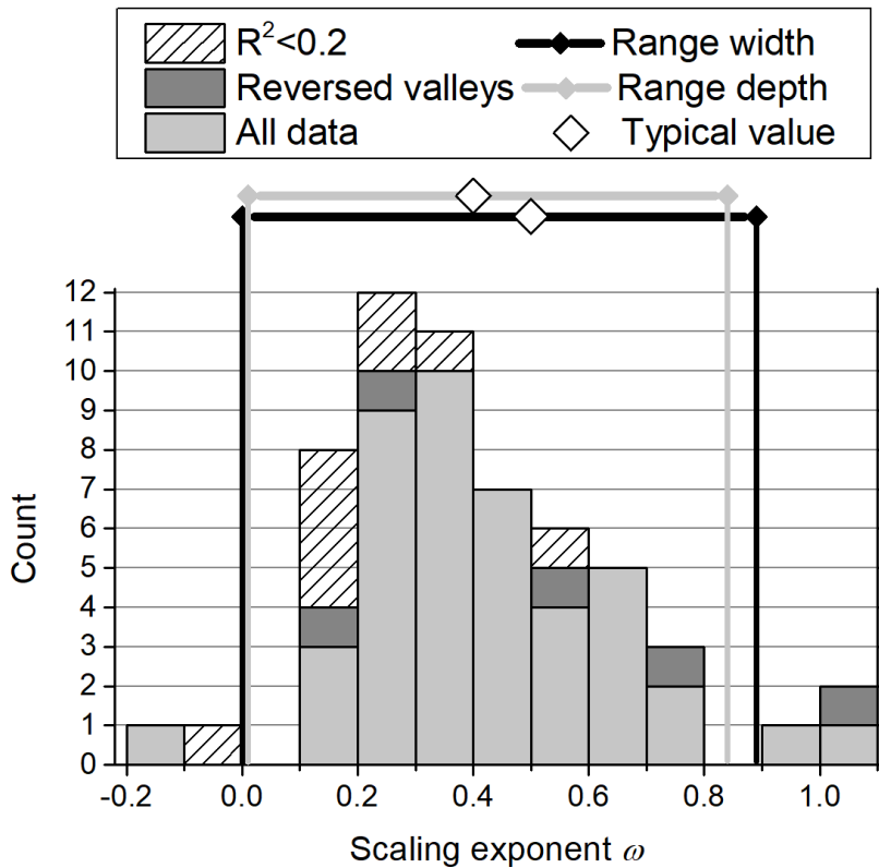
455 Fig. 6: Histogram of 57 valley width to drainage area scaling exponents \omega (eq. 21), compiled from the literature (Table 4). Light grey blocks give all data from regular valleys with a correlation coefficient R^2 between valley width and drainage area exceeding 0.2, striped blocks give data with R^2 < 0.2 , and dark grey blocks correspond to reversed valleys reported by Harel et al. (2022), where tilting reversed the flow direction of the river. The range of scaling exponent values for flow depth (grey; 0.01-0.84) and channel width (black; 0-0.89) reported by Park (1977) and Rhodes (1978) are also indicated (cf. eq. 8).
