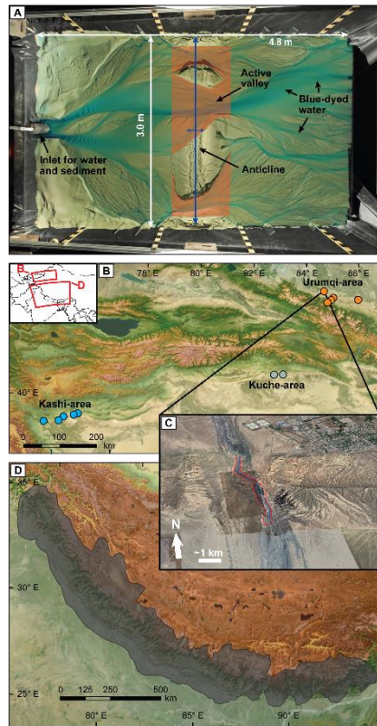
280 Fig. 3: Overview of the datasets used for model testing. (A) Overhead picture from an analogue experiment of braided rivers that cross an active uplift. The red shaded area marks the area of the uplift eroded by streams that is divided by the length of the area in the downstream direction to obtain a characteristic width. Where the stream splits, the entire valley area is summed. Figure adapted from Bufe et al. (2016a). (B) Locations of folds in the foreland of the Tian Shan for which we assembled uplift rates from the literature and mapped valley widths on Google Earth. Basemap sourced from Esri and hillshade created from an SRTM digital elevation model. (C) Oblique © Google Earth View of the Dushanzi anticline (location in B) and the mapped area (red) and stream length 285 (blue) across the valley. (D) Overview of the Himalaya and the area covered by the width dataset of Clubb et al. (2023b). Basemap sourced from Esri and hillshade created from an SRTM digital elevation model.
