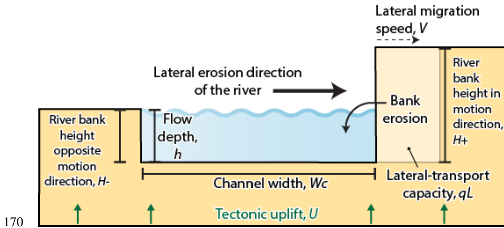
170 Fig. 2: Schematic cross section of a migrating channel, with definition of parameters.
