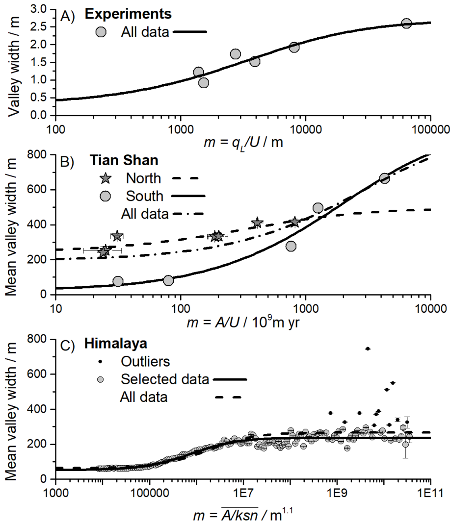
405 Fig. 5: Valley width as a function of the proxy m for the ratio of lateral transport capacity and uplift. Lines give fits according to eq. (17); all fit parameters are listed in Table 3. (A) Data from the analogue experiments by Bufe et al. (2016a). Mean valley width is calculated from the bevelled area of the fold divided by the length of the uplifted area of 0.5 m (Table 1). The proxy for the ratio of lateral transport capacity, q_L and uplift rate U is given in eq. (18). (B) Valley width in the Tian Shan (Table 2) as a function of the ratio of drainage area, used as a proxy for q_L , and uplift rate (eq. 19). Values for the north (dark stars, dashed line) and south (grey dots, solid line) are treated separately. The dash-dotted line shows a fit to all data. (C) Mean valley width shown as a function of the ratio of drainage area A and the steepness index k_{sn} , with the latter assumed to linearly scale with uplift rate (eq. 20). Error bars show the standard error of the mean for all values within a bin. We assumed that values of k_{sn} < 1 are unrealistic. If all remaining data points are included, the fit yields R^2 = 0.63 (dashed line). However, assuming that valleys with a mean width above 300 m are dominantly formed by processes other than fluvial beveling, some of the data points can be treated as outliers (black circles). The remaining data points yield R^2 = 0.91 (grey circles, solid line). Note that the inferred channel widths W_c are likely affected by 30-m resolution of the digital elevation model that underlies the dataset. 410 415
