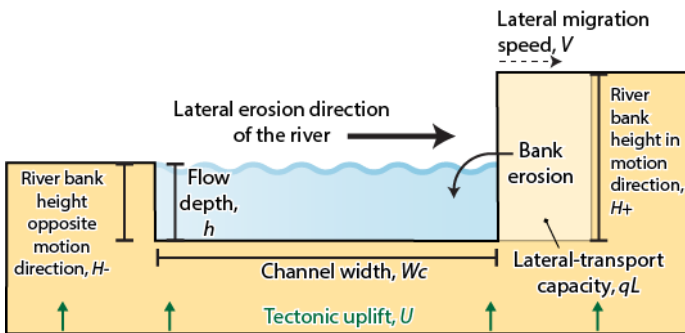
Fig. 2: Schematic cross section of a migrating channel, with definition of parameters.
