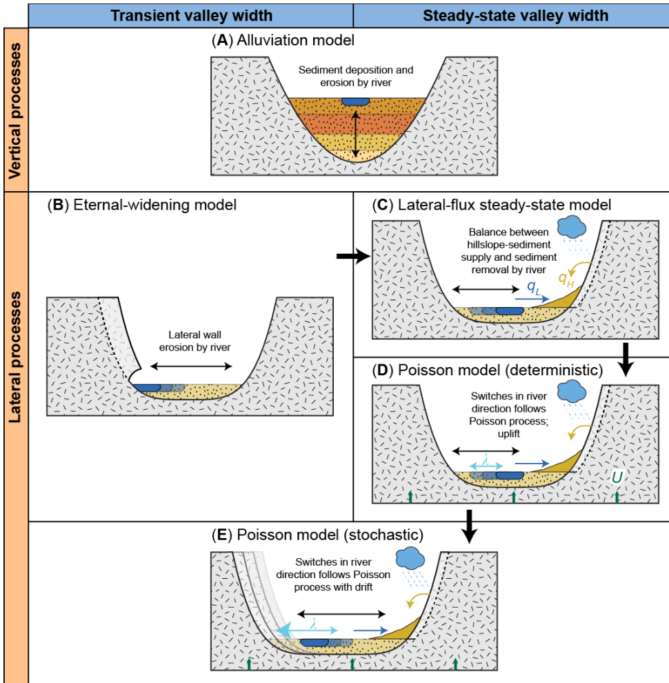
610 Figure 7: Overview of the existing models, organised into groups according on whether they emphasize vertical or lateral processes (vertical axis), and whether they yield a transient or steady state valley width (horizontal axis). See text for model descriptions.
