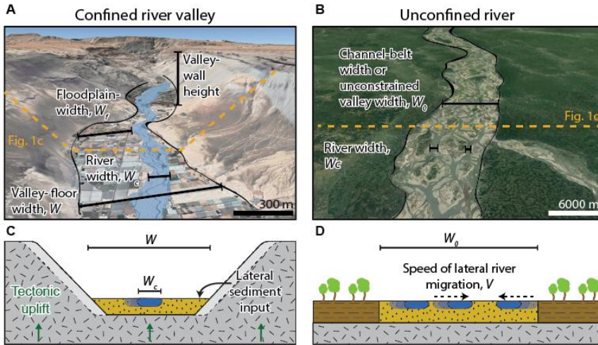
135 Fig. 1: Examples and concepts for confined river valleys and unconfined rivers. (A) Oblique view from © Google Earth of the San Jose River, Chile (18.58°S, 69.97°W), showing a confined valley. Debris cones on the valley flanks are signs for substantial sediment input from valley walls into the river valley. The scalebars refer to the foreground. (B) Oblique view from © Google Earth of the Brahmaputra river, Bangladesh (25.3°N, 89.7°E), that is laterally unconfined. (C) Conceptual sketch of the dynamics in a confined river valley. (D) Conceptual sketch for the dynamics in an unconfined channel belt.
