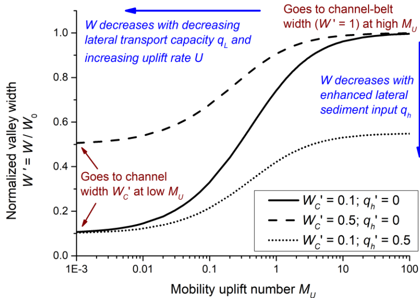
Fig. 4: Evolution of dimensionless valley width as function of the mobility-uplift number M_U , predicted by eq. (16). An increase in M_U corresponds either to an increase in lateral transport capacity, q_L , or a decrease in uplift rate U . A change in the relative channel width W'_C affects the left-hand limit (solid, and dashed and dash-dotted-lines), while a change in the relative hillslope supply q'_h affects the right-hand limit (solid and dotted lines).
