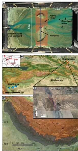
275 Fig. 3: Overview of the datasets used for model testing. (A) Overhead picture from an analogue experiment of braided rivers that cross an active uplift. The red shaded area marks the area of the uplift eroded by streams that is divided by the length of the area in the downstream direction to obtain a characteristic width. Where the stream splits, the entire valley area is summed. Figure adapted from Bufe et al. (2016a). (B) Locations of folds in the foreland of the Tian Shan for which we assembled uplift rates from the literature and mapped valley widths on Google Earth. Basemap sourced from Esri and hillshade created from an SRTM digital elevation
