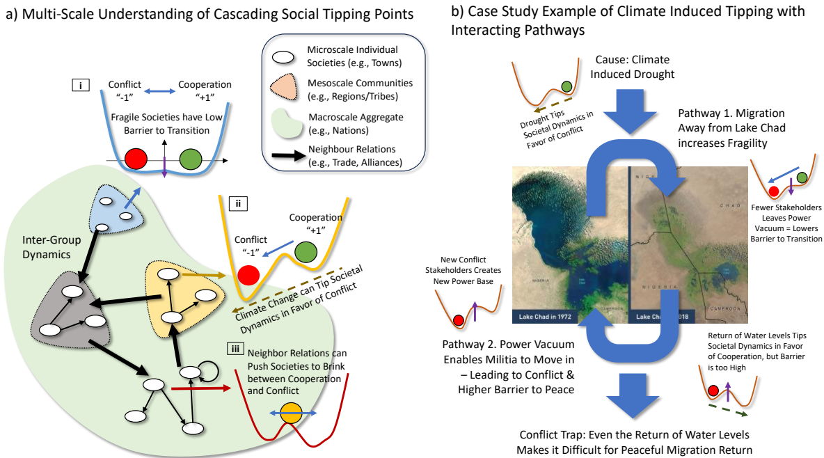
Figure 6 (a) Multi-scale understanding of cascading transitions between conflict and cooperation/peace, and (b) Example case study in Lake Chad region of climate induced tipping points with interacting pathways.
