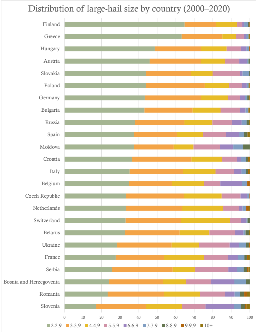
424 Figure 15. Horizontal bar charts of the size distribution of large hail for countries with 100 or more 425 reports (%): 2000–2020.
