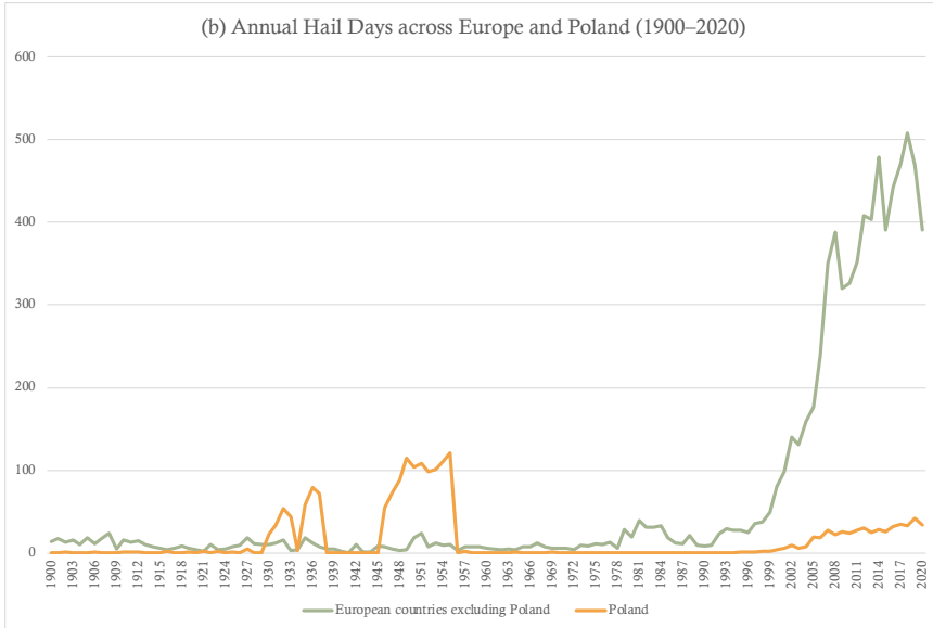
Figure 16. Time series of annual numbers of (a) large-hail reports for Europe (green line) and Poland (red line), and (b) large-hail days for Europe (green line) and Poland (red line): 1900–2020.
