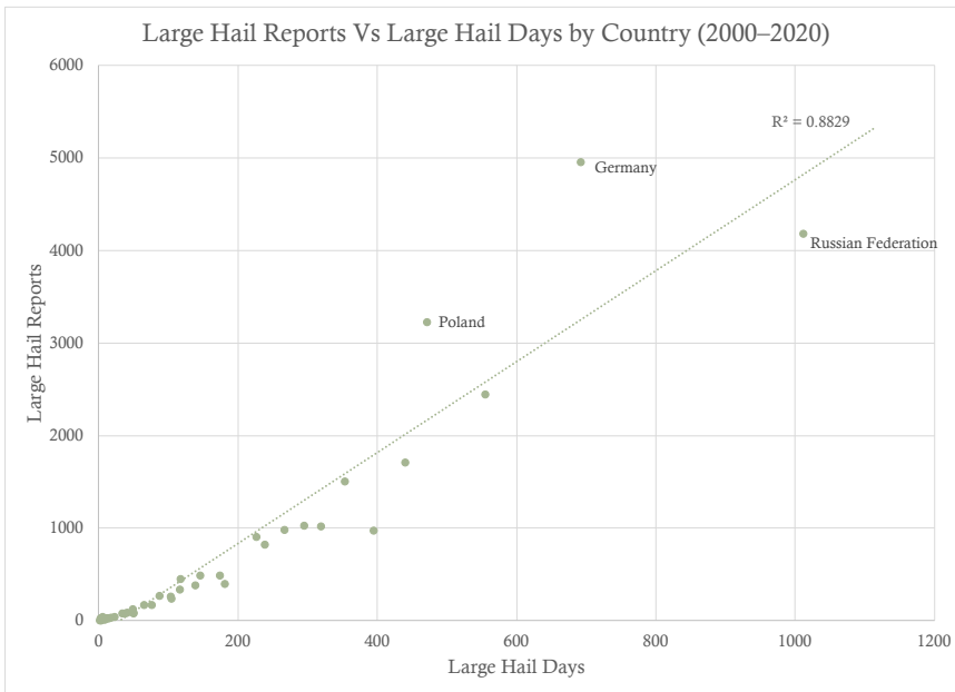
362 363 Figure 13. Scatterplot of the total number of large-hail reports versus large-hail days by country: 2000– 364 2020.
