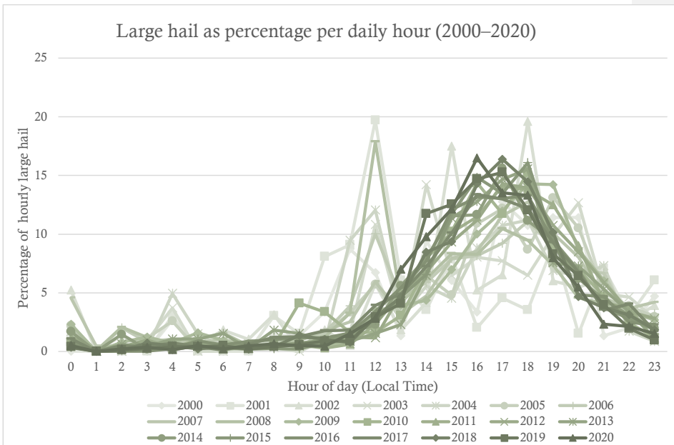
255 Figure 6. Hourly percentage of large hail in local time across Europe in local time for each year 2000 to 256 2020.
