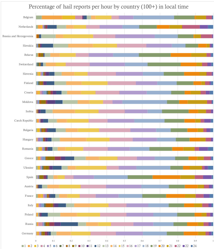
264 Figure 7. Horizontal bar charts of the hourly distributions of large-hail reports (percentage divided by 265 100) for countries with 100 or more reports: 2000–2020.
