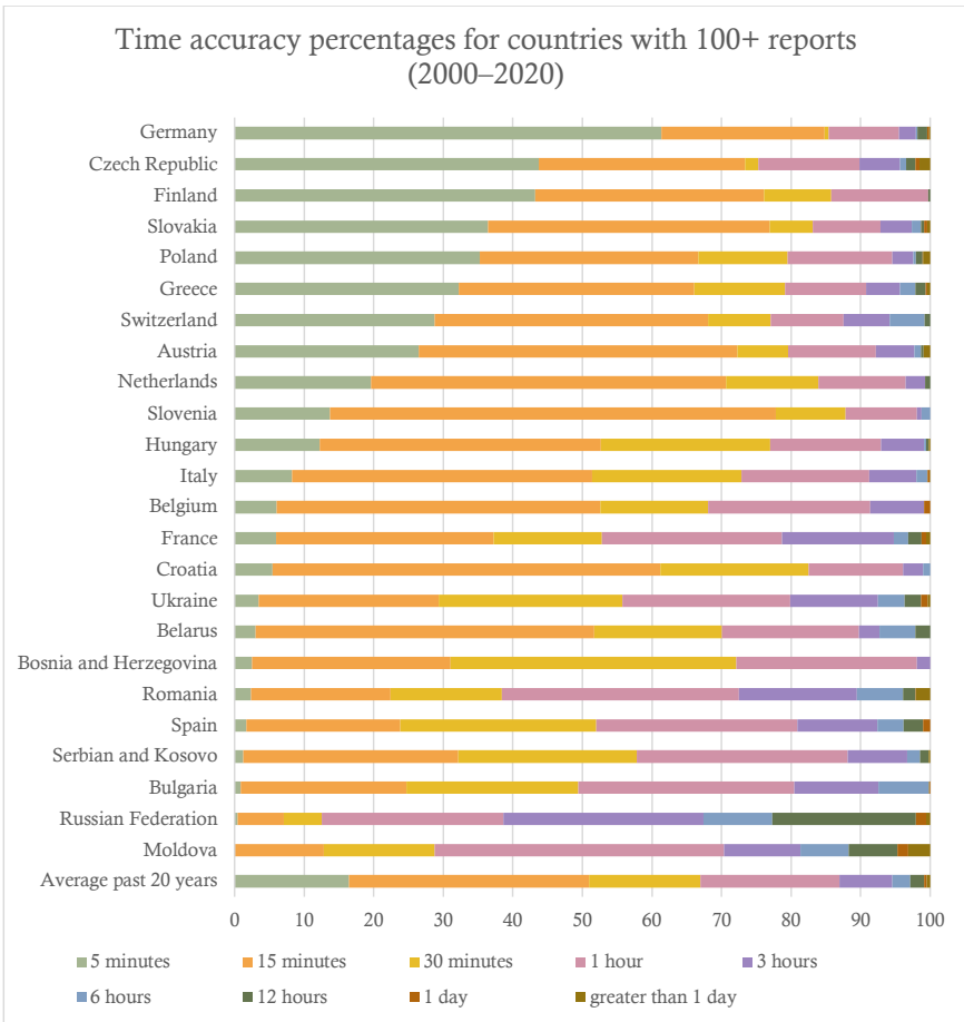
330 331 Figure 12. Horizontal bar charts of the time accuracy for countries with 100 or more reports (%): 2000– 332 2020.
