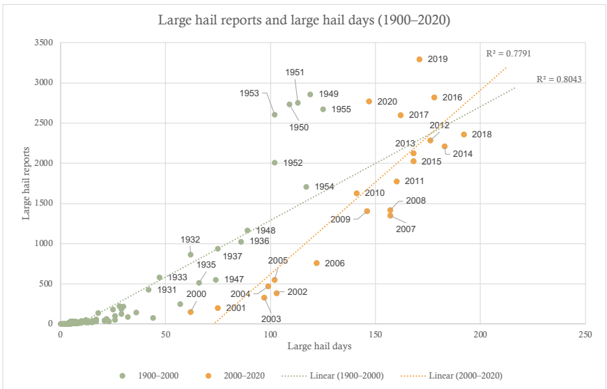
189 190 Figure 2. Scatterplot of the annual number of large-hail days versus annual number of large-hail reports 191 across Europe: 1900–2000 (green dots) and 2000–2020 (orange dots), with corresponding linear regression 192 lines. These quantities are not divided by the number of years because of the incomplete data for the year 193 2020.
