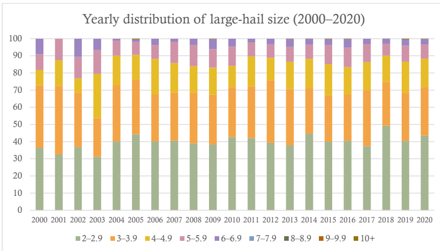
294 Figure 9. Time series of bar charts of the annual distributions of large-hail size across Europe in 1-cm 295 diameter bins (%): 2000–2020. 296
