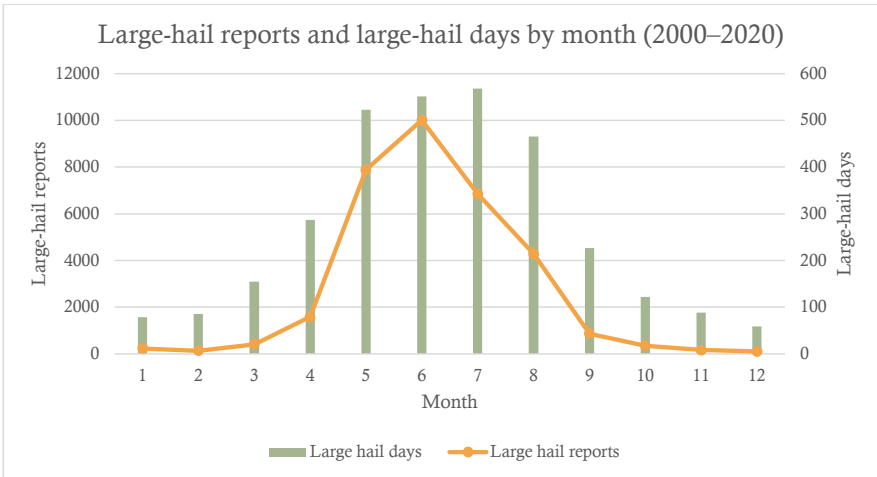
209 210 Figure 3. Combined line graph and bar chart of the total monthly numbers of large-hail reports (orange 211 line) and large-hail days (green bars) across Europe: 2000–2020. These quantities are not divided by the 212 number of years because of the incomplete data for the year 2020.
