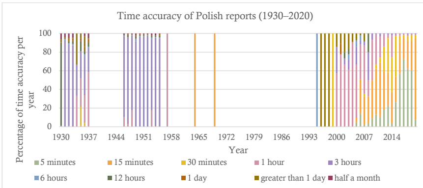
497 498 Figure 17. Time series of bar charts the annual distributions of time accuracy of reports for Poland (%): 499 1930–2020.
