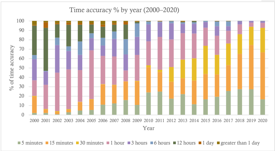
321 Figure 11. Time series of bar charts of the annual distributions of time accuracy of reports across Europe 322 (%): 2000–2020. 323
