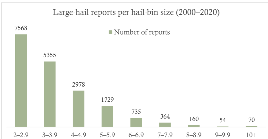
283 Figure 8. Bar chart of the number of large-hail reports across Europe by maximum diameter in 1-cm bins: 284 2000–2020.
