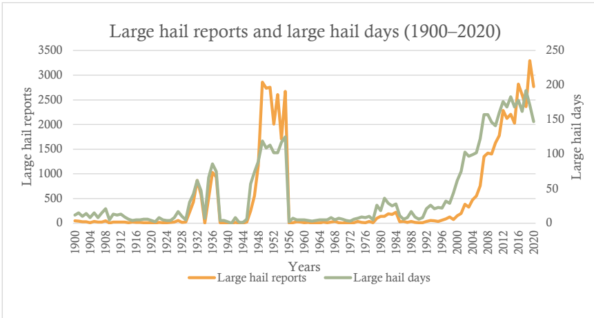
173 174 Figure 1. Time series of annual numbers of large-hail reports (orange line) and large-hail days (green 175 line) across Europe 1900–2020.
