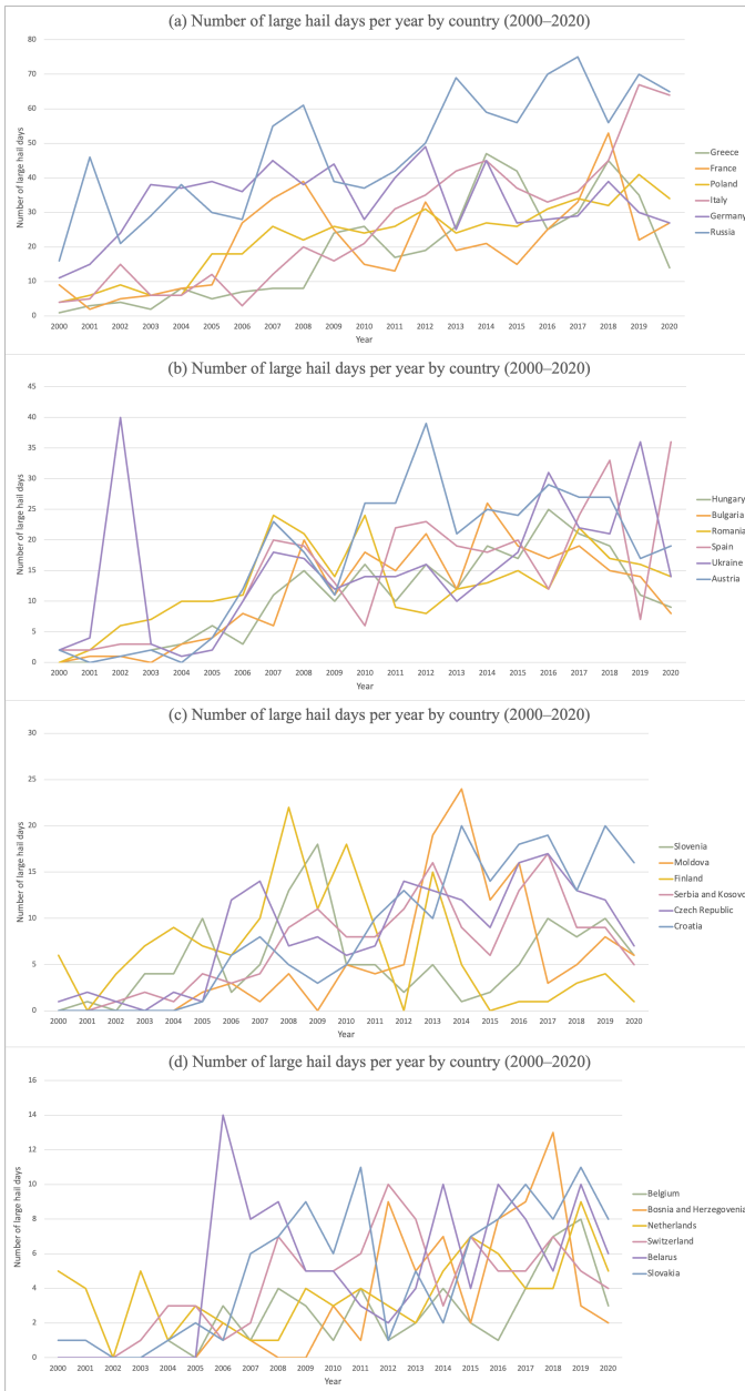
412 Figure 14. Line graph of large hail days per country for countries with 100+ reports: 2000–2020. (a) top 6
