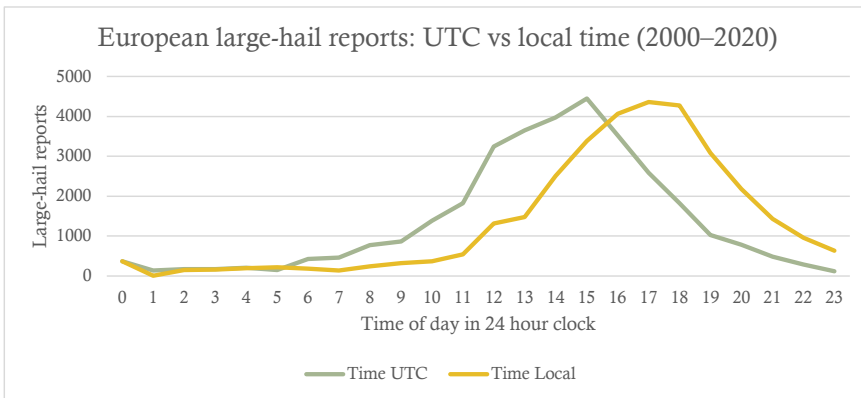
240 241 Figure 5. Distribution of the hourly time of large-hail reports across Europe in UTC (green line) and local 242 time (orange line): 2000–2020. Reports are associated with the starting hour (i.e., a report at 1515 UTC 243 would be placed in the 1500-UTC bin).
